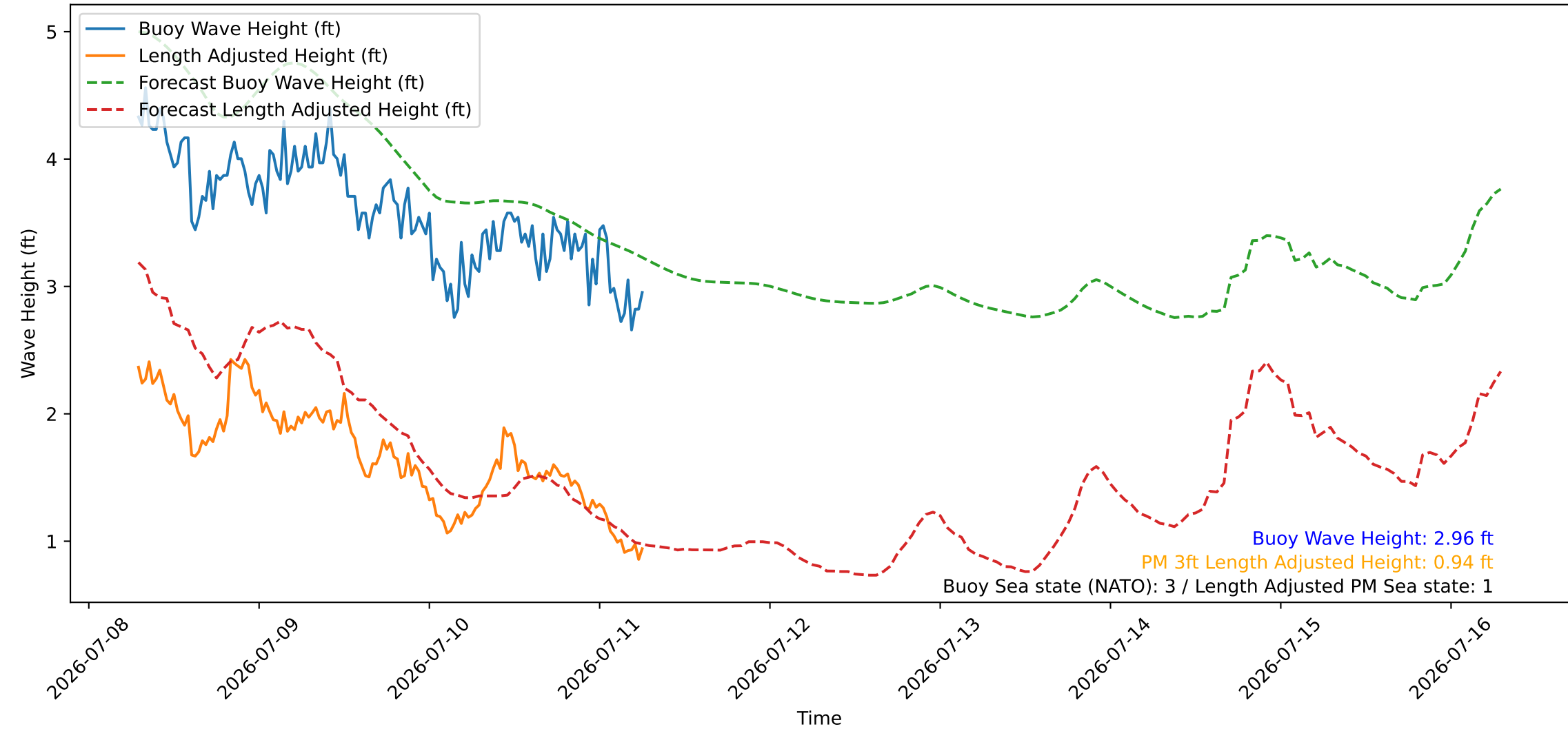
Wave Heights over Time for Green Beach at 2026-07-11 06:51:09
