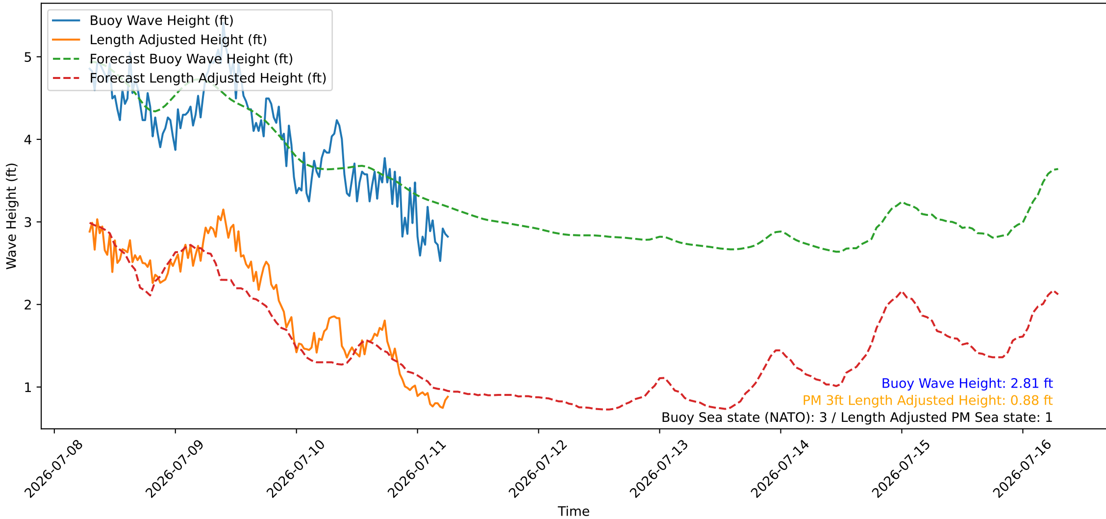
Wave Heights over Time for Oceanside Harbor at 2026-07-11 06:50:26
