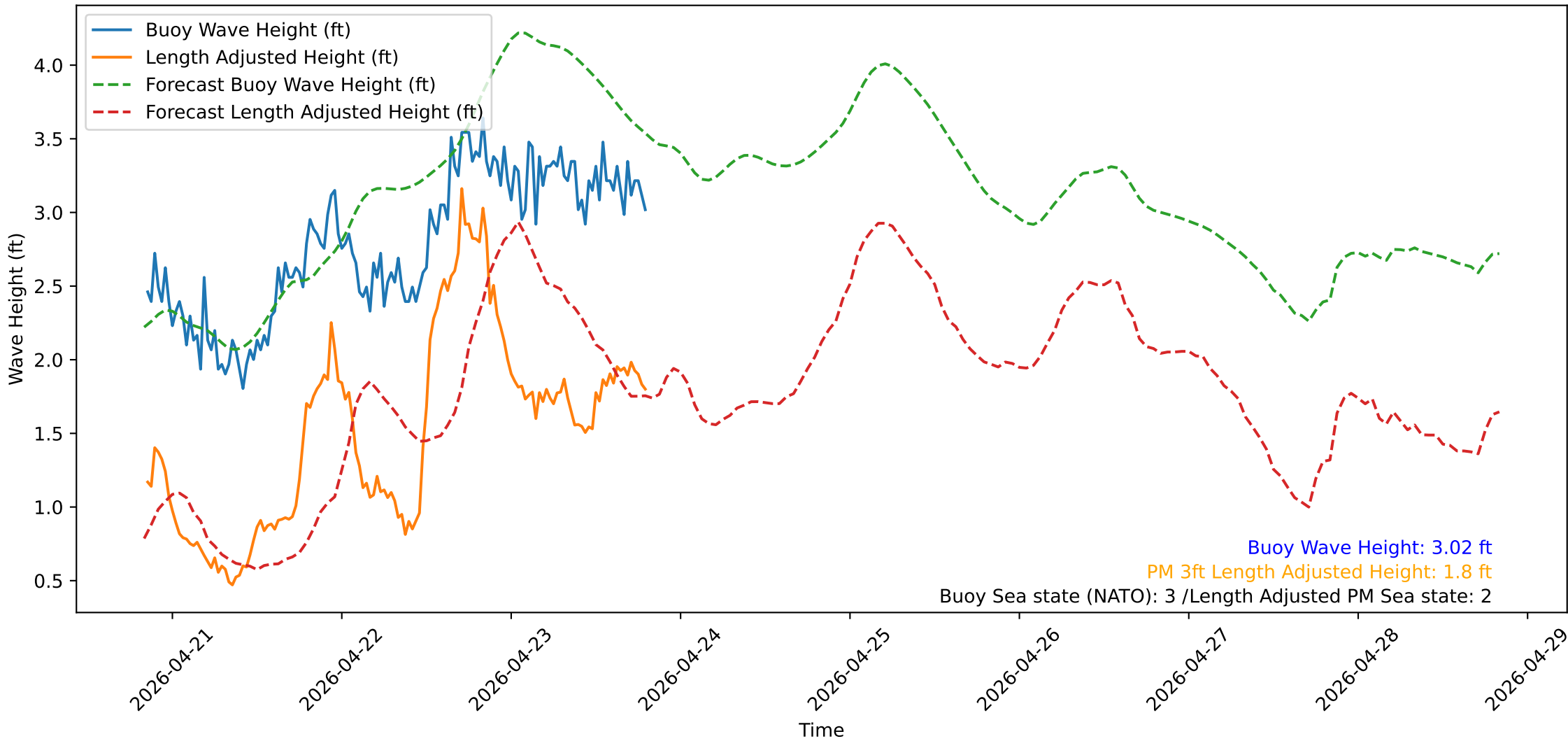
Wave Heights over Time for Red Beach at 2026-04-23 20:00:50
