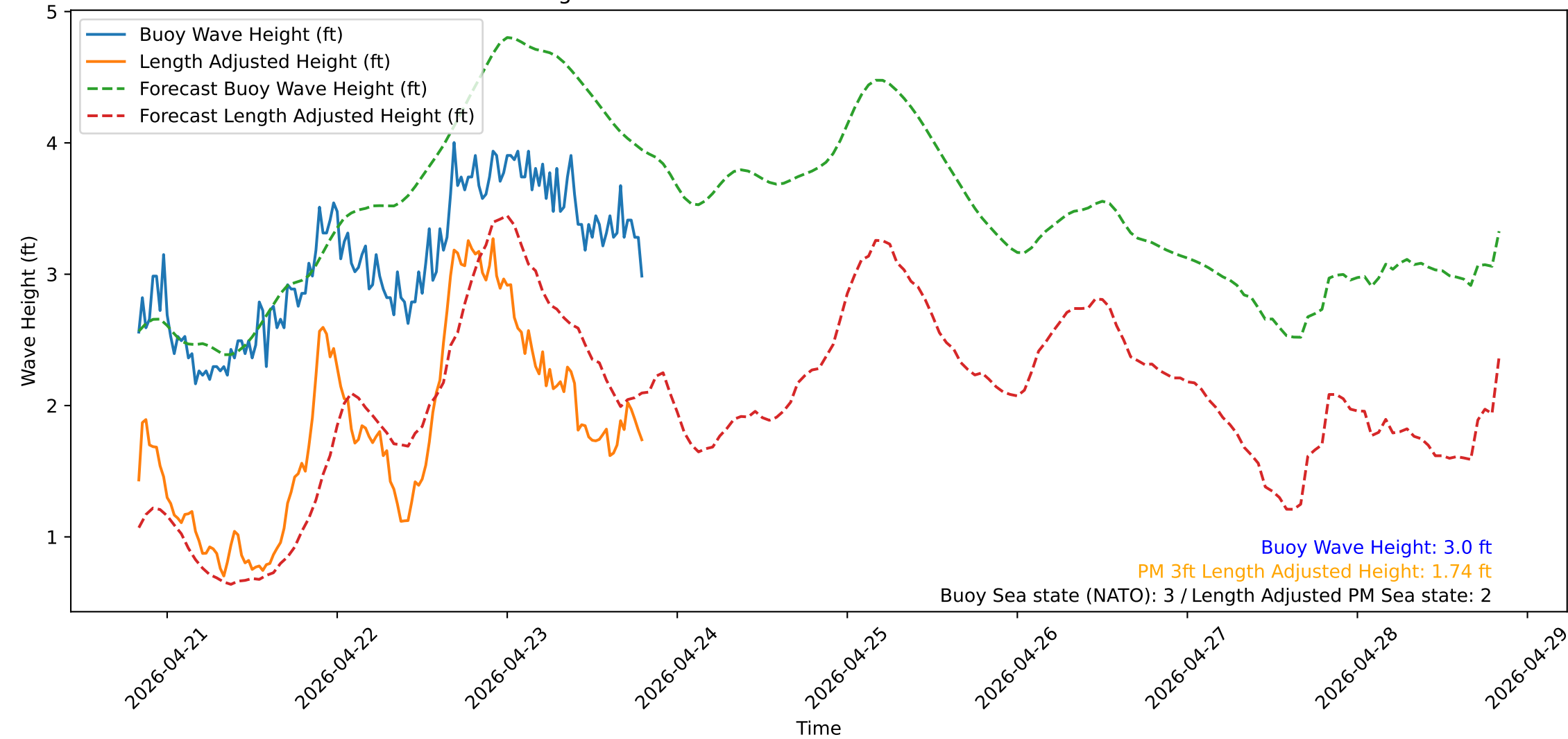
Wave Heights over Time for Green Beach at 2026-04-23 20:01:13
