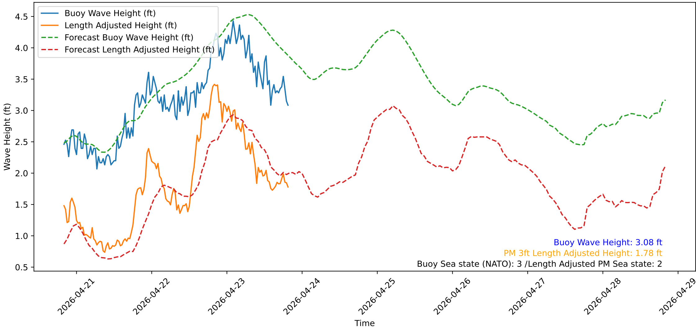
Wave Heights over Time for Oceanside Harbor at 2026-04-23 20:00:31
