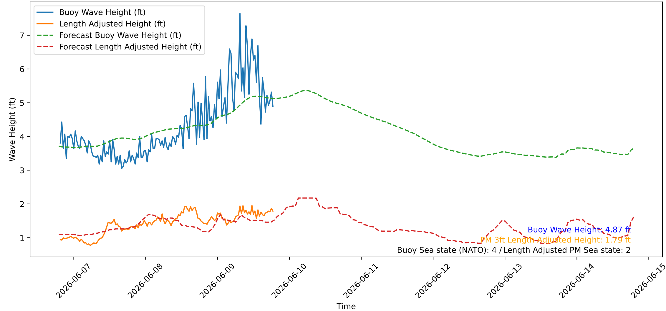
Wave Heights over Time for Red Beach at 2026-06-09 19:10:47
