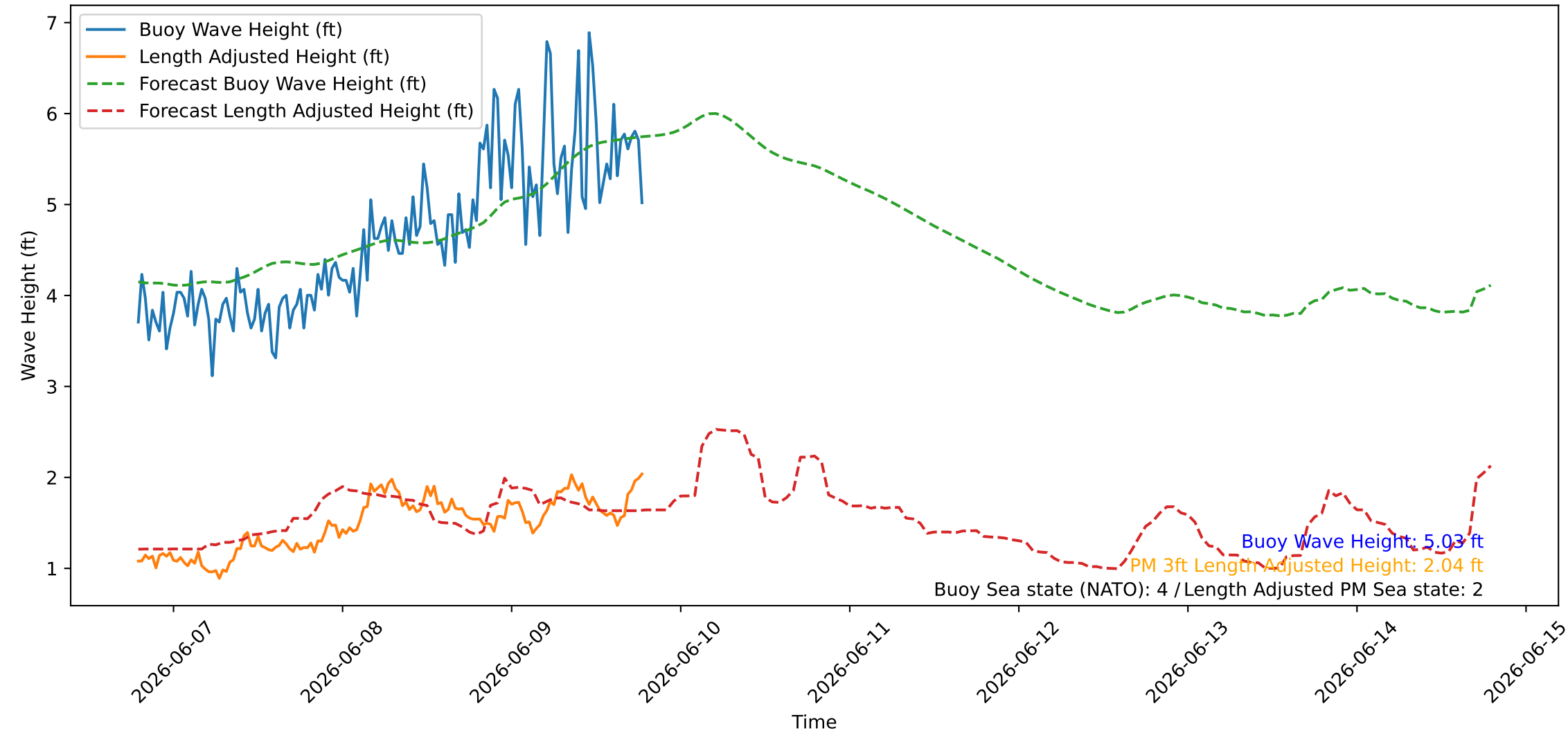
Wave Heights over Time for Green Beach at 2026-06-09 19:11:10
