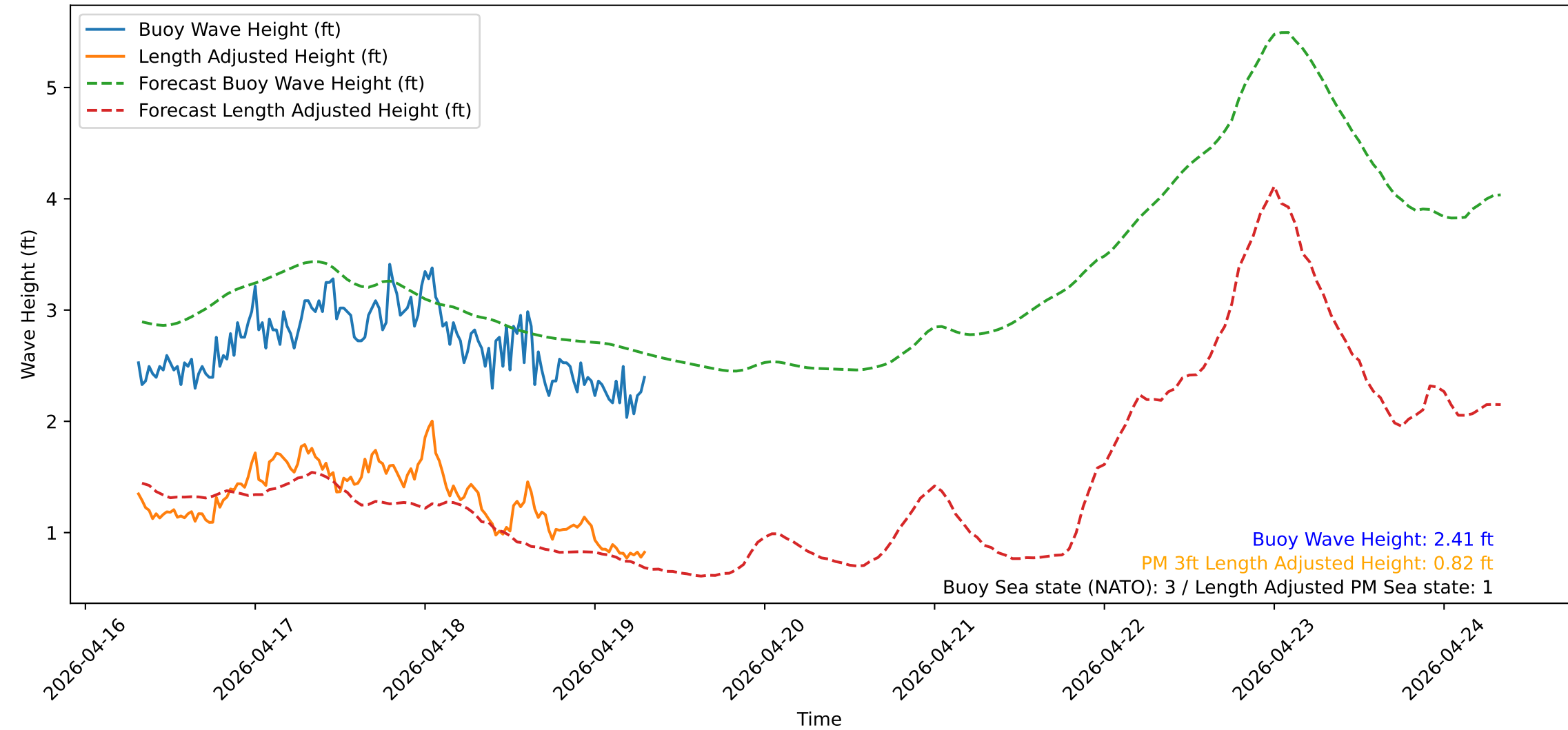
Wave Heights over Time for Oceanside Harbor at 2026-04-19 07:40:31
