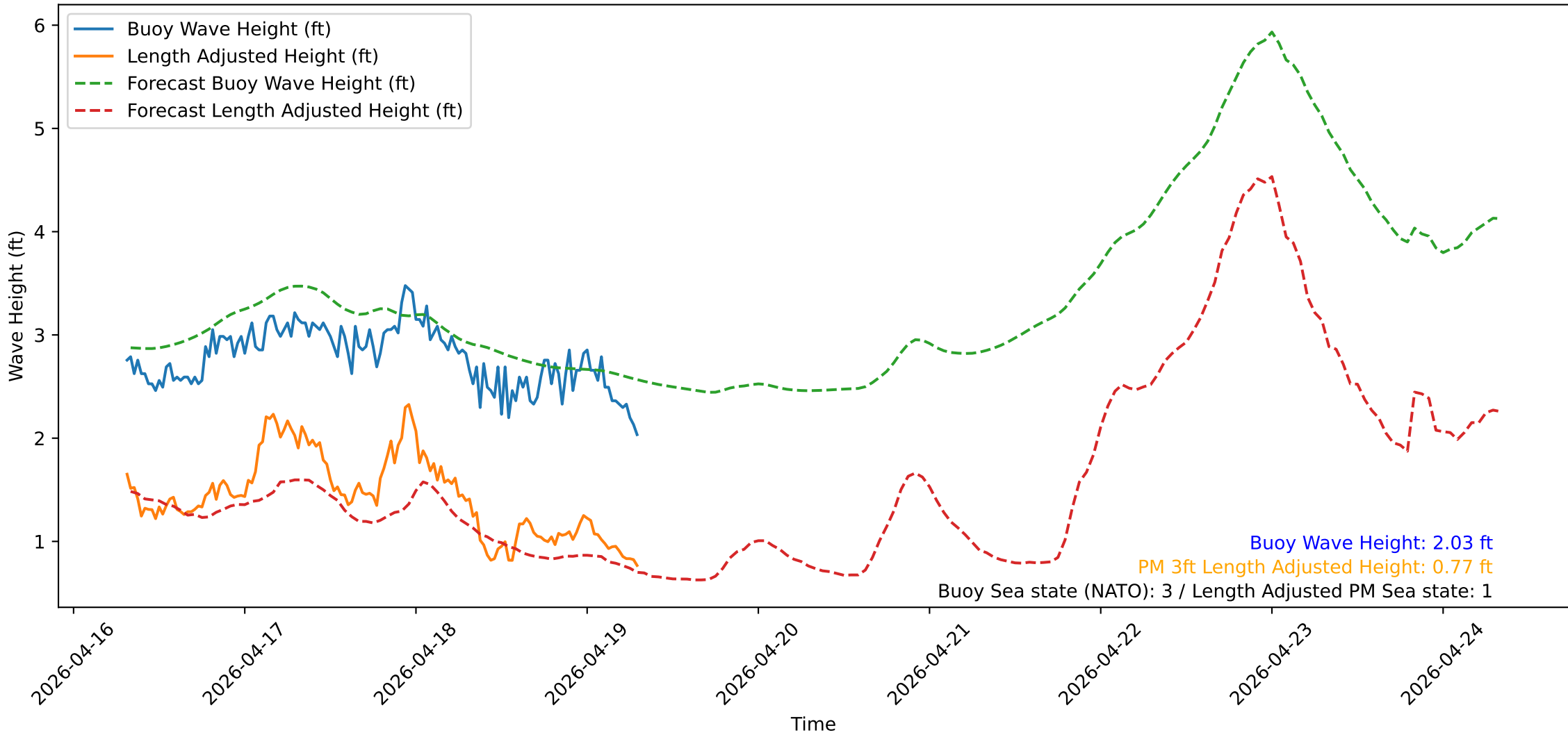
Wave Heights over Time for Green Beach at 2026-04-19 07:41:13
