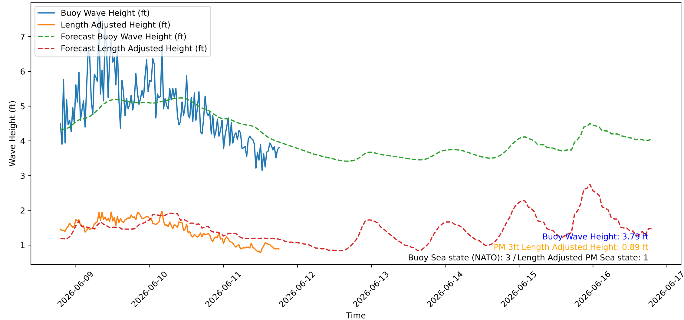
Wave Heights over Time for Red Beach at 2026-06-11 18:50:48
