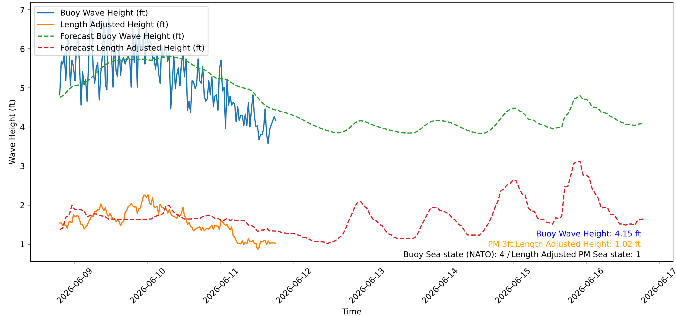
Wave Heights over Time for Green Beach at 2026-06-11 18:51:11
