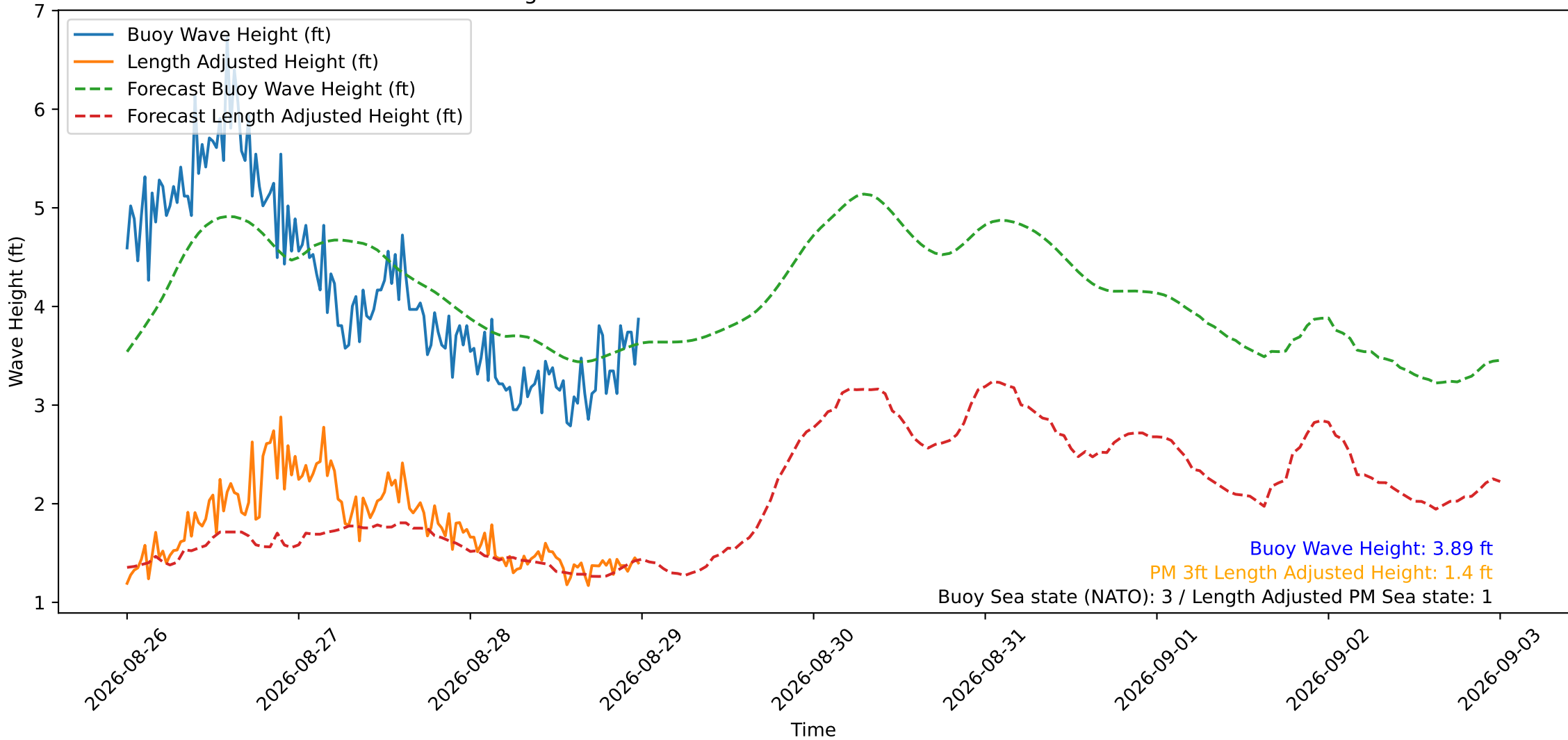
Wave Heights over Time for Oceanside Harbor at 2026-08-29 00:00:30
