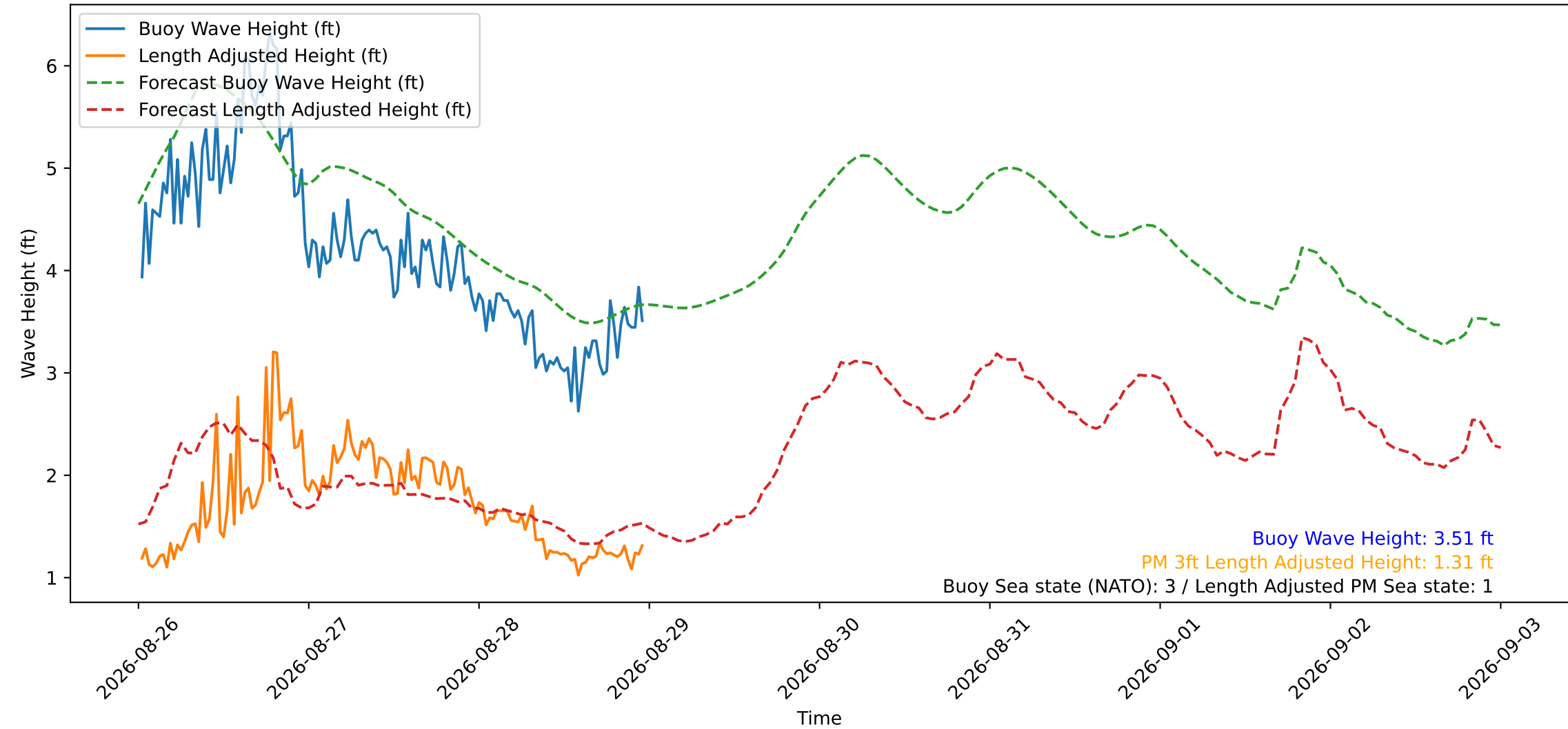
Wave Heights over Time for Green Beach at 2026-08-29 00:01:12
