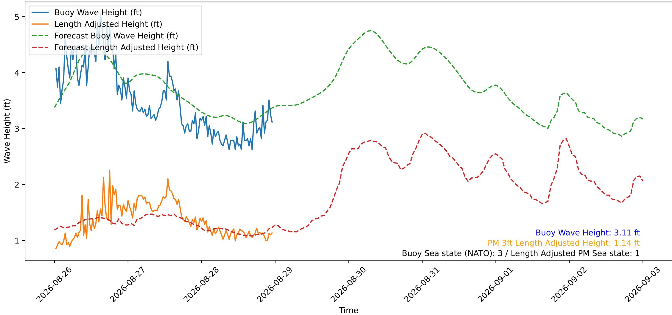
Wave Heights over Time for Red Beach at 2026-08-29 00:00:50
