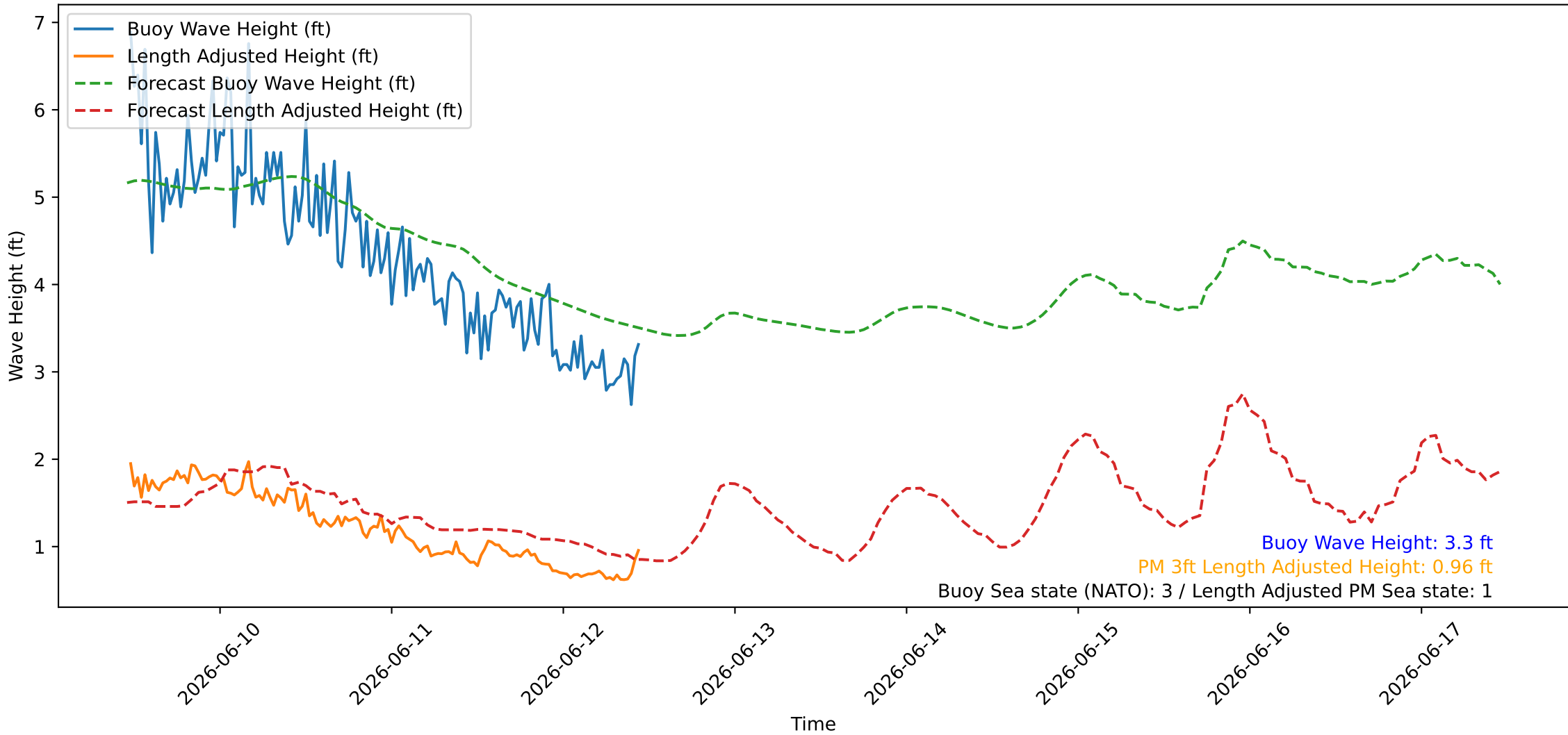
Wave Heights over Time for Red Beach at 2026-06-12 11:20:47
