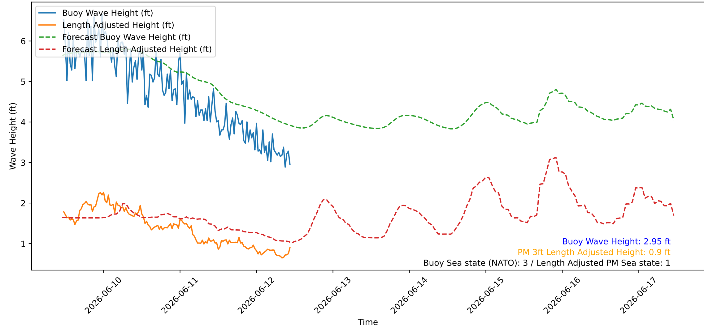
Wave Heights over Time for Green Beach at 2026-06-12 11:21:10
