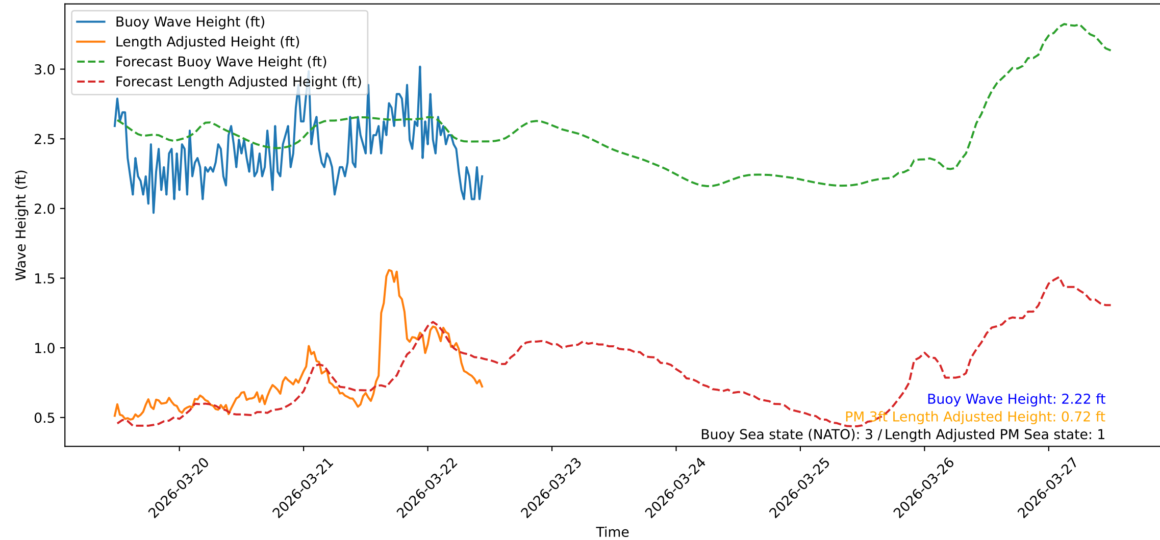
Wave Heights over Time for Oceanside Harbor at 2026-03-22 11:40:32
