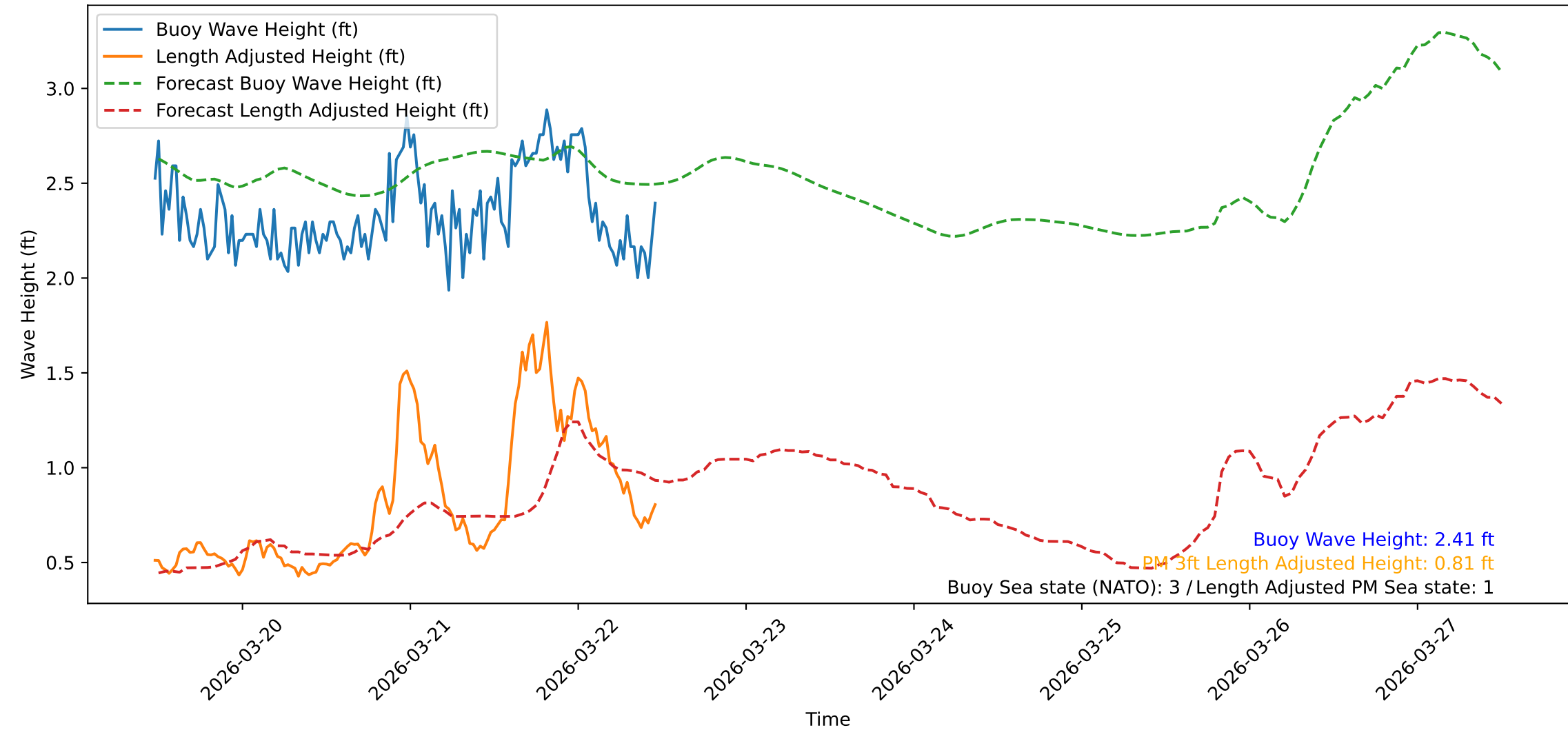
Wave Heights over Time for Green Beach at 2026-03-22 11:41:12
