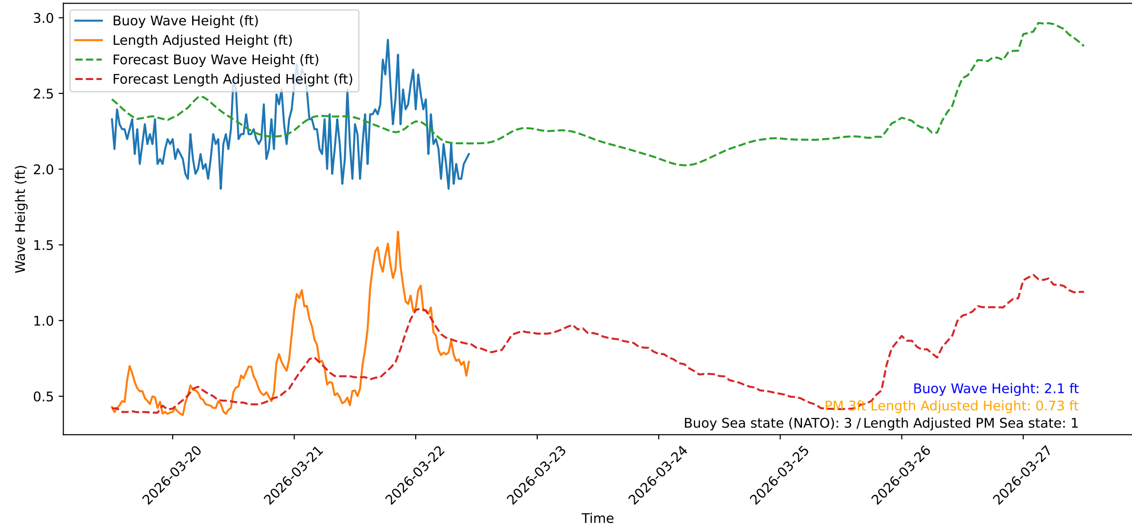
Wave Heights over Time for Red Beach at 2026-03-22 11:40:49
