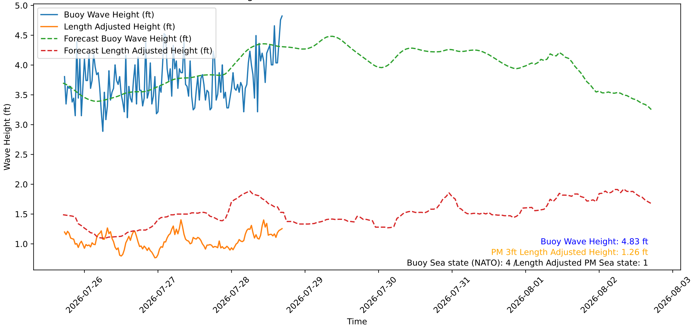
Wave Heights over Time for Red Beach at 2026-07-28 17:10:46
