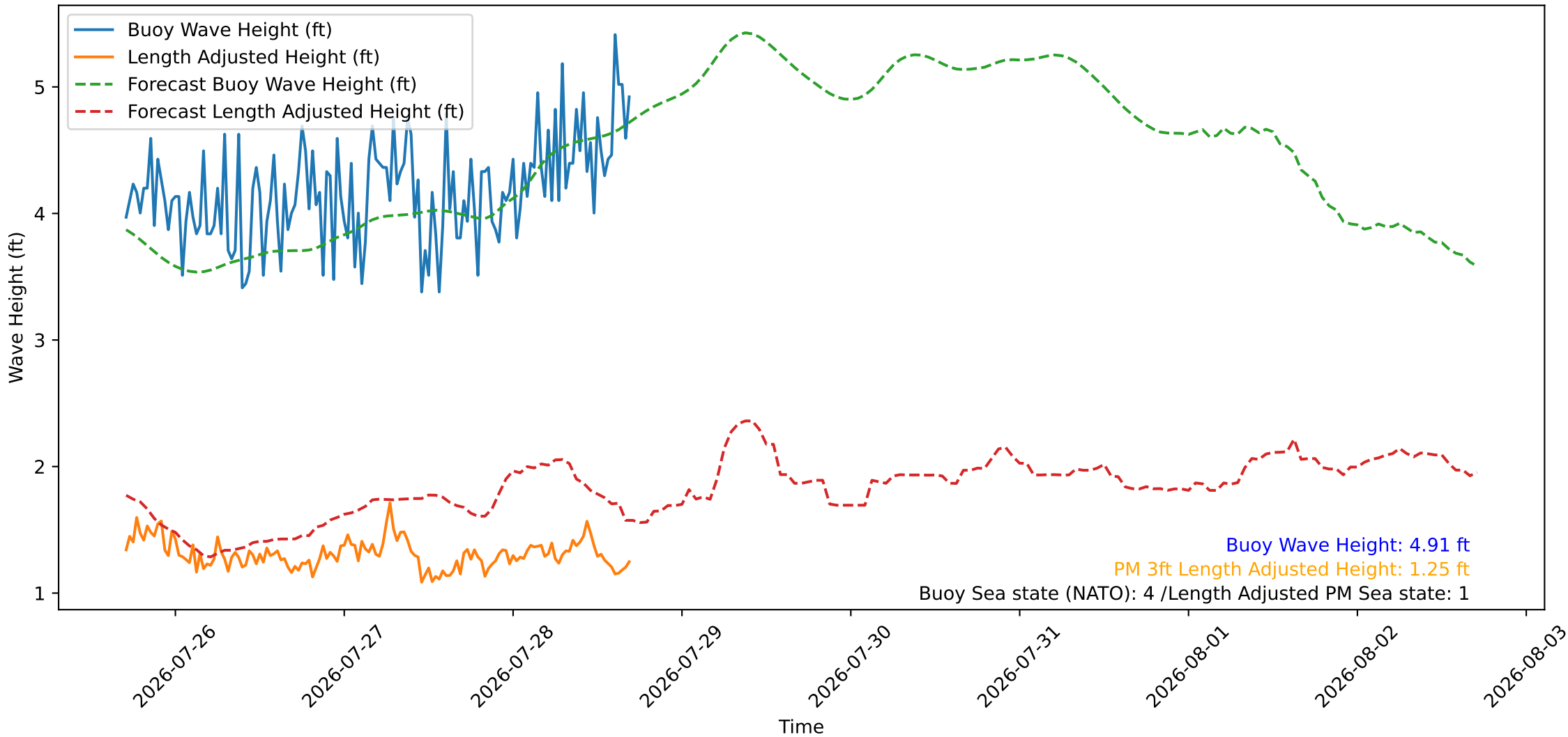
Wave Heights over Time for Green Beach at 2026-07-28 17:11:09
