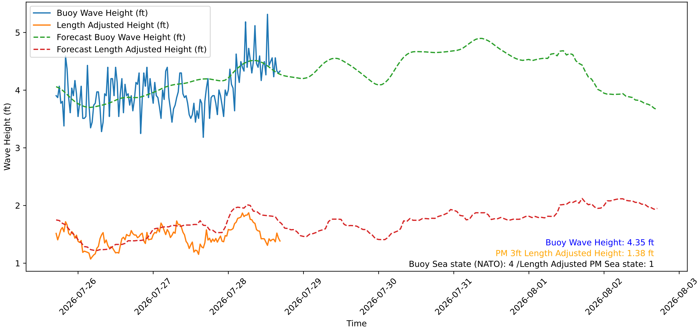
Wave Heights over Time for Oceanside Harbor at 2026-07-28 17:10:27
