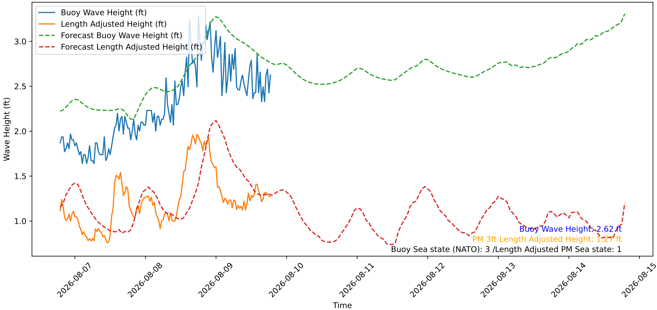
Wave Heights over Time for Oceanside Harbor at 2026-08-09 19:10:26
