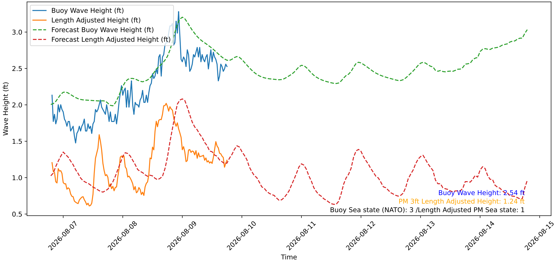
Wave Heights over Time for Red Beach at 2026-08-09 19:10:45
