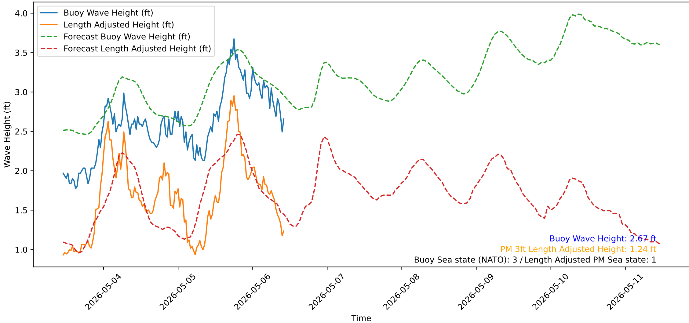
Wave Heights over Time for Green Beach at 2026-05-06 11:01:13
