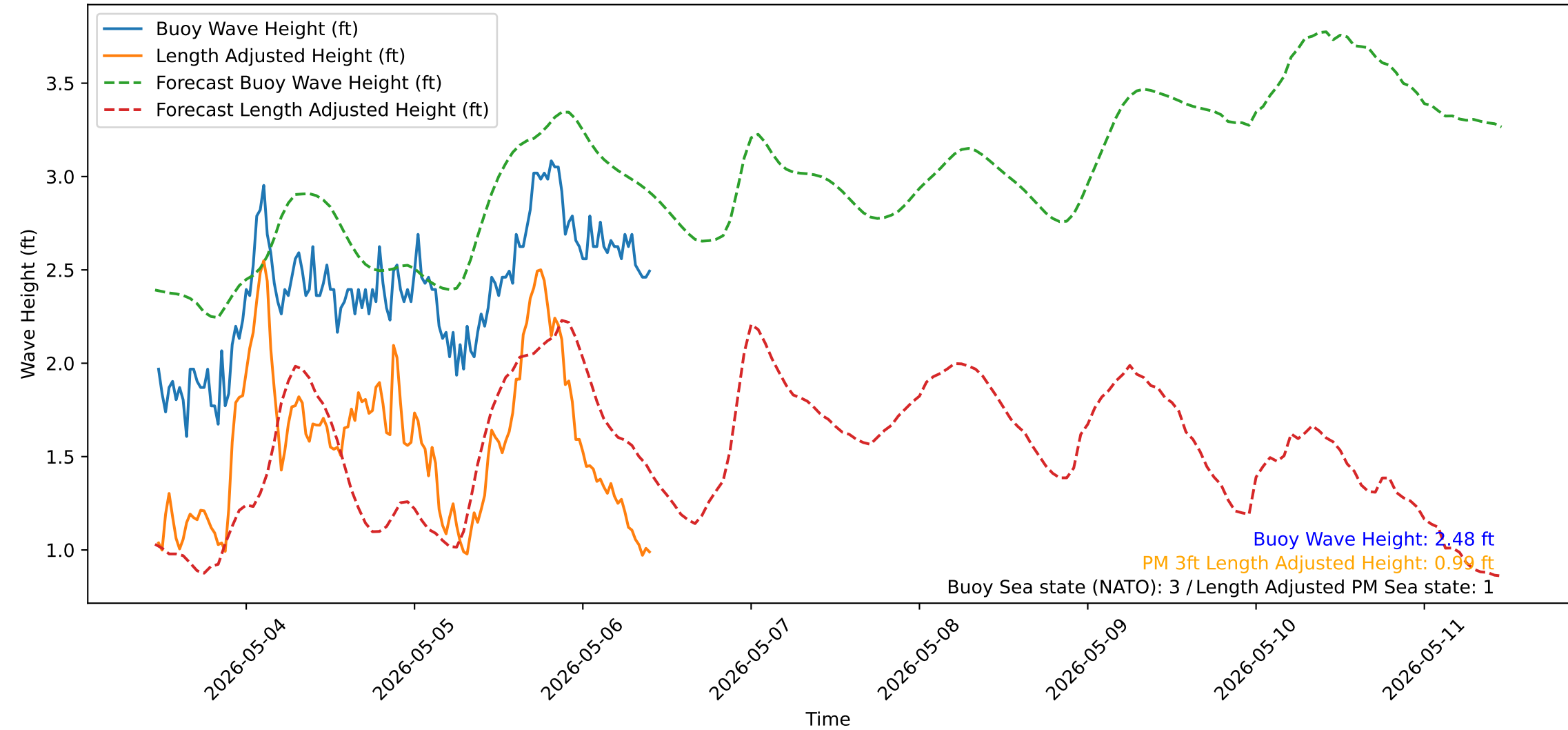
Wave Heights over Time for Red Beach at 2026-05-06 11:00:50
