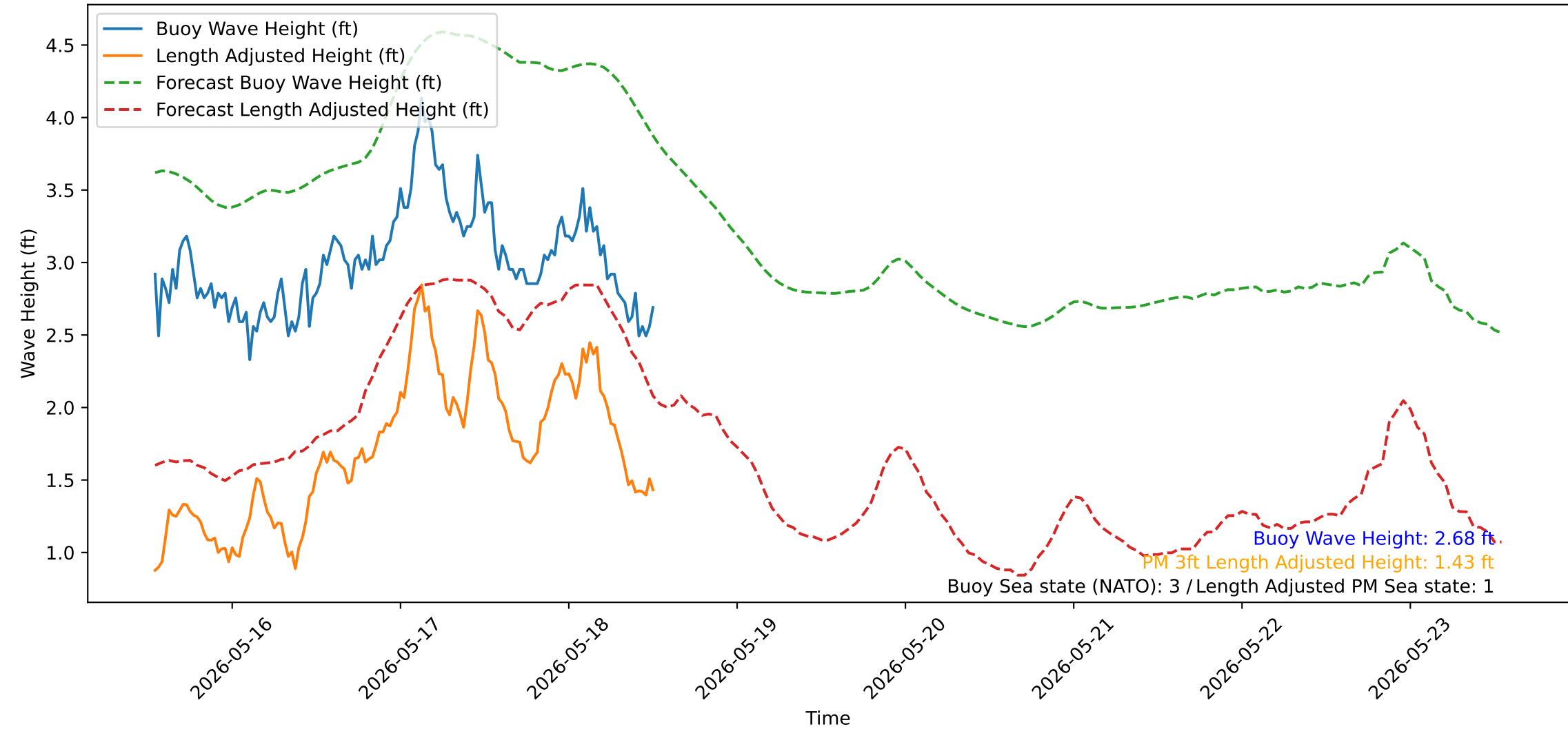
Wave Heights over Time for Red Beach at 2026-05-18 12:50:53
