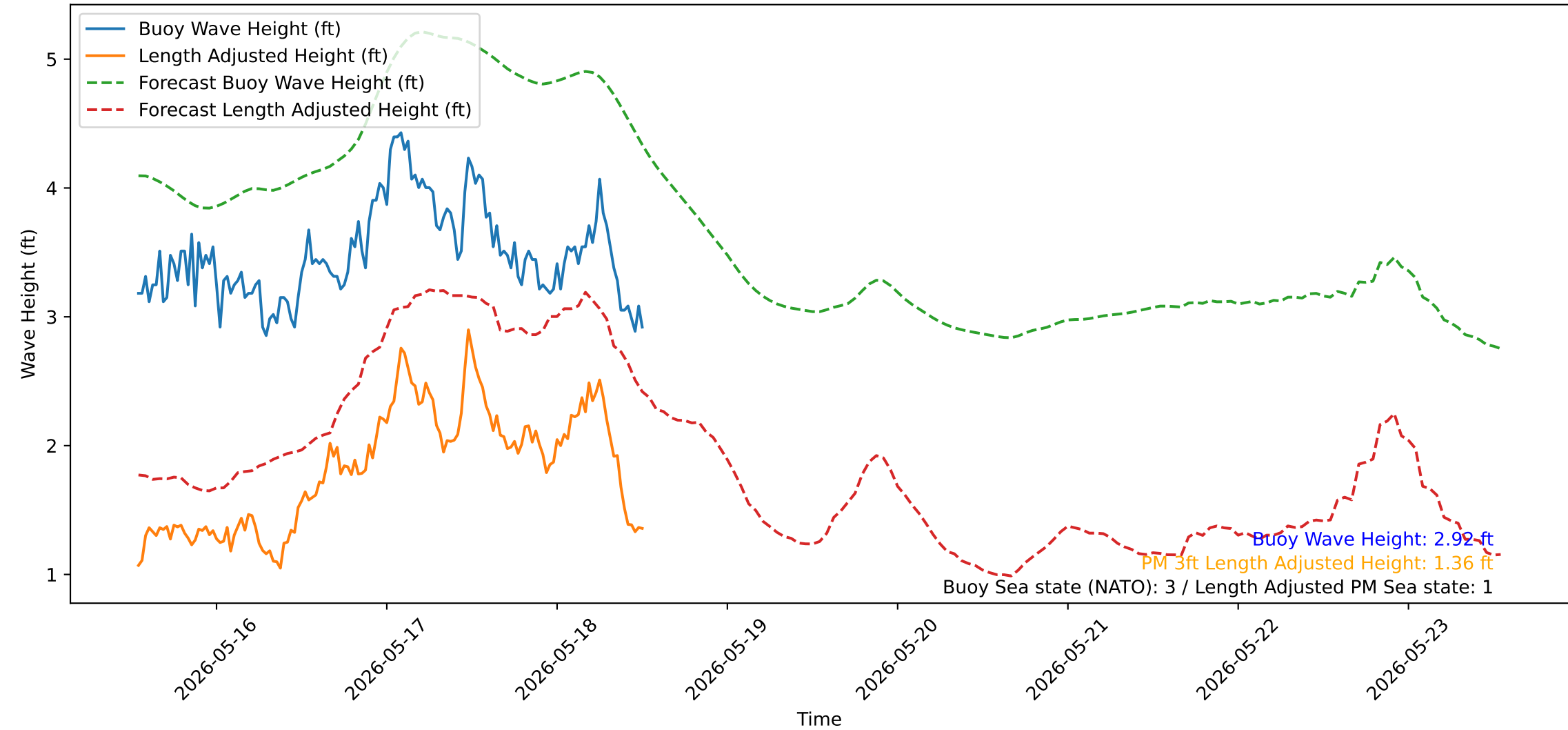
Wave Heights over Time for Green Beach at 2026-05-18 12:51:15
