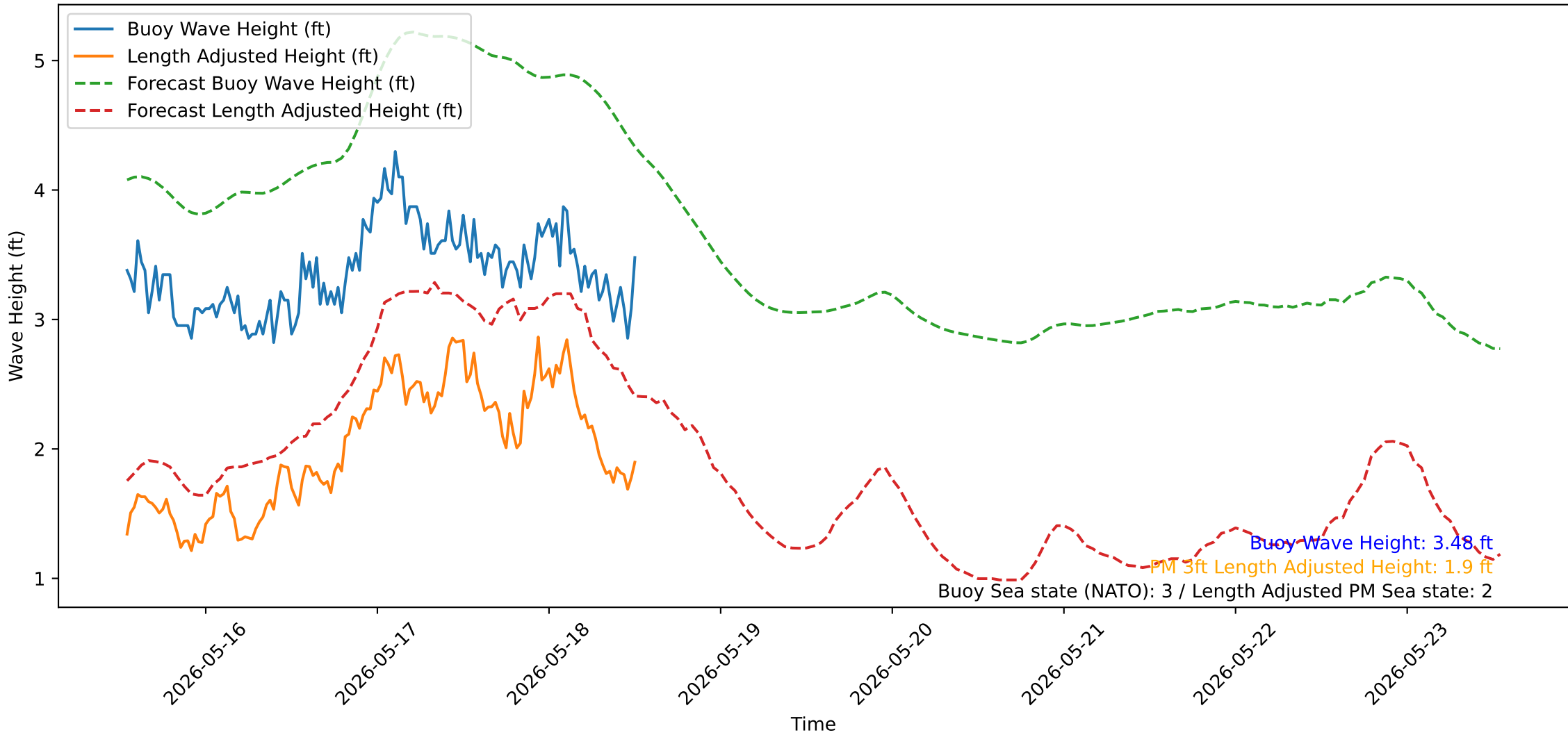
Wave Heights over Time for Oceanside Harbor at 2026-05-18 12:50:32
