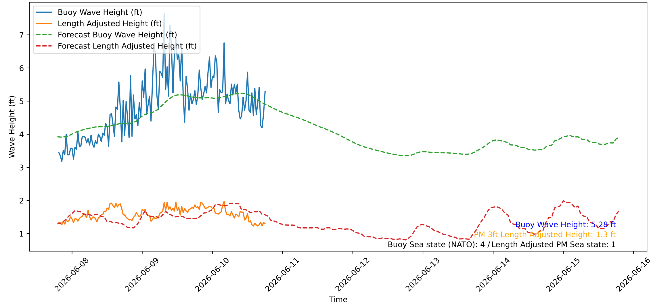
Wave Heights over Time for Red Beach at 2026-06-10 19:10:47
