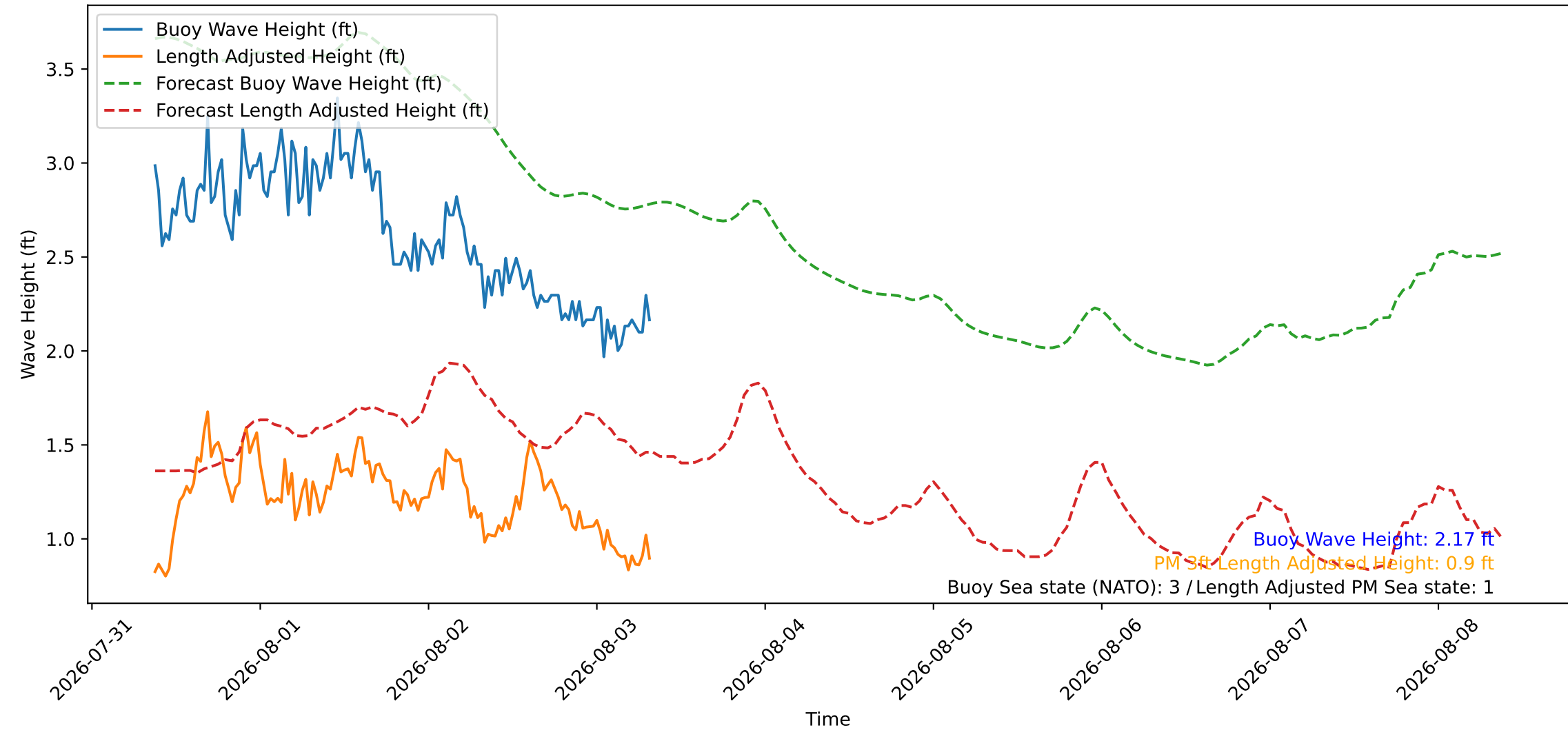
Wave Heights over Time for Red Beach at 2026-08-03 08:40:45
