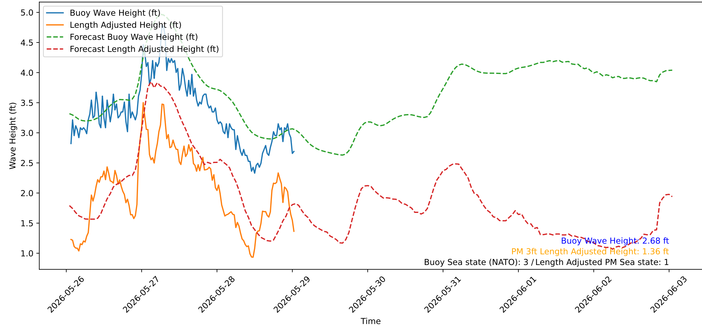
Wave Heights over Time for Red Beach at 2026-05-29 01:10:39
