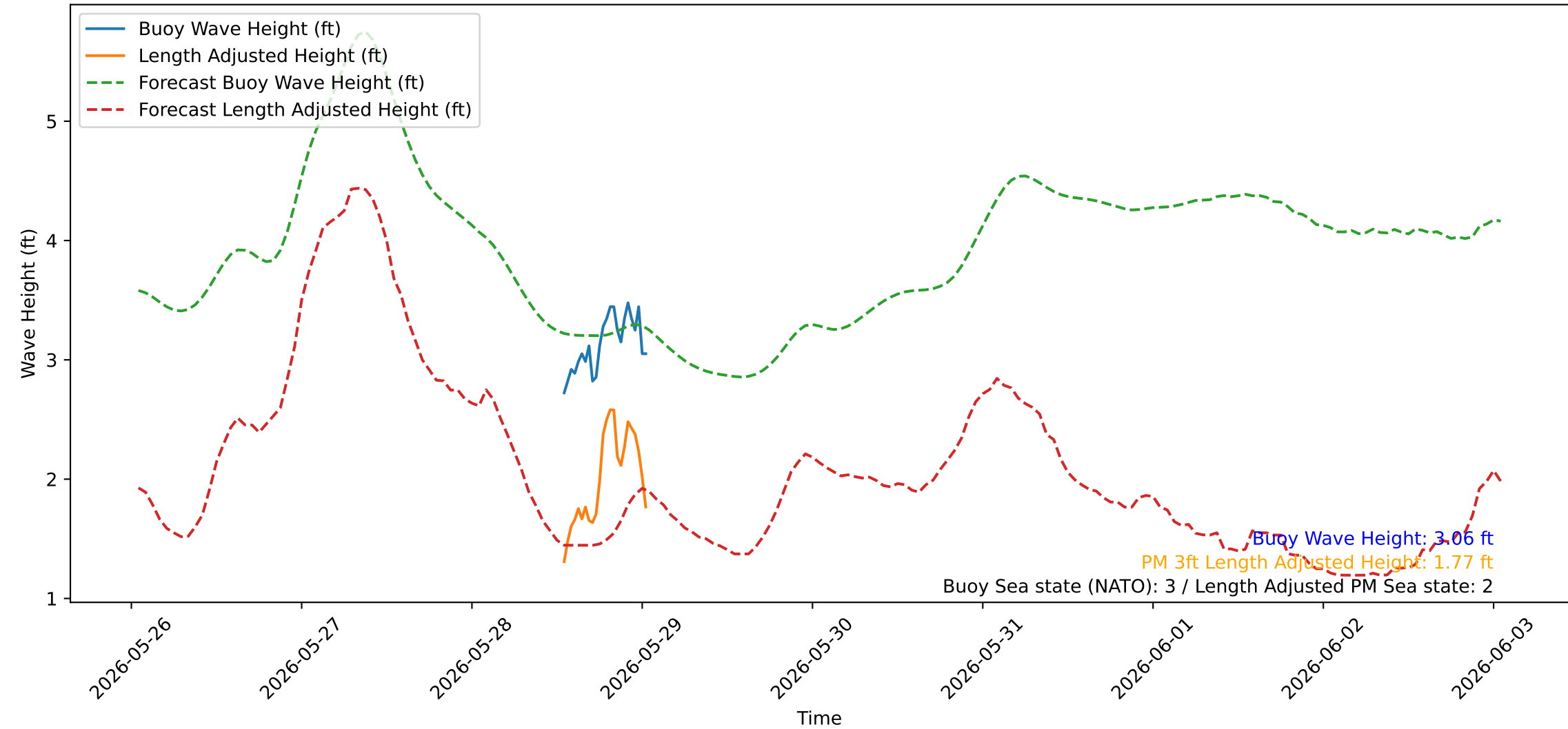
Wave Heights over Time for Oceanside Harbor at 2026-05-29 01:10:20
