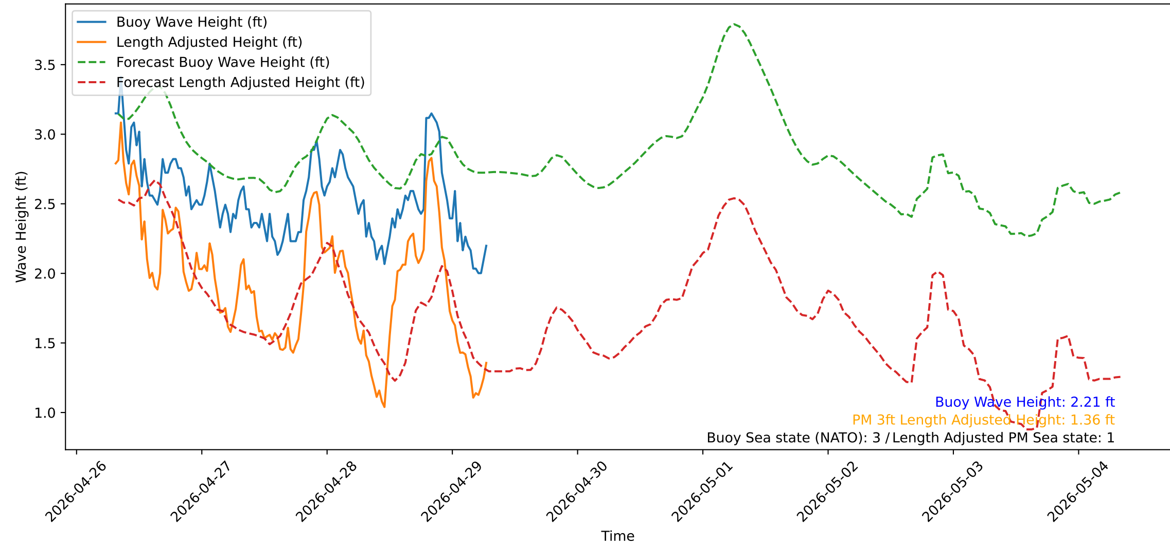
Wave Heights over Time for Green Beach at 2026-04-29 07:31:13
