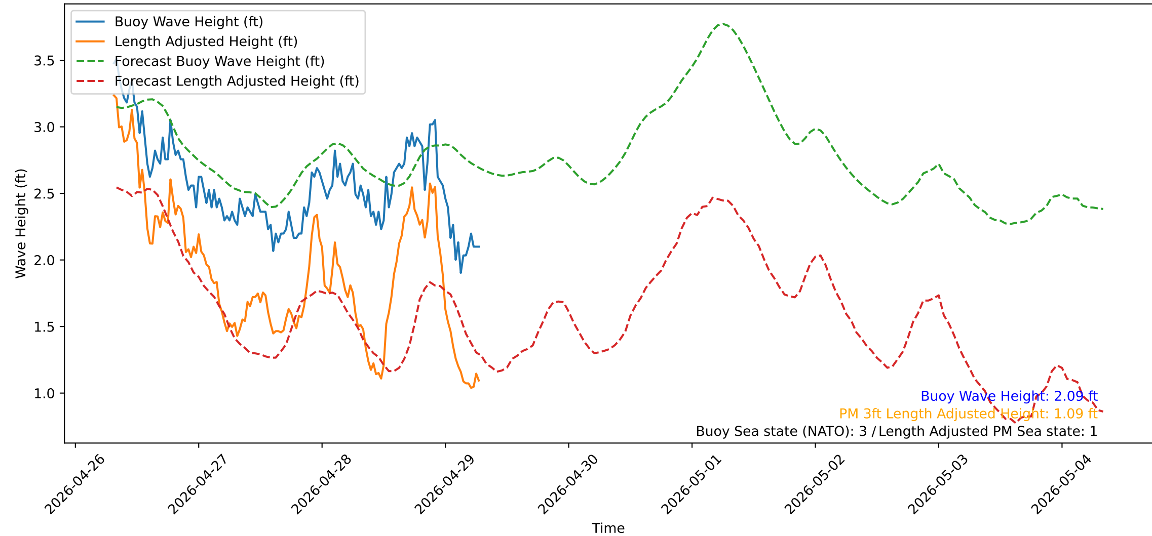
Wave Heights over Time for Oceanside Harbor at 2026-04-29 07:30:32
