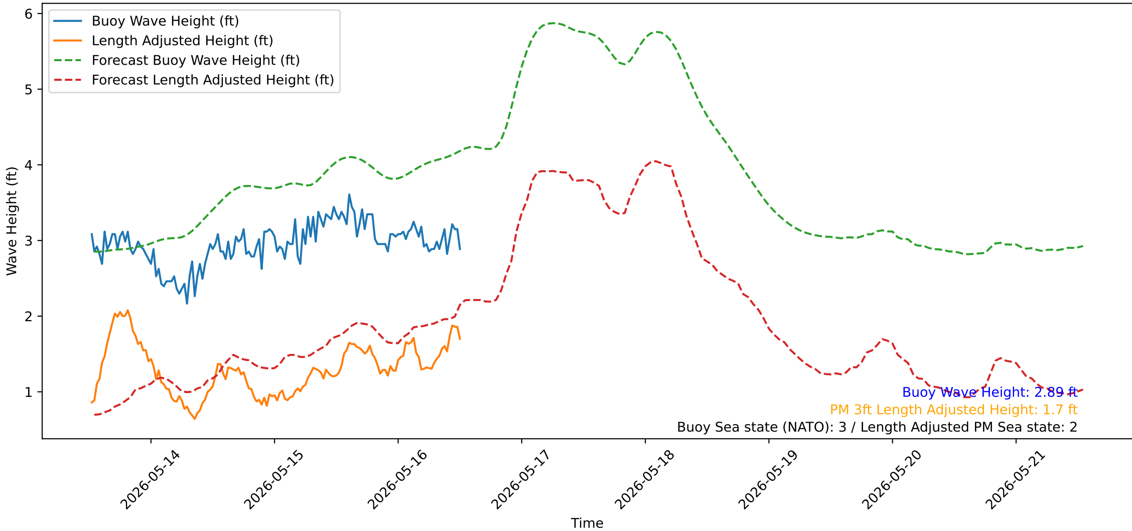
Wave Heights over Time for Oceanside Harbor at 2026-05-16 12:40:32
