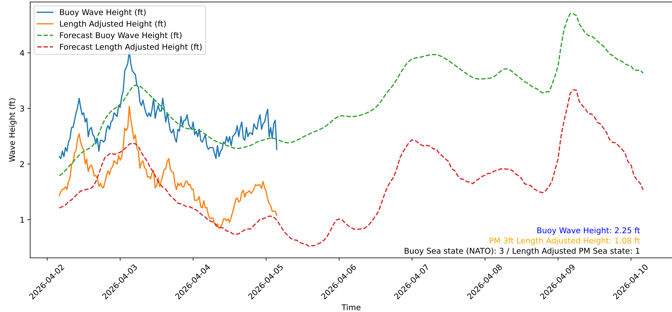
Wave Heights over Time for Oceanside Harbor at 2026-04-05 04:00:31
