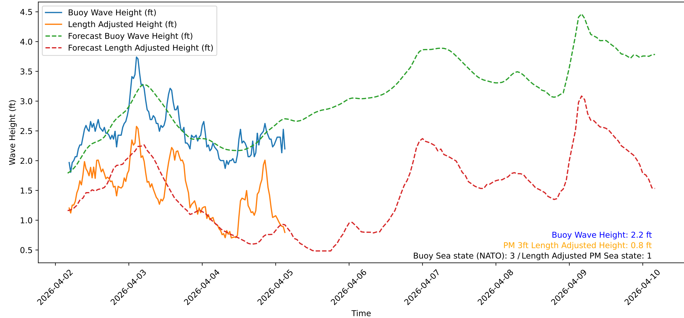
Wave Heights over Time for Red Beach at 2026-04-05 04:00:47
