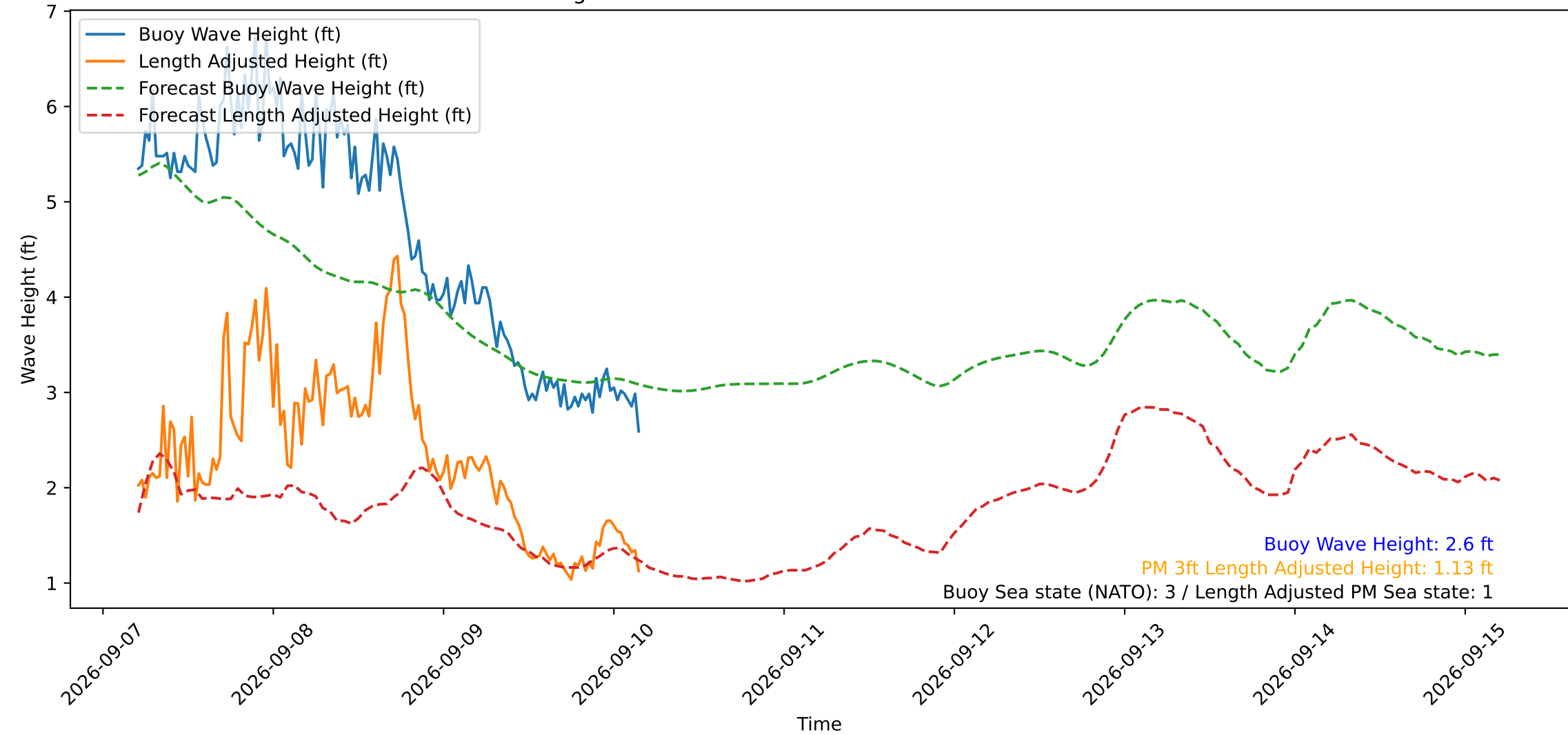
Wave Heights over Time for Red Beach at 2026-09-10 04:30:49
