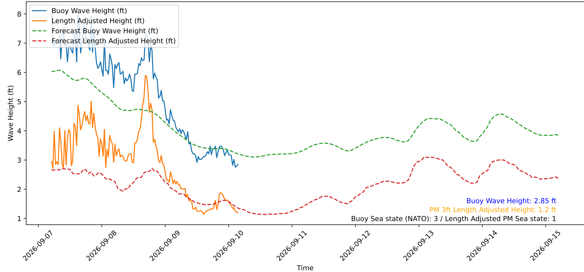
Wave Heights over Time for Green Beach at 2026-09-10 04:31:11
