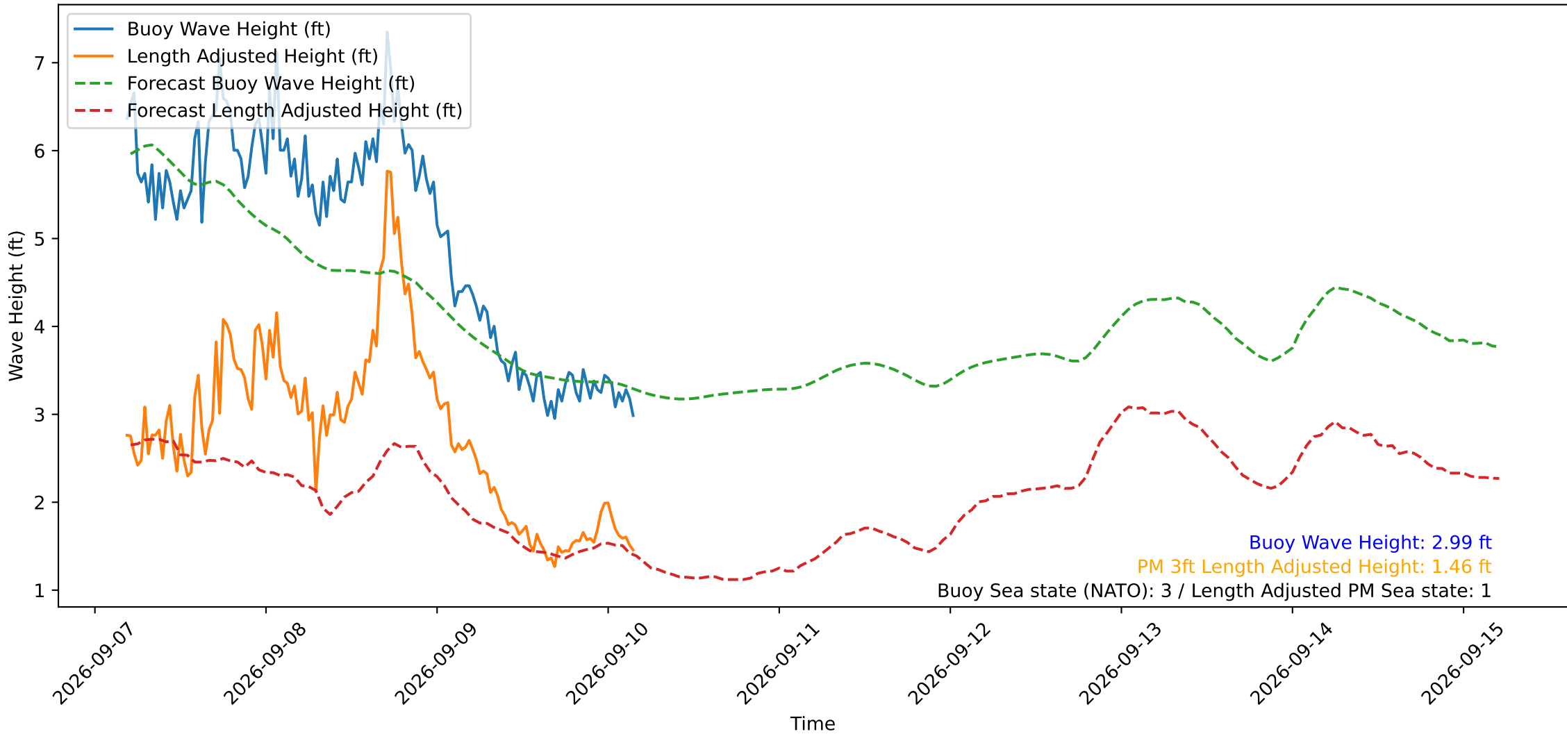
Wave Heights over Time for Oceanside Harbor at 2026-09-10 04:30:29
