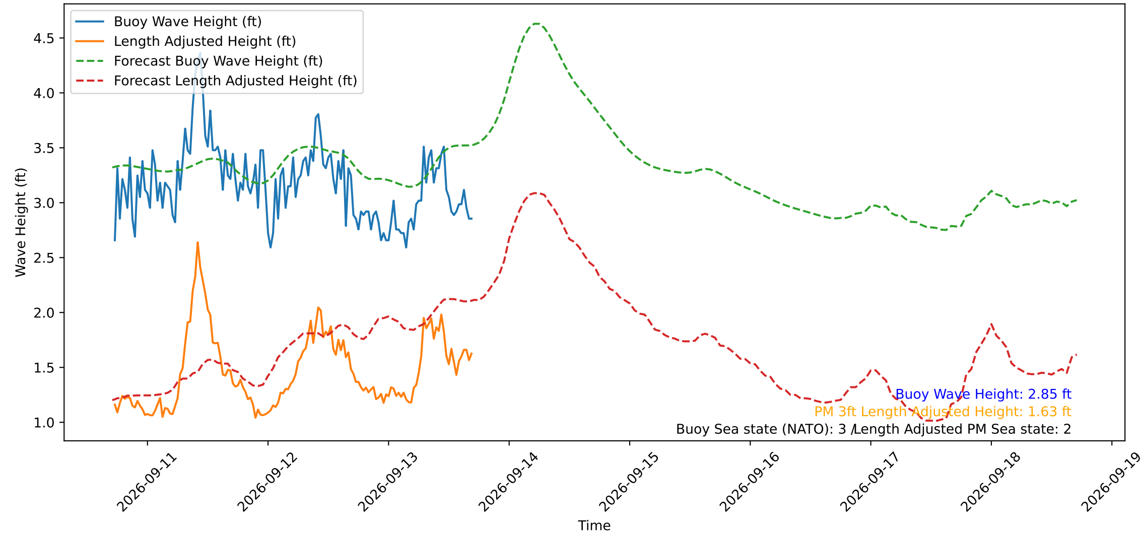
Wave Heights over Time for Oceanside Harbor at 2026-09-13 17:20:30
