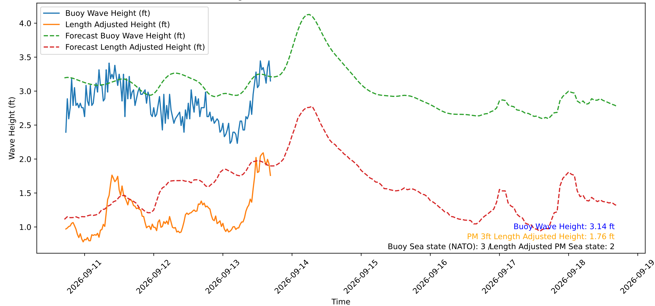
Wave Heights over Time for Red Beach at 2026-09-13 17:20:50
