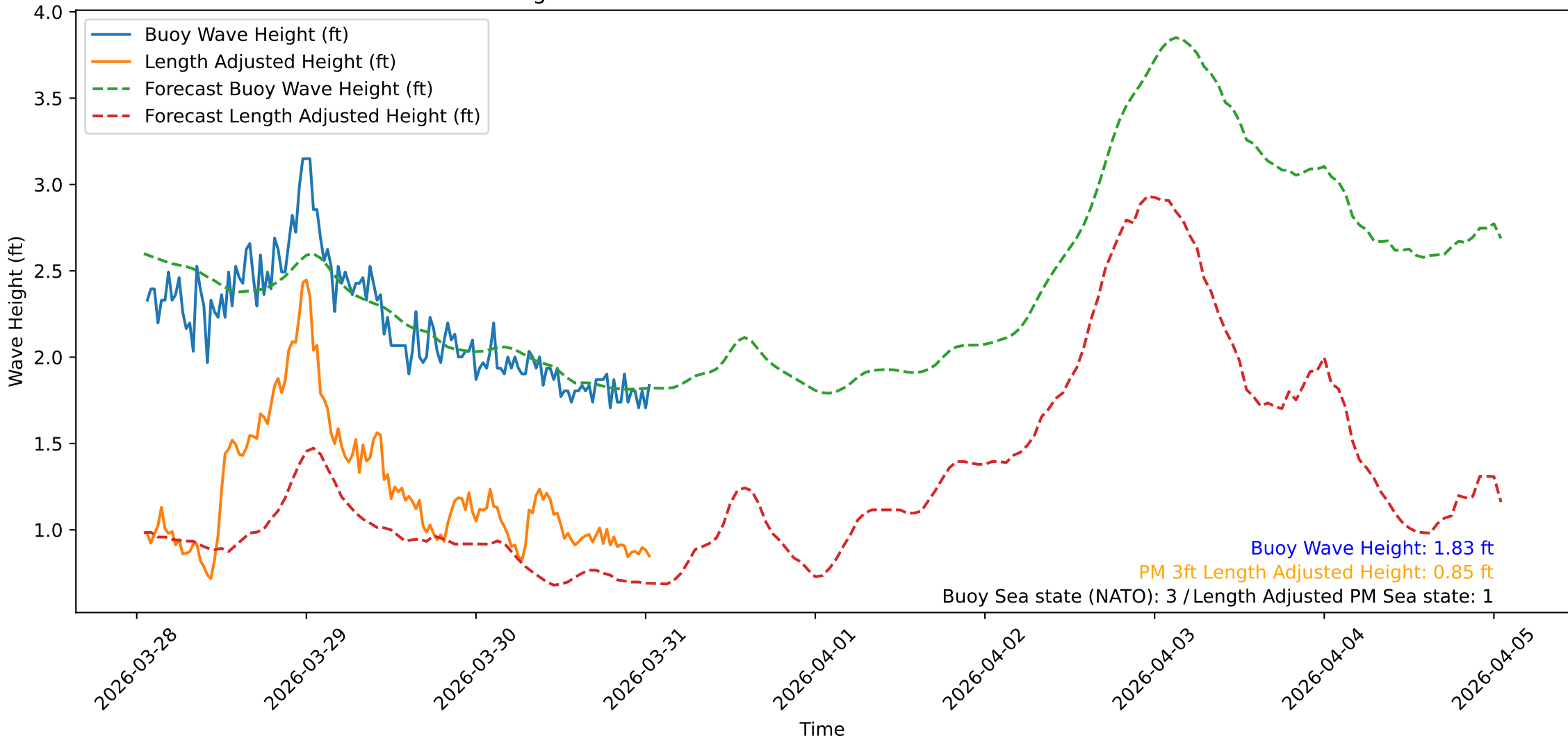
Wave Heights over Time for Oceanside Harbor at 2026-03-31 01:20:31
