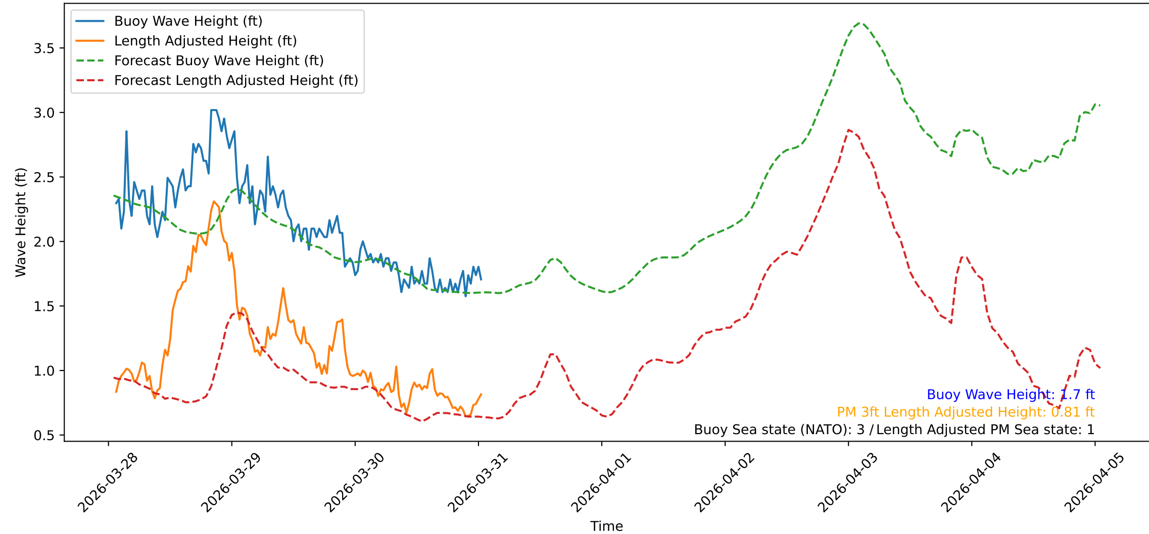
Wave Heights over Time for Red Beach at 2026-03-31 01:20:47
