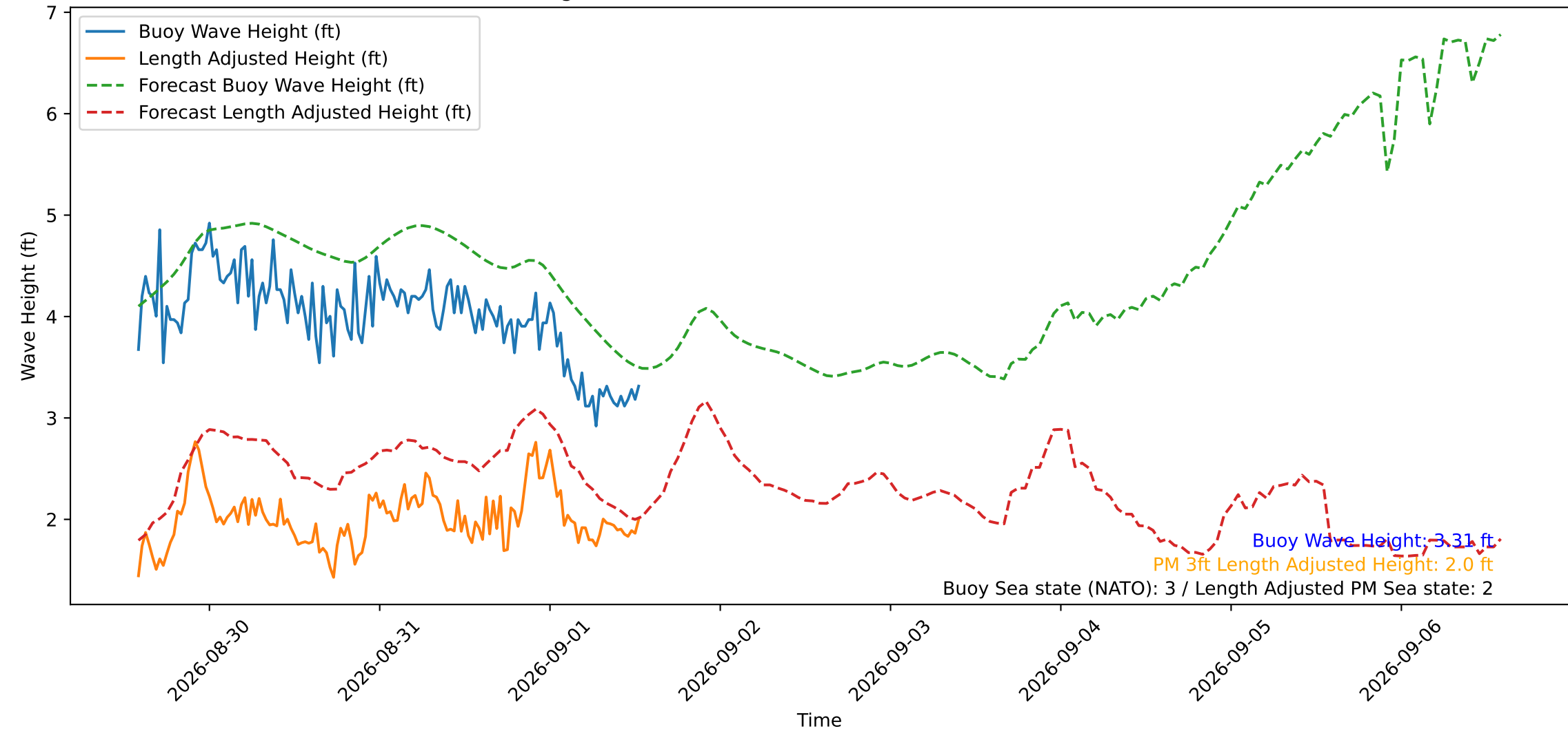
Wave Heights over Time for Green Beach at 2026-09-01 13:31:13
