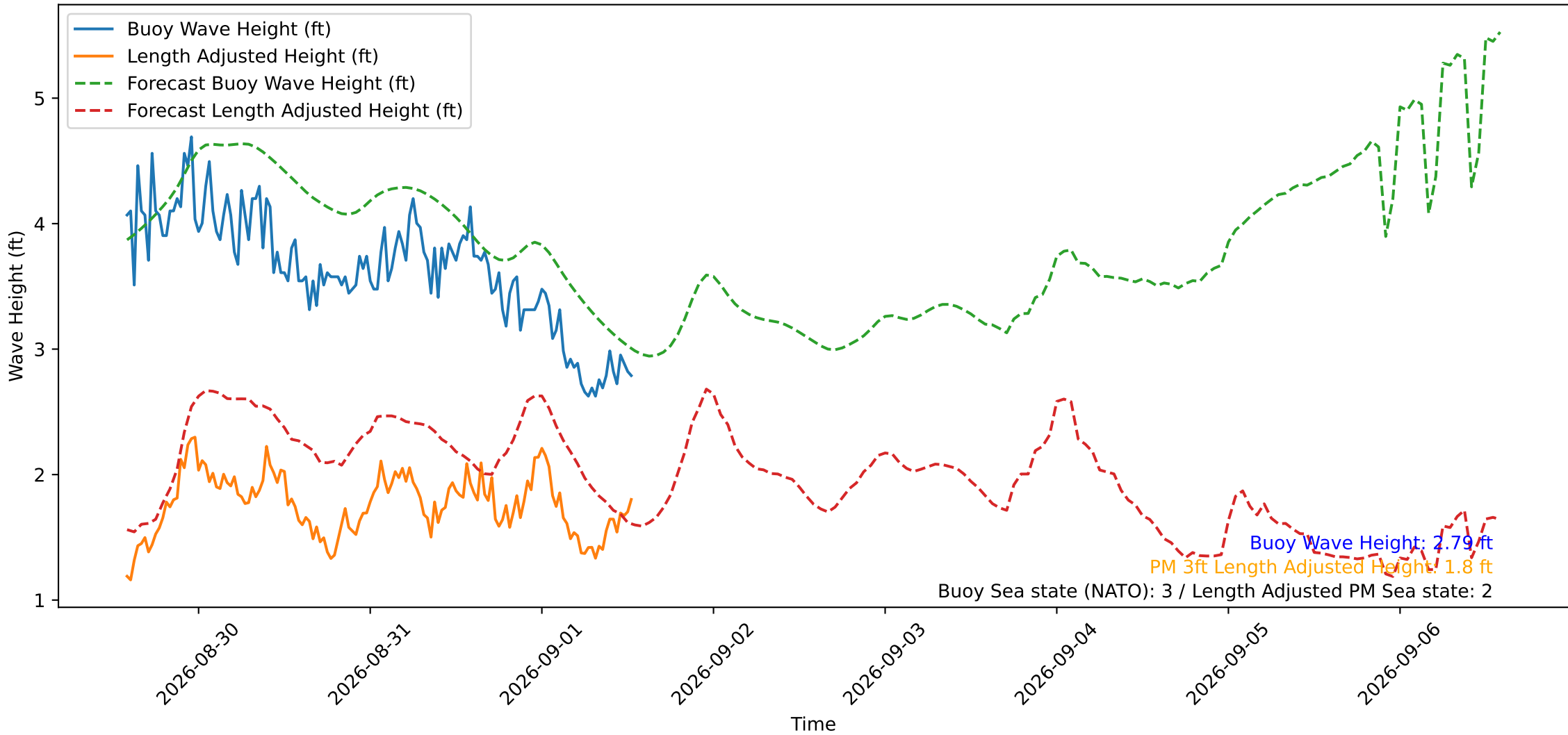
Wave Heights over Time for Red Beach at 2026-09-01 13:30:50
