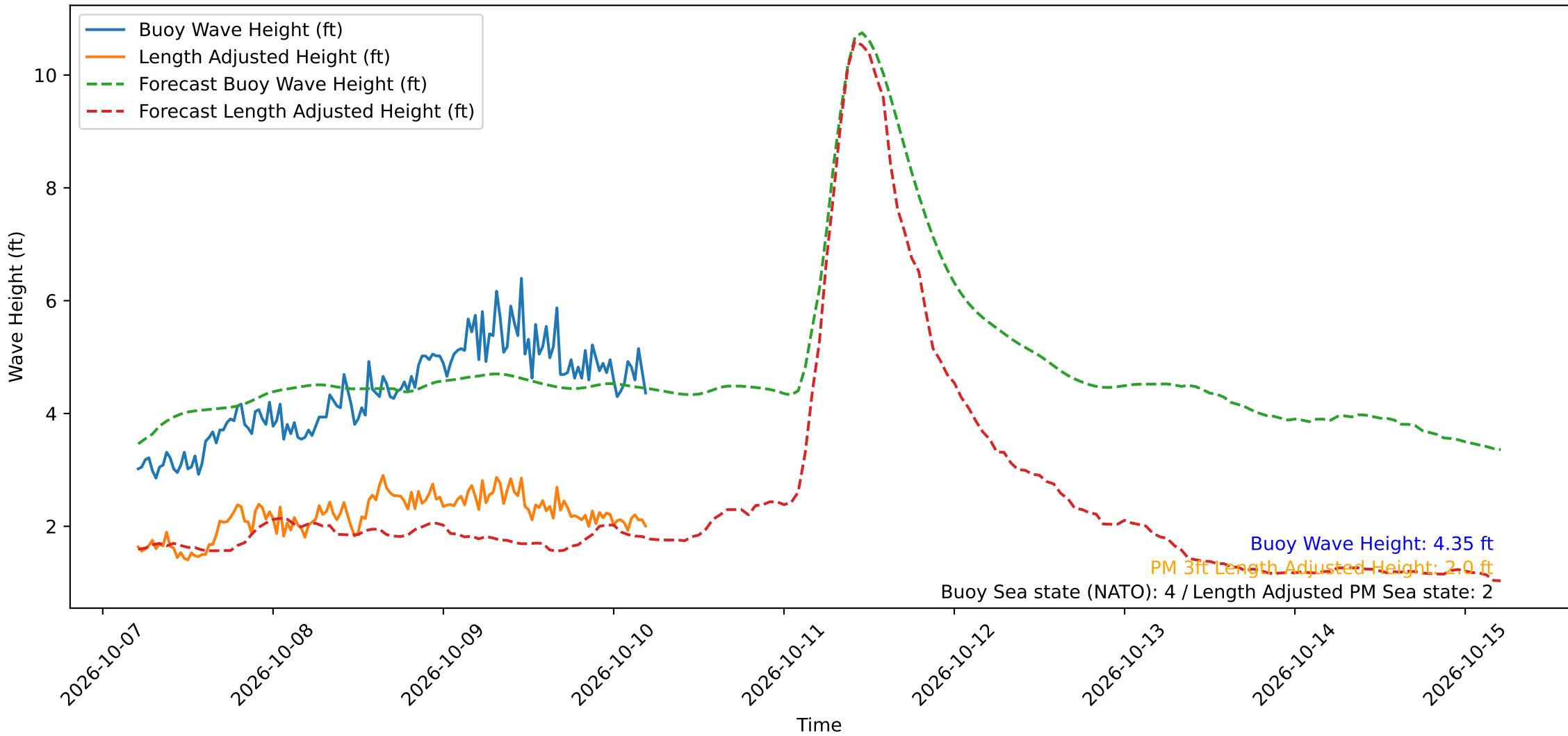
Wave Heights over Time for Oceanside Harbor at 2026-10-10 05:00:29
