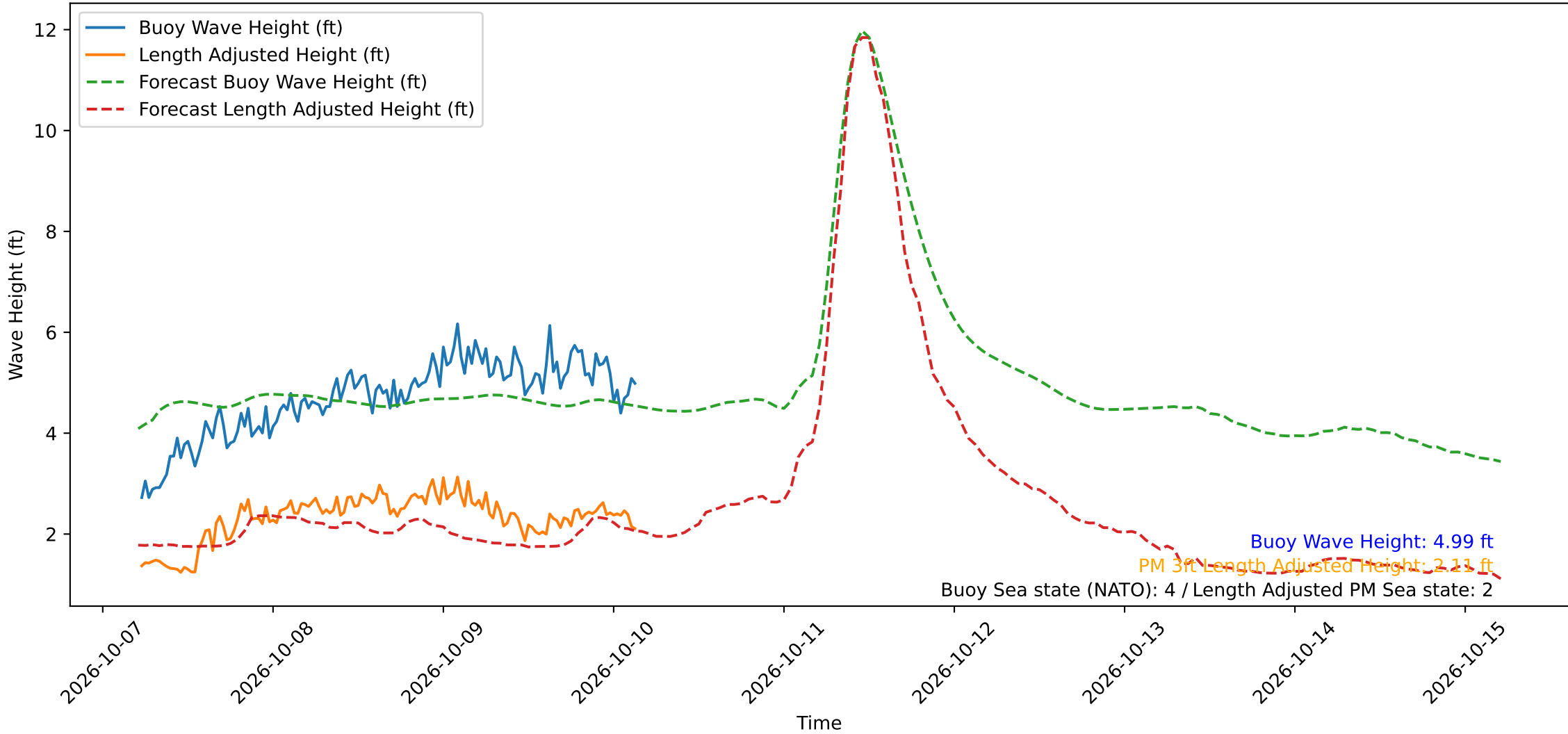
Wave Heights over Time for Green Beach at 2026-10-10 05:01:12
