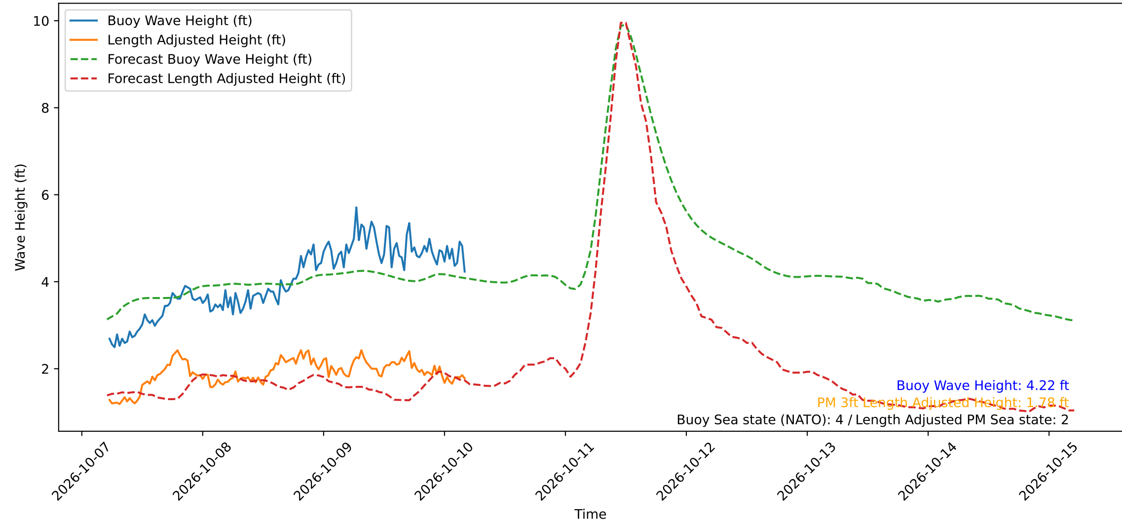
Wave Heights over Time for Red Beach at 2026-10-10 05:00:49
