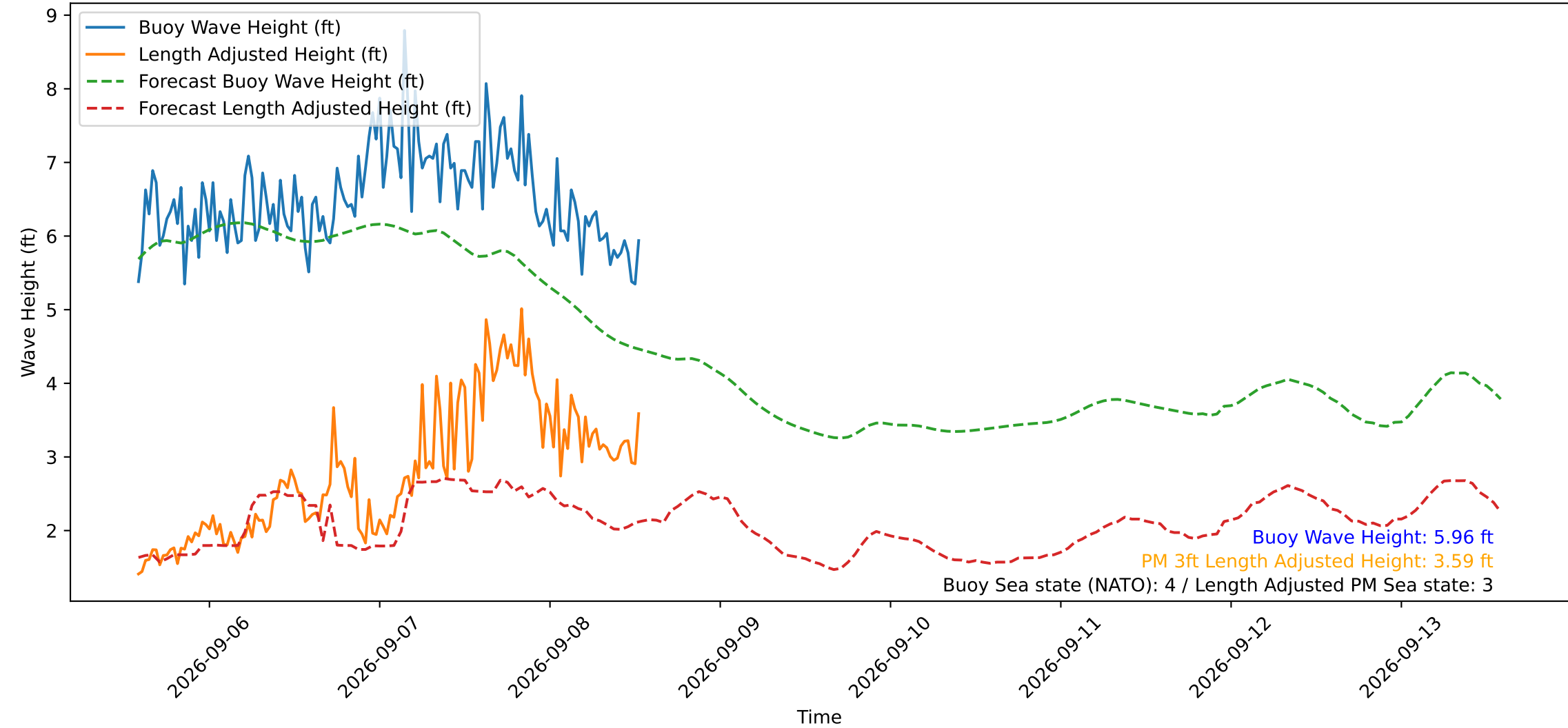
Wave Heights over Time for Green Beach at 2026-09-08 13:31:11
