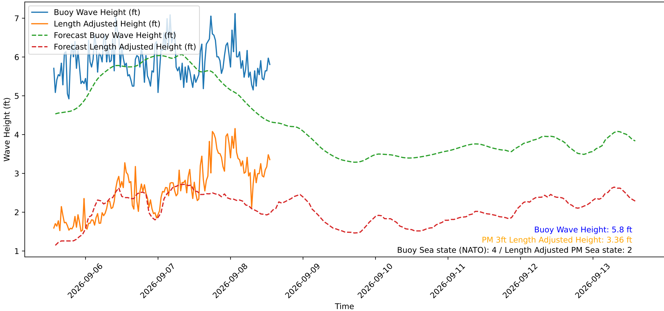
Wave Heights over Time for Oceanside Harbor at 2026-09-08 13:30:30
