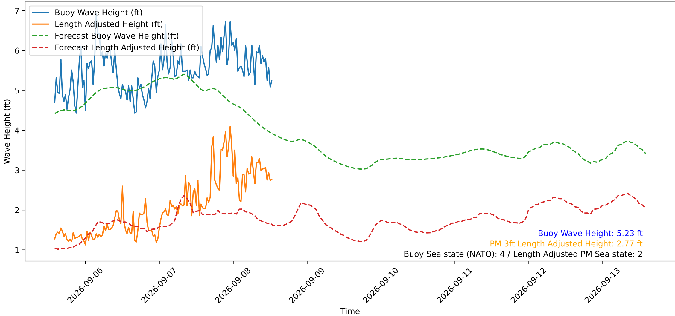
Wave Heights over Time for Red Beach at 2026-09-08 13:30:49
