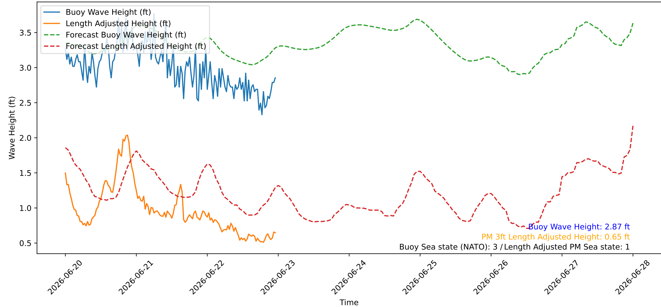
Wave Heights over Time for Red Beach at 2026-06-22 23:50:47
