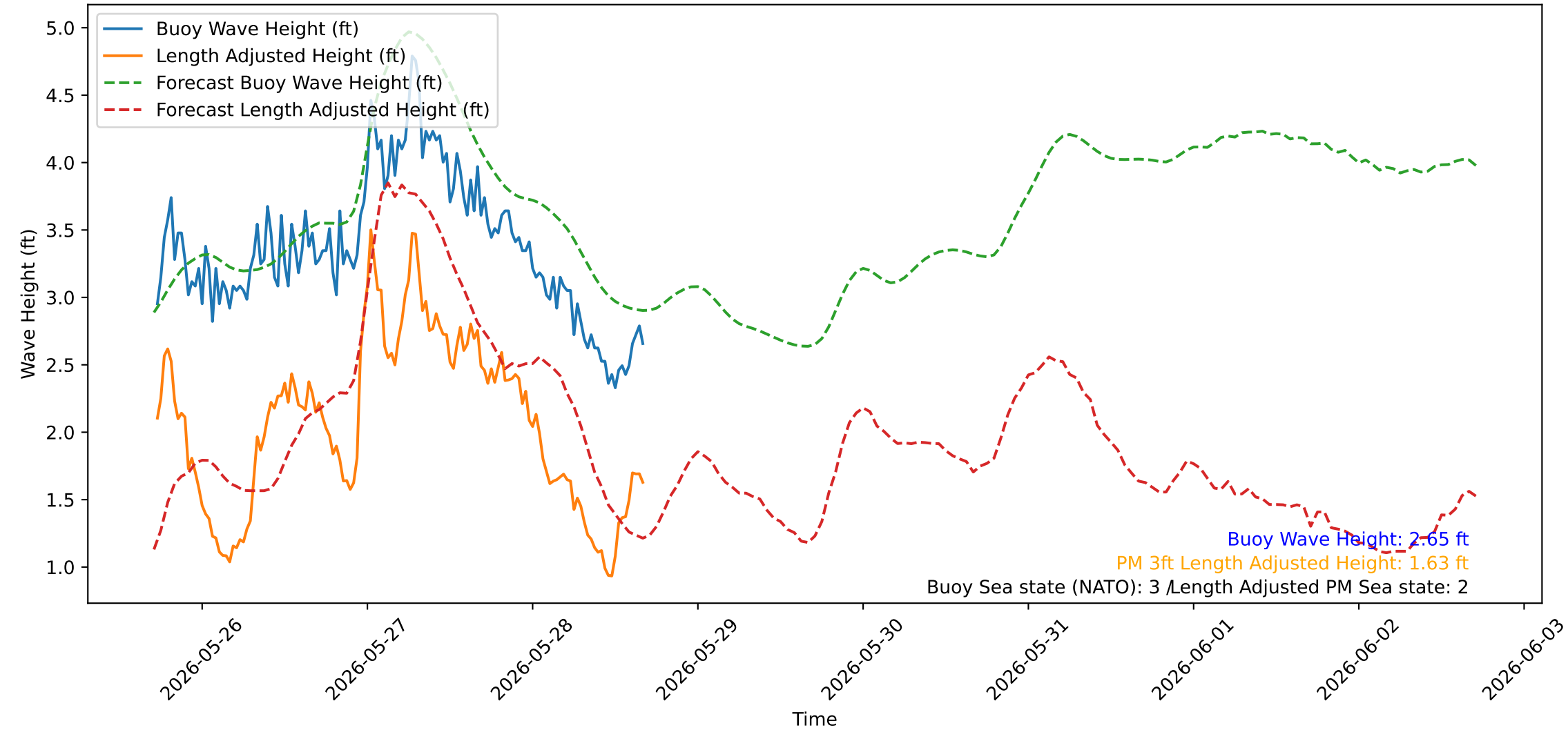
Wave Heights over Time for Red Beach at 2026-05-28 17:00:38
