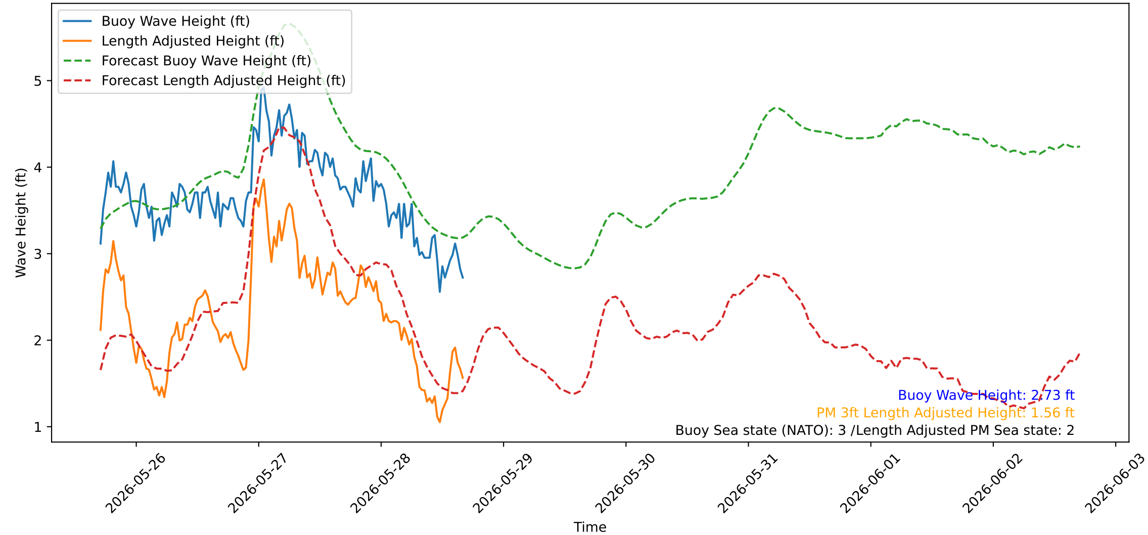
Wave Heights over Time for Green Beach at 2026-05-28 17:01:00
