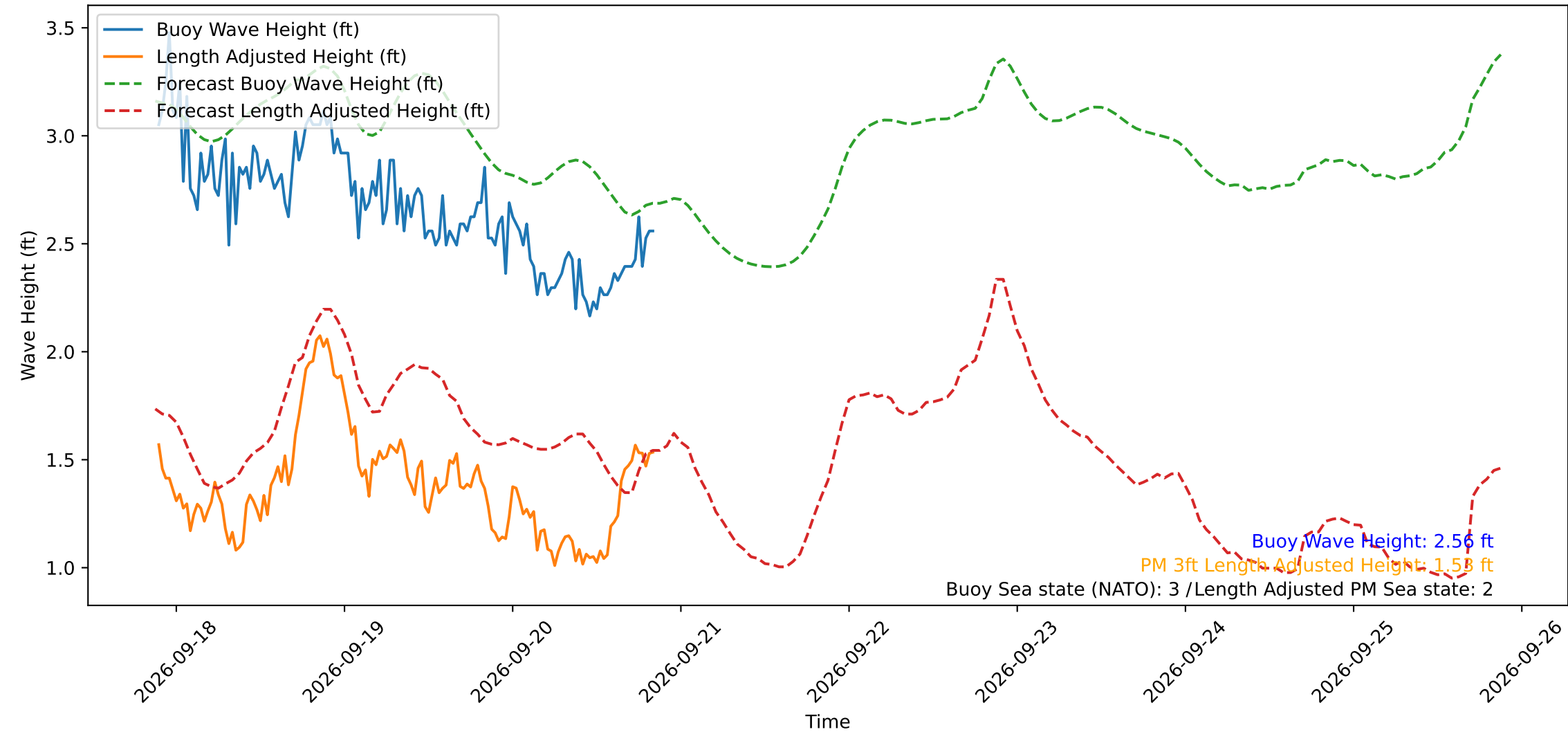
Wave Heights over Time for Green Beach at 2026-09-20 21:01:11
