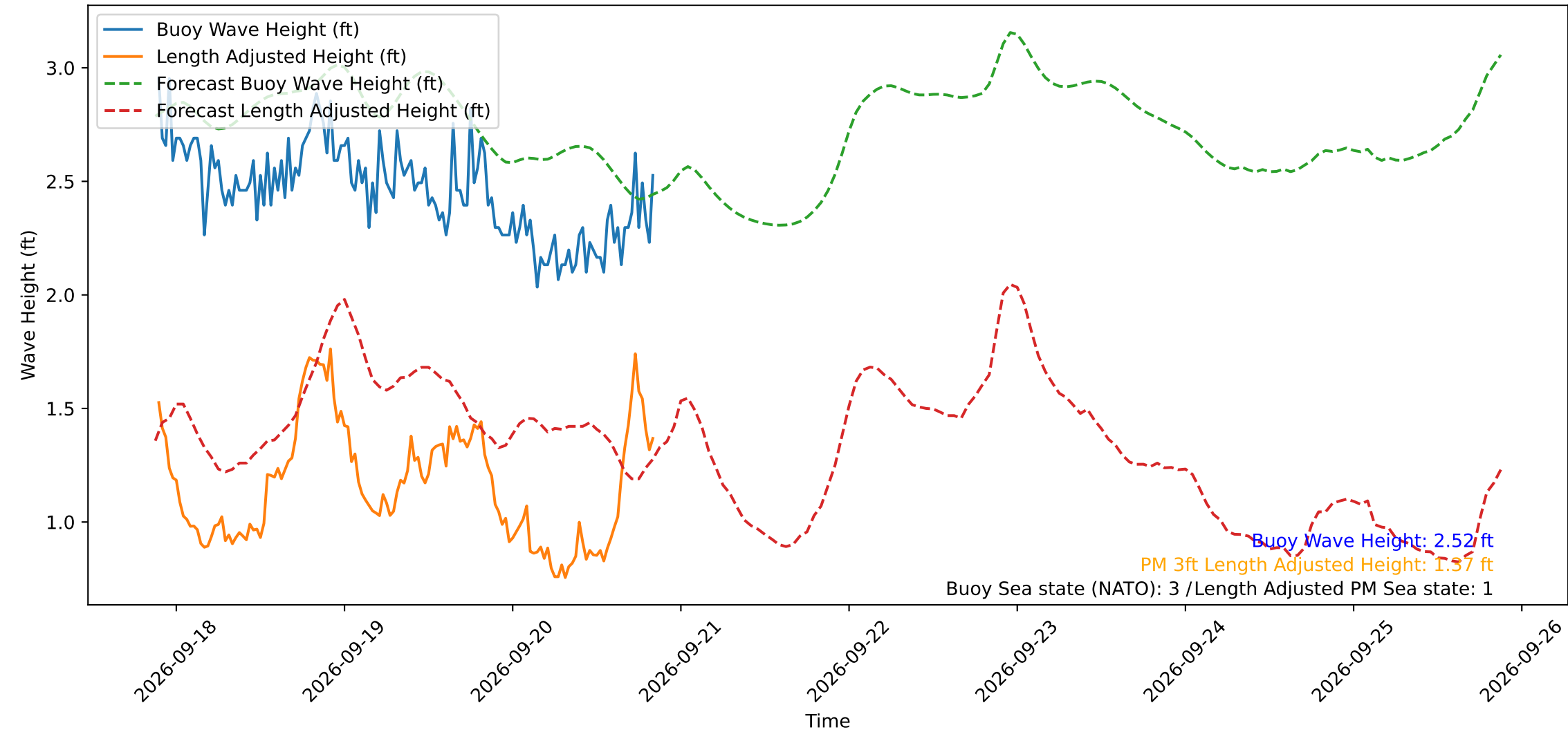
Wave Heights over Time for Red Beach at 2026-09-20 21:00:49
