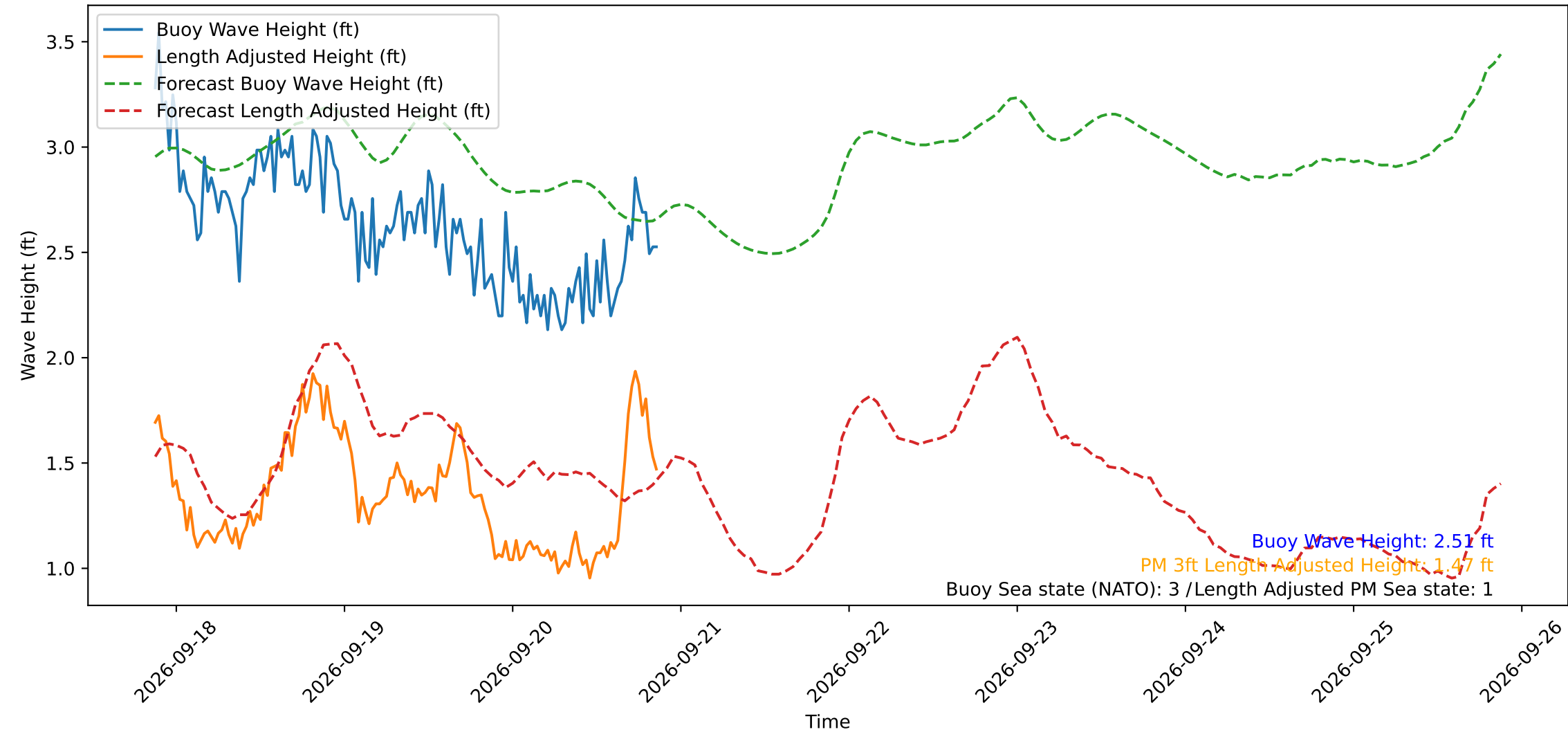
Wave Heights over Time for Oceanside Harbor at 2026-09-20 21:00:30
