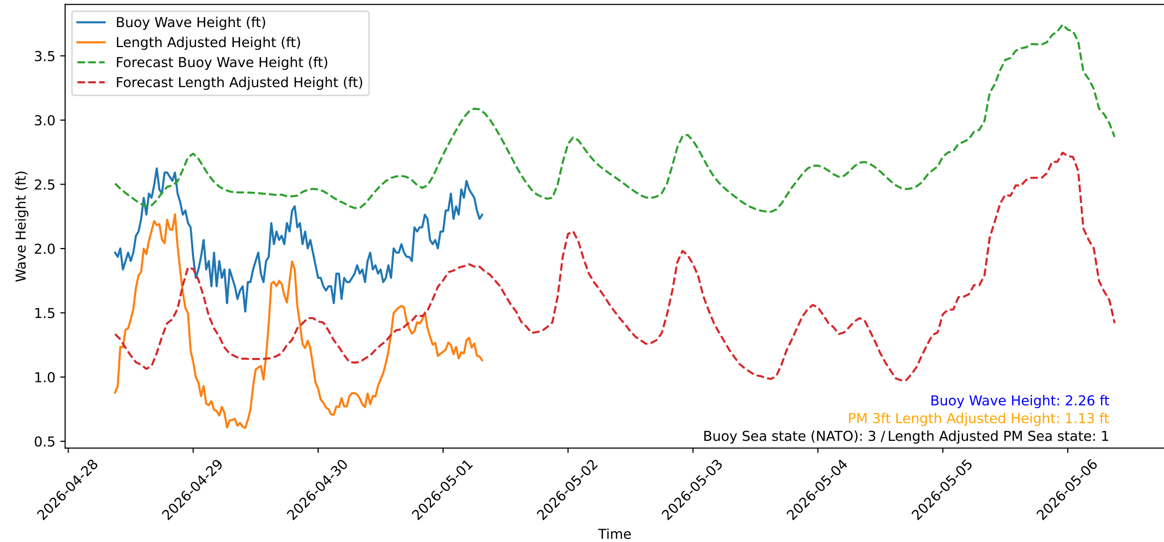
Wave Heights over Time for Red Beach at 2026-05-01 08:30:51
