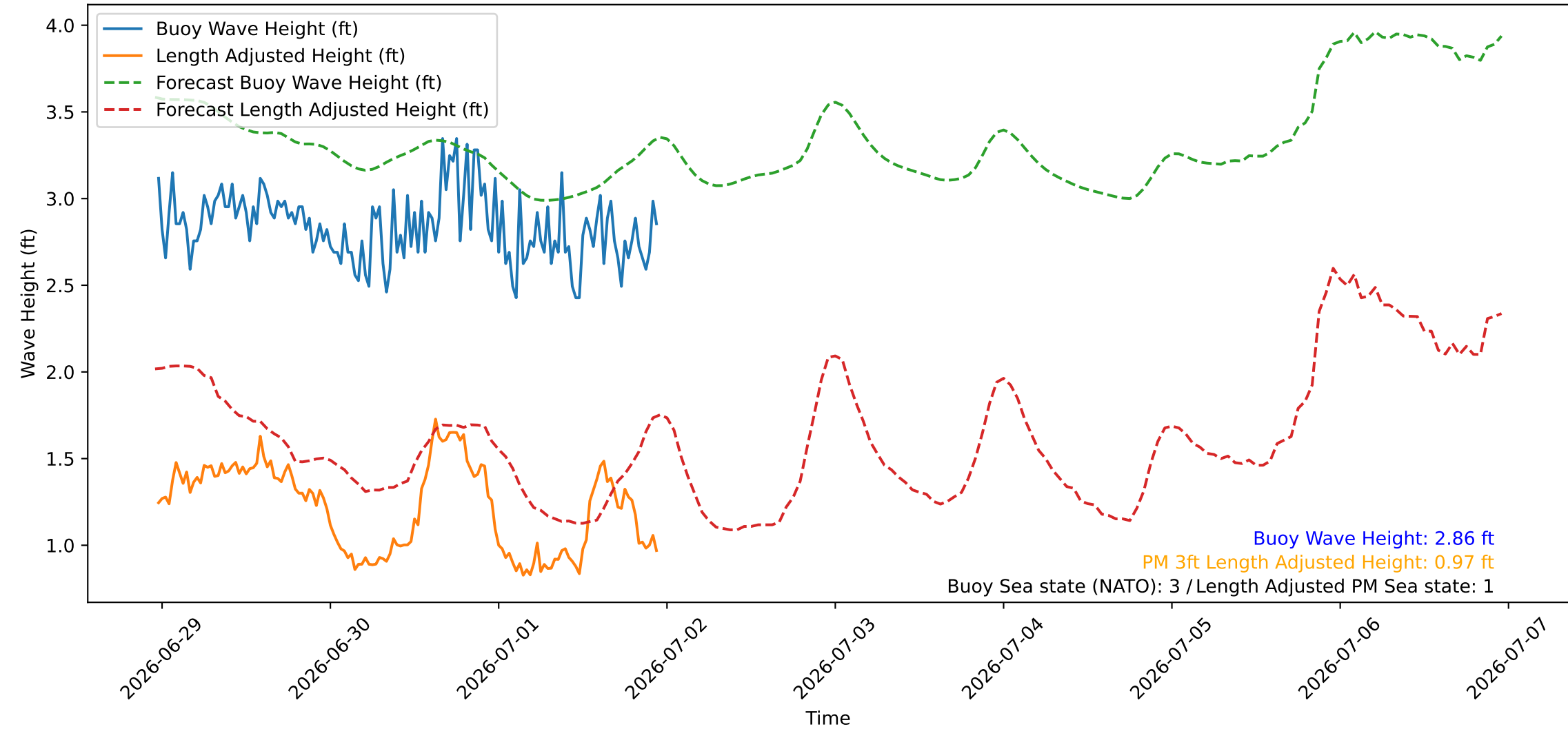
Wave Heights over Time for Red Beach at 2026-07-01 23:20:46
