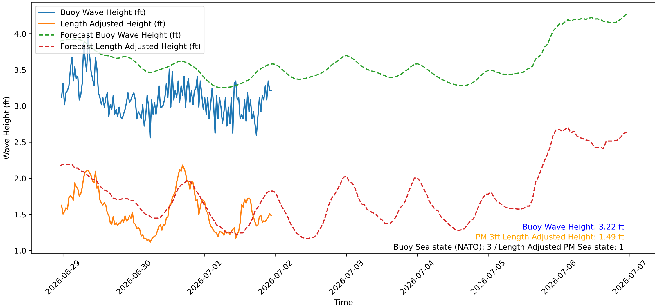
Wave Heights over Time for Oceanside Harbor at 2026-07-01 23:20:26
