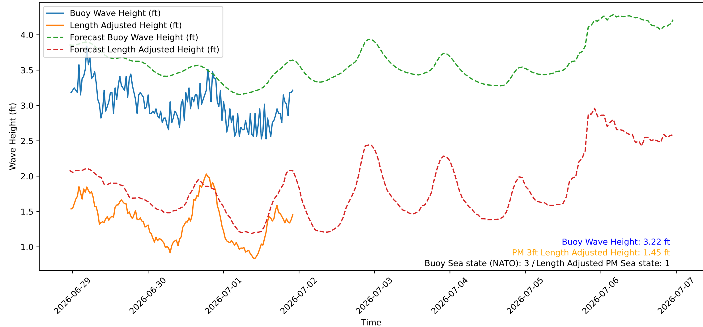
Wave Heights over Time for Green Beach at 2026-07-01 23:21:08
