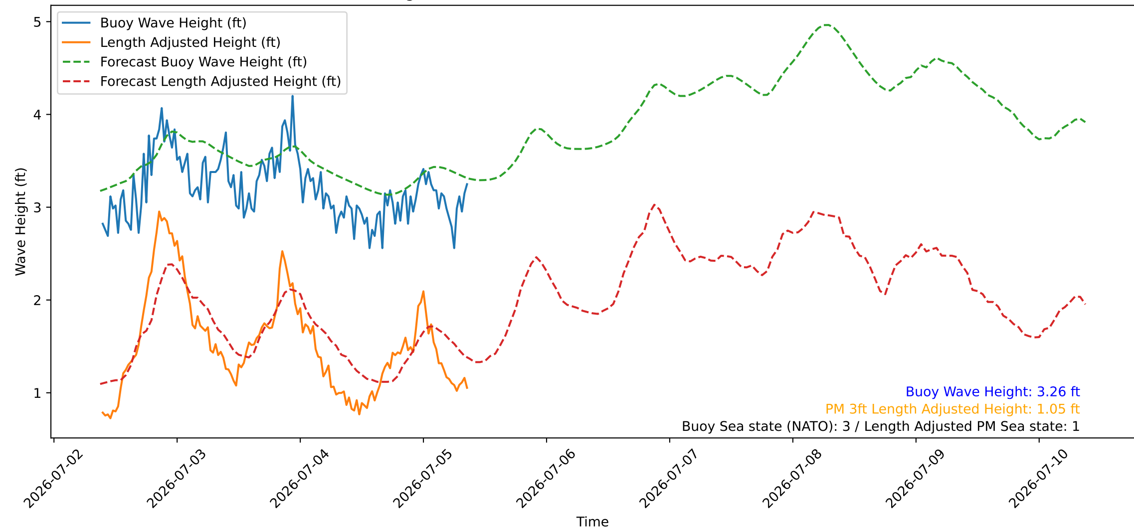
Wave Heights over Time for Green Beach at 2026-07-05 09:21:09
