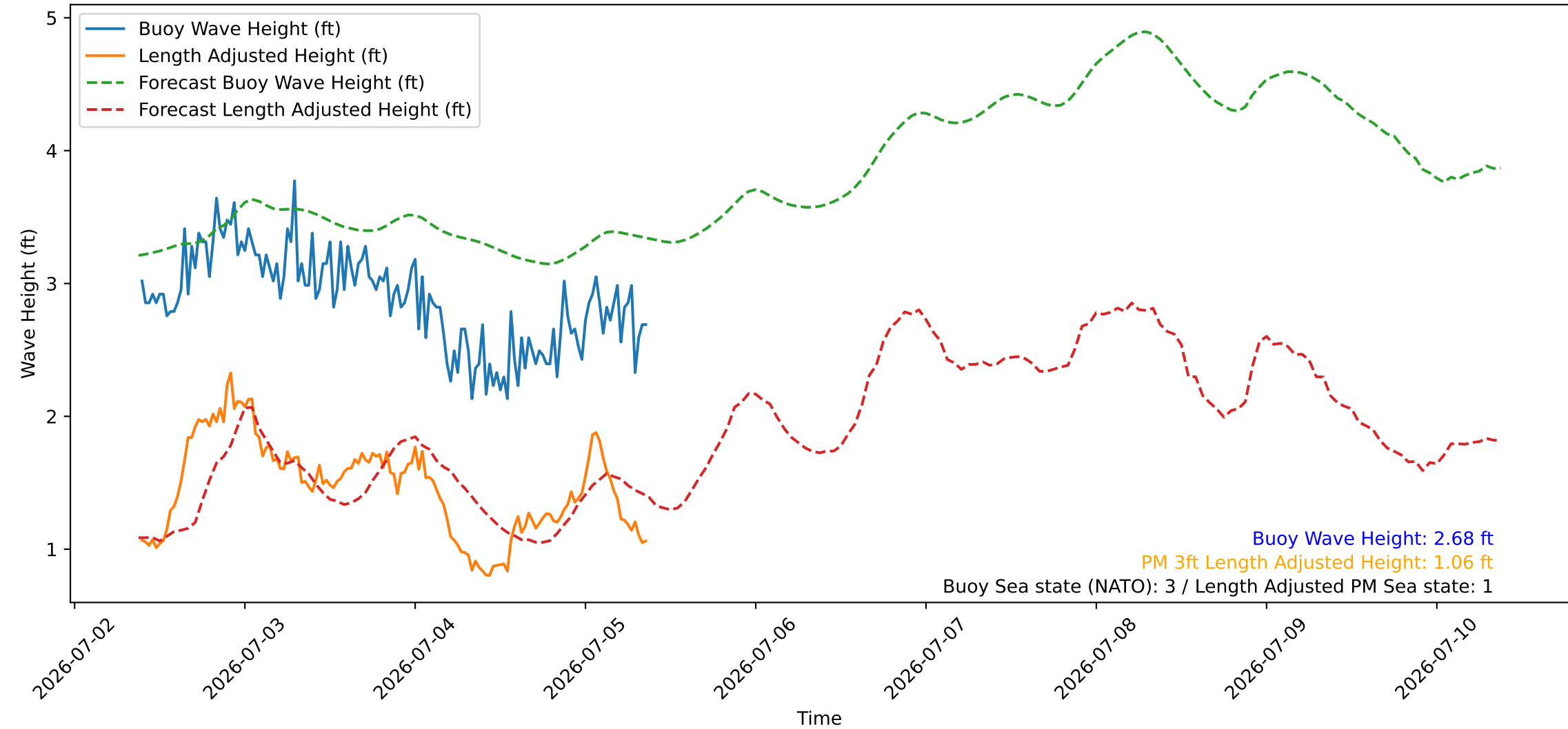
Wave Heights over Time for Oceanside Harbor at 2026-07-05 09:20:26
