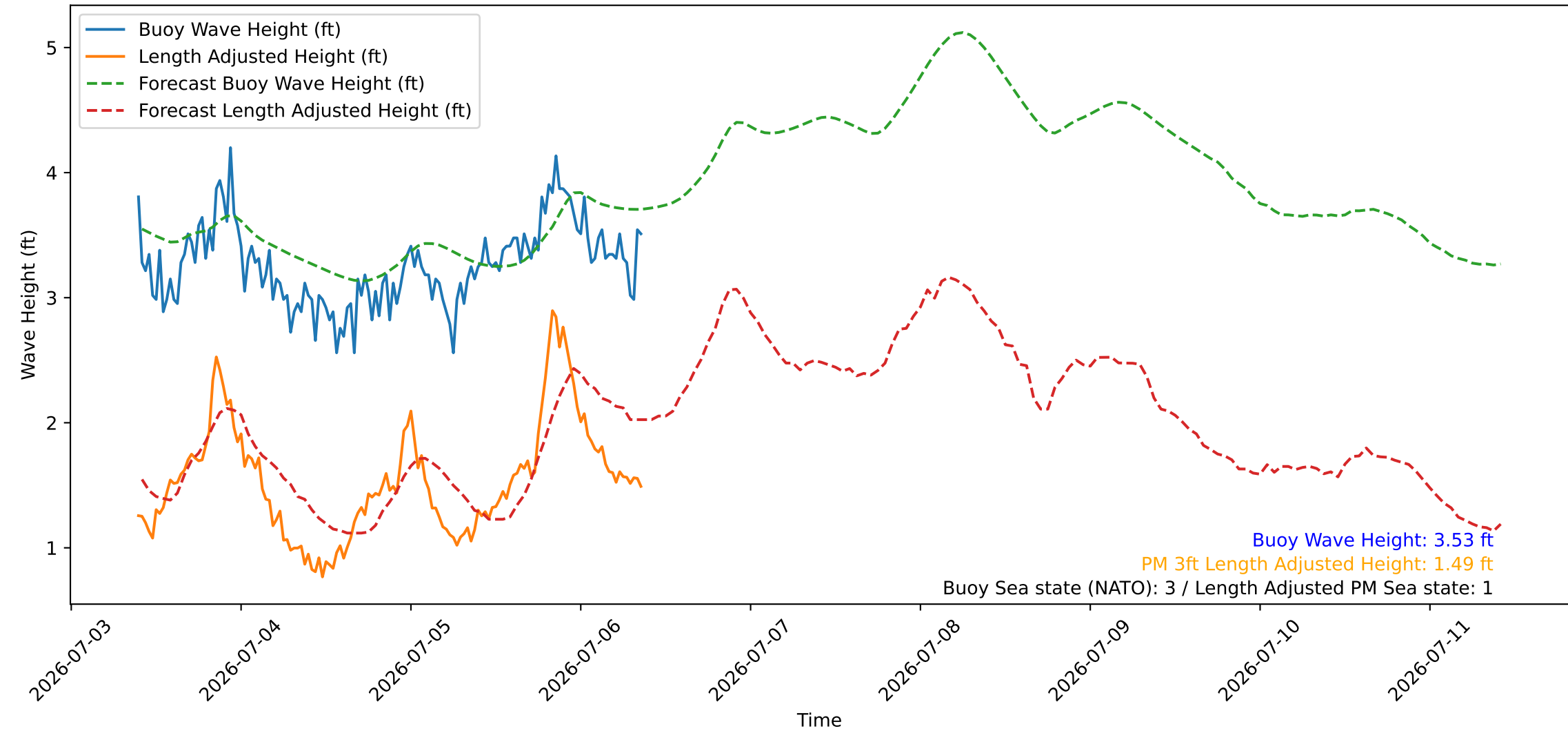
Wave Heights over Time for Green Beach at 2026-07-06 09:31:07
