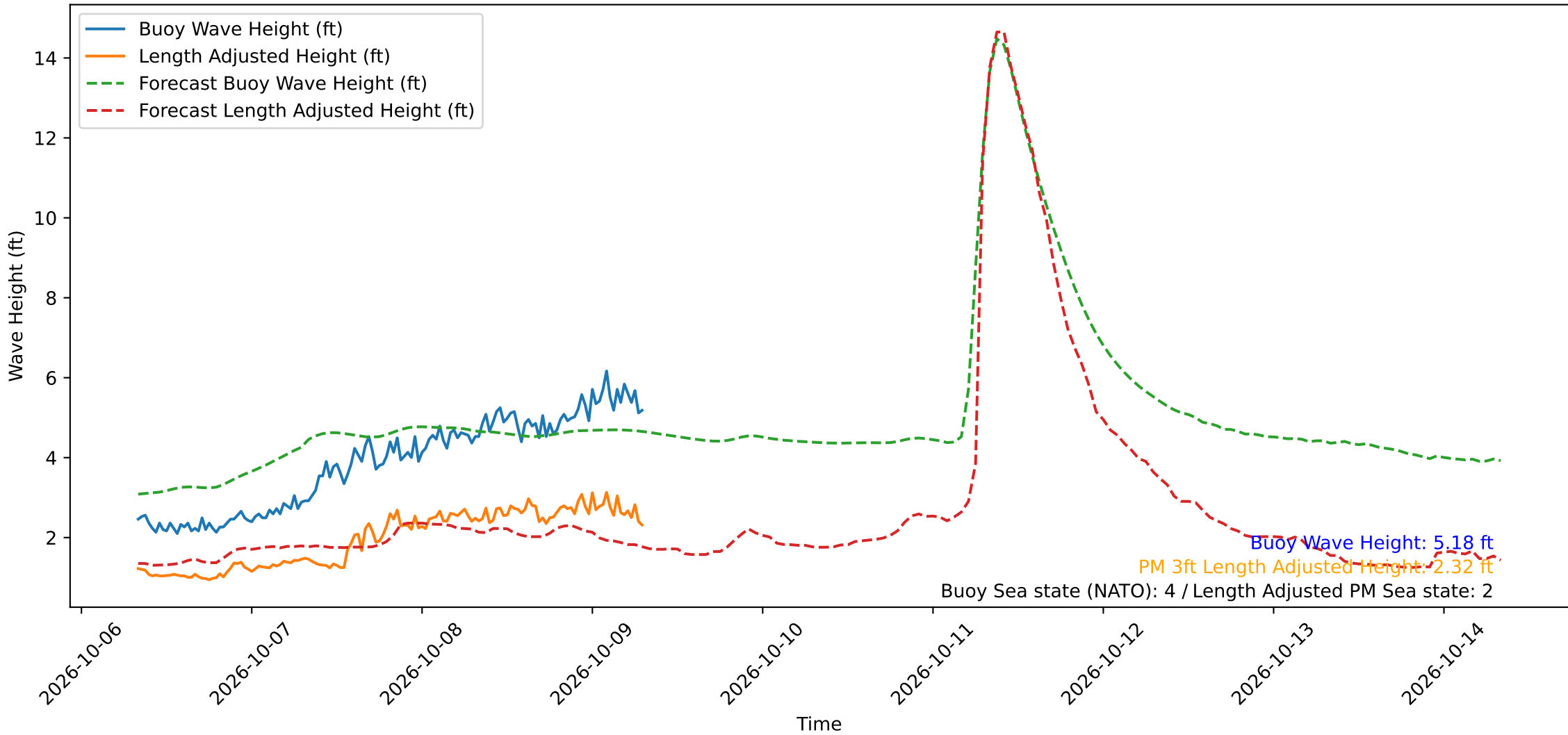
Wave Heights over Time for Green Beach at 2026-10-09 07:41:11
