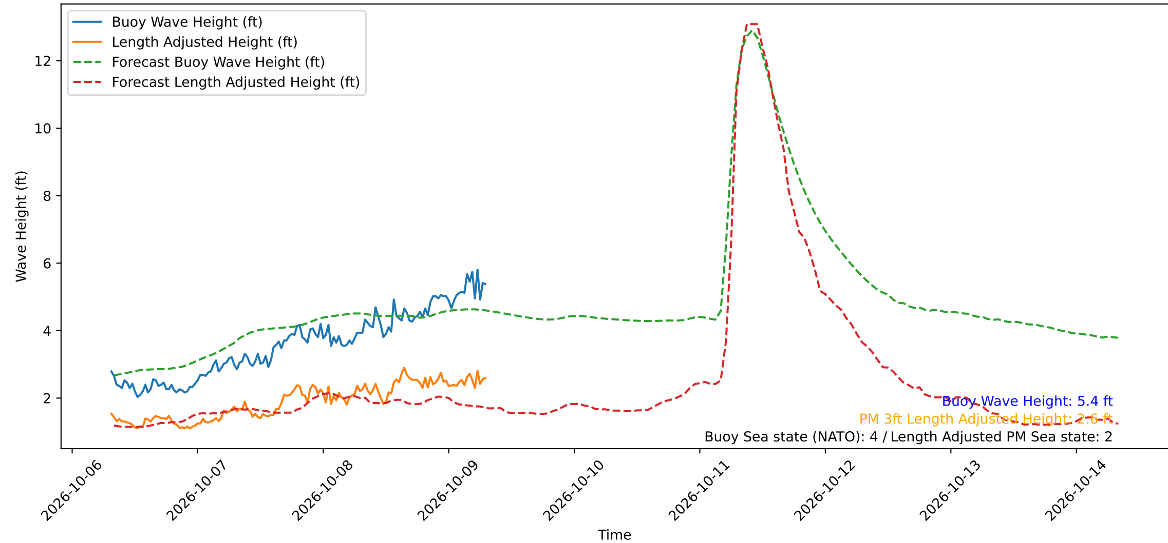
Wave Heights over Time for Oceanside Harbor at 2026-10-09 07:40:29
