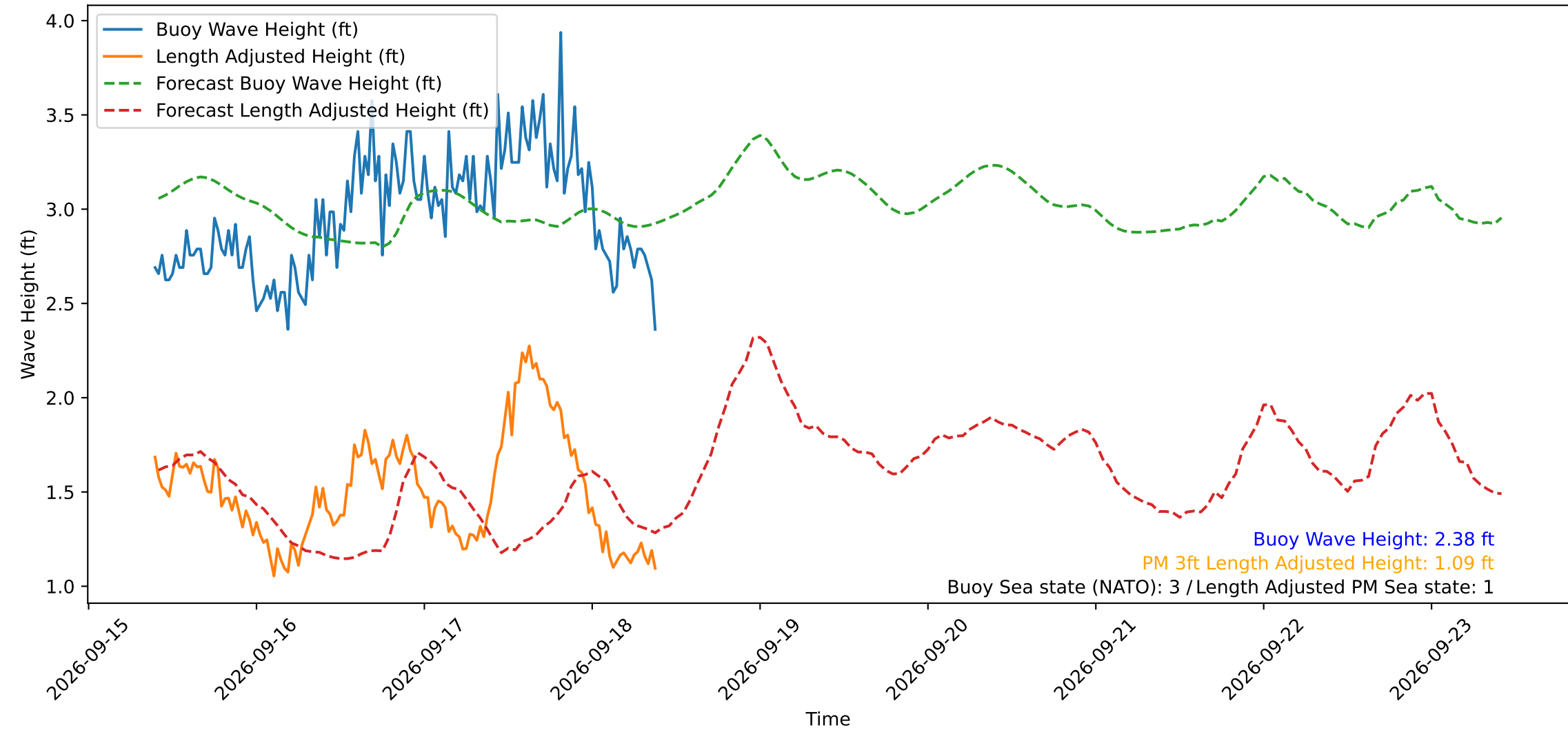
Wave Heights over Time for Oceanside Harbor at 2026-09-18 09:40:29
