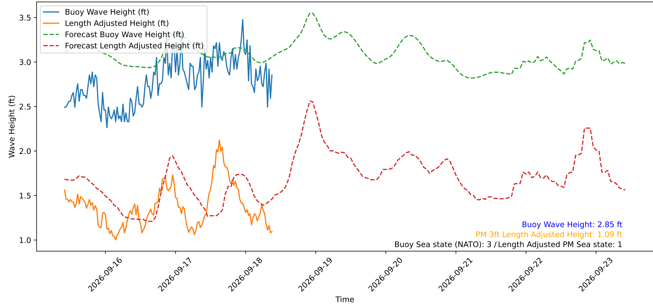
Wave Heights over Time for Green Beach at 2026-09-18 09:41:12
