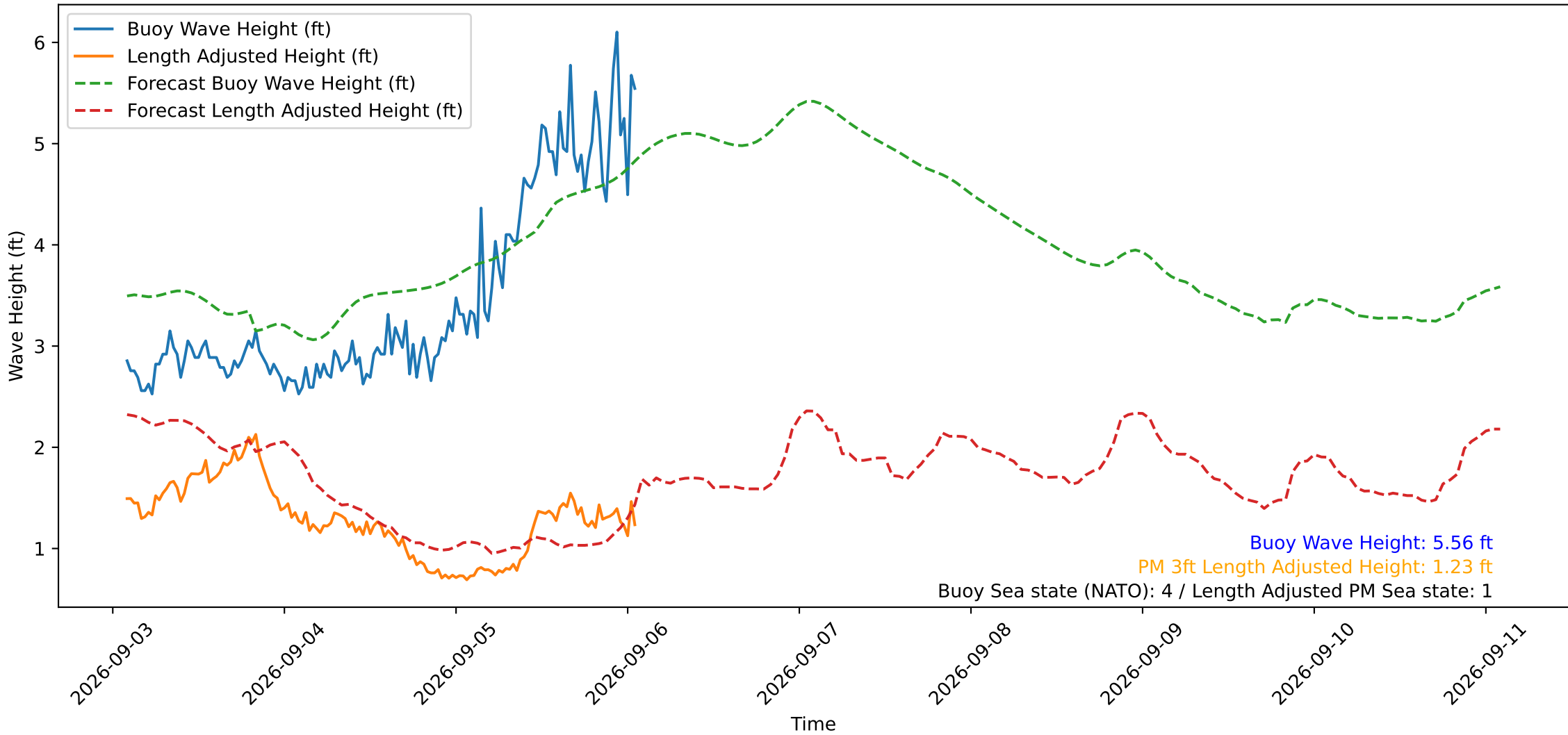
Wave Heights over Time for Red Beach at 2026-09-06 01:40:49
