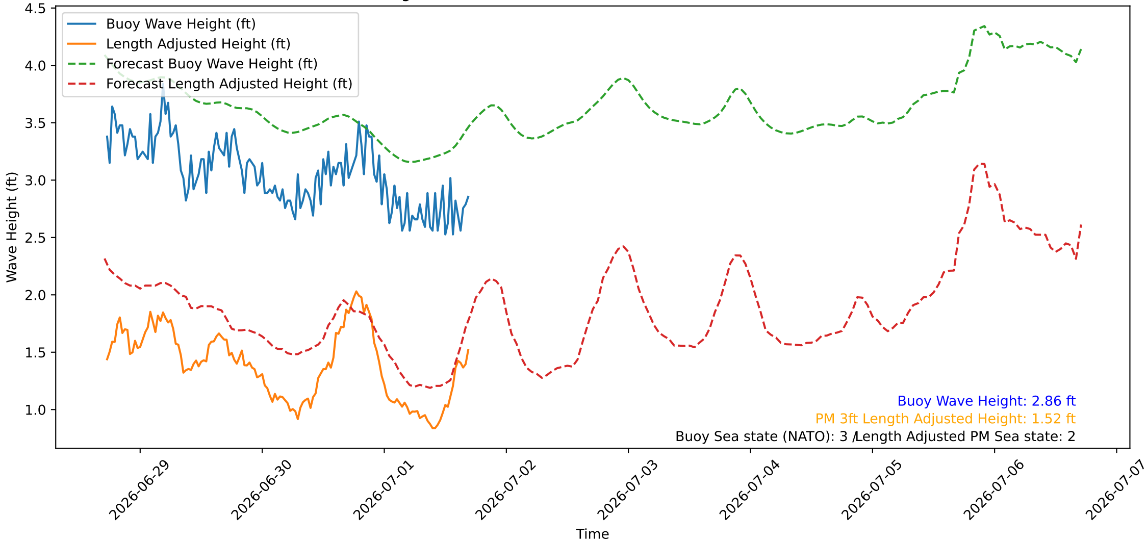
Wave Heights over Time for Green Beach at 2026-07-01 17:21:08
