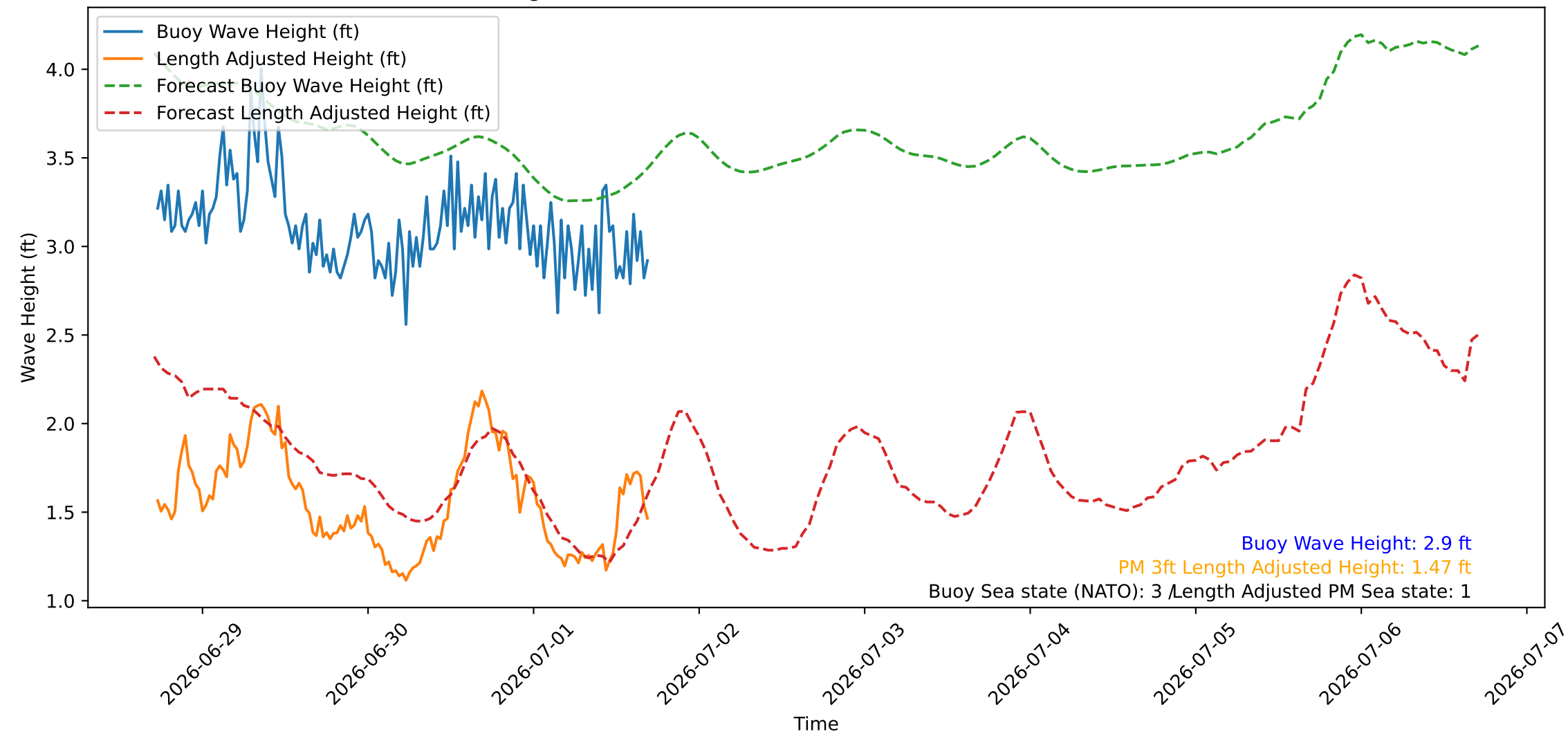
Wave Heights over Time for Oceanside Harbor at 2026-07-01 17:20:26
