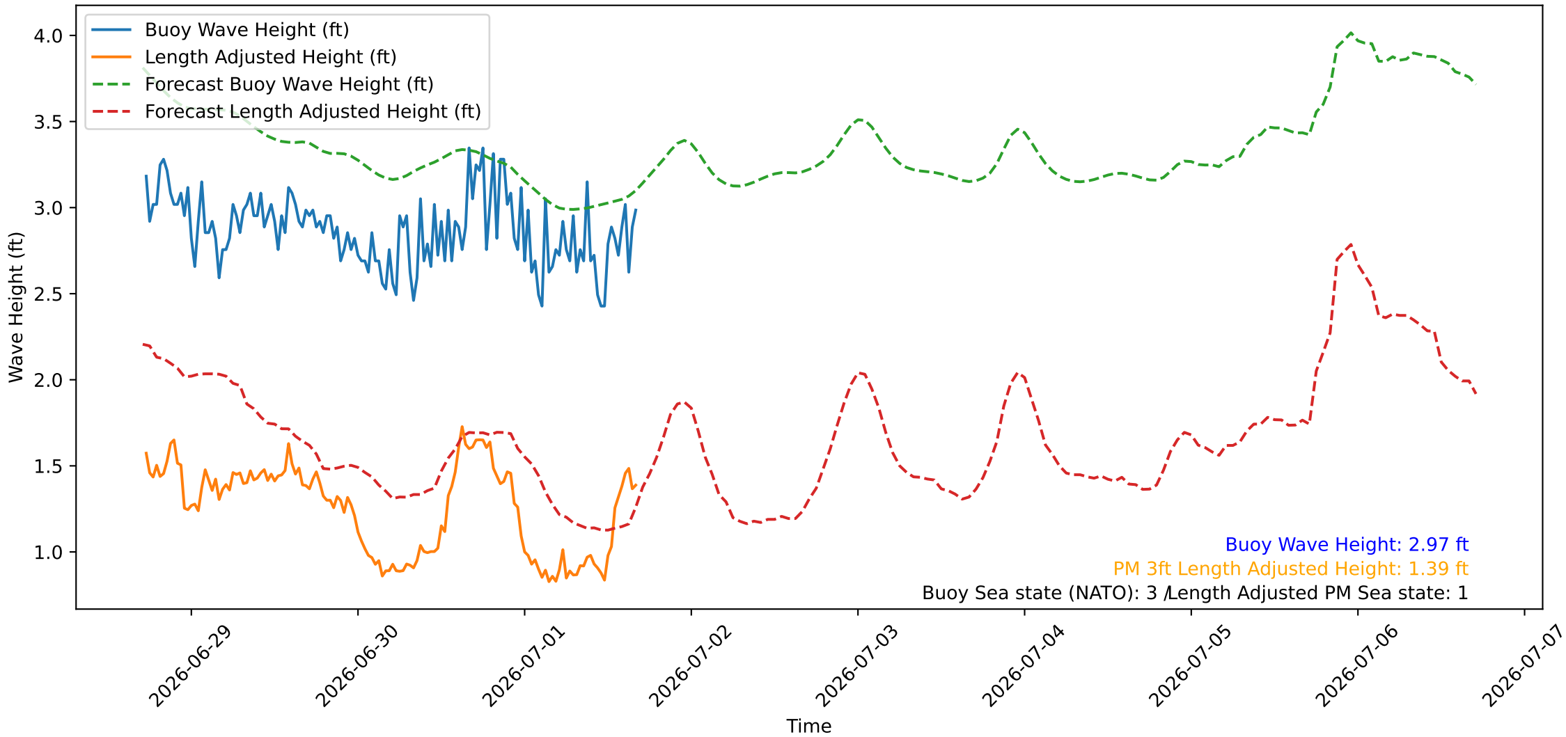
Wave Heights over Time for Red Beach at 2026-07-01 17:20:47
