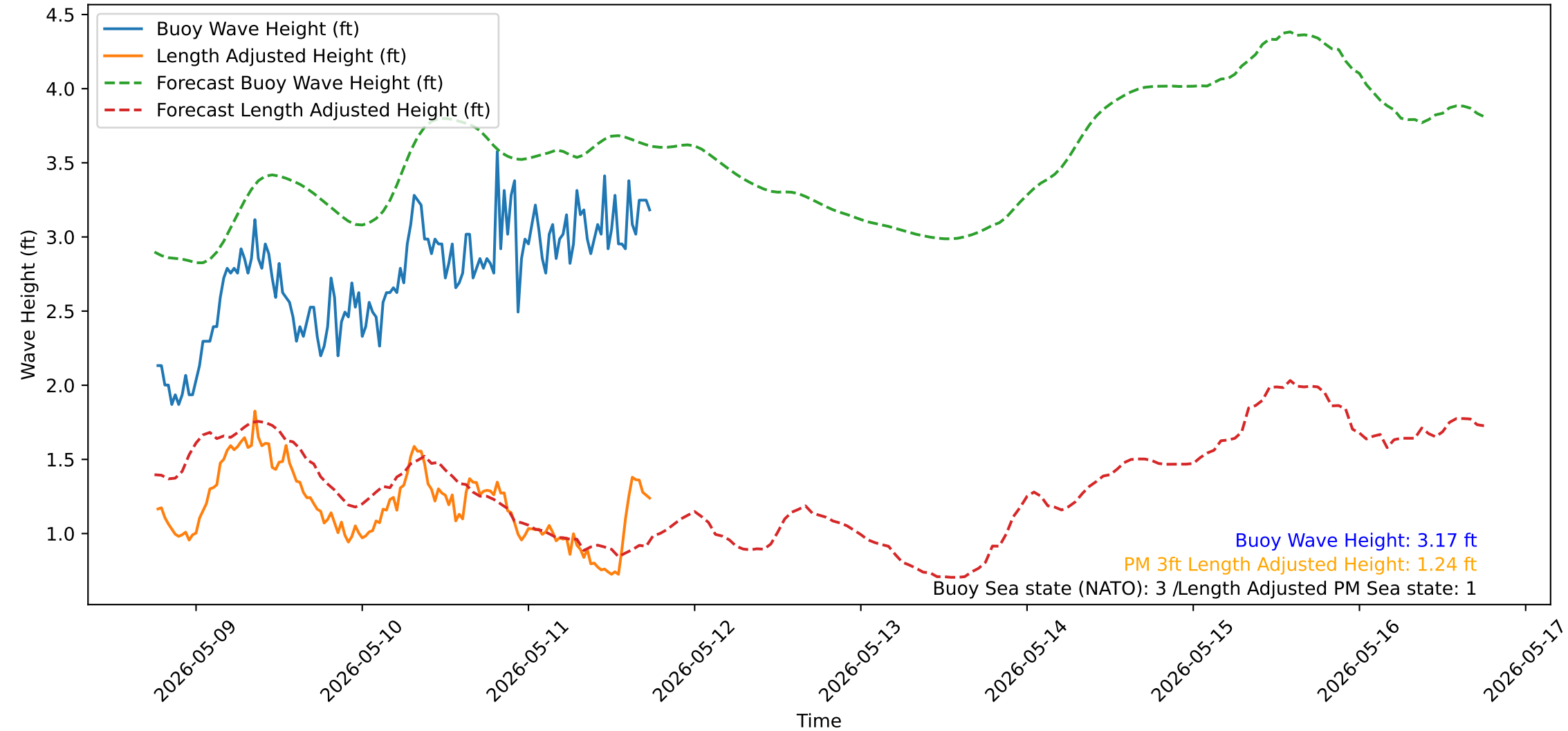
Wave Heights over Time for Oceanside Harbor at 2026-05-11 18:20:31
