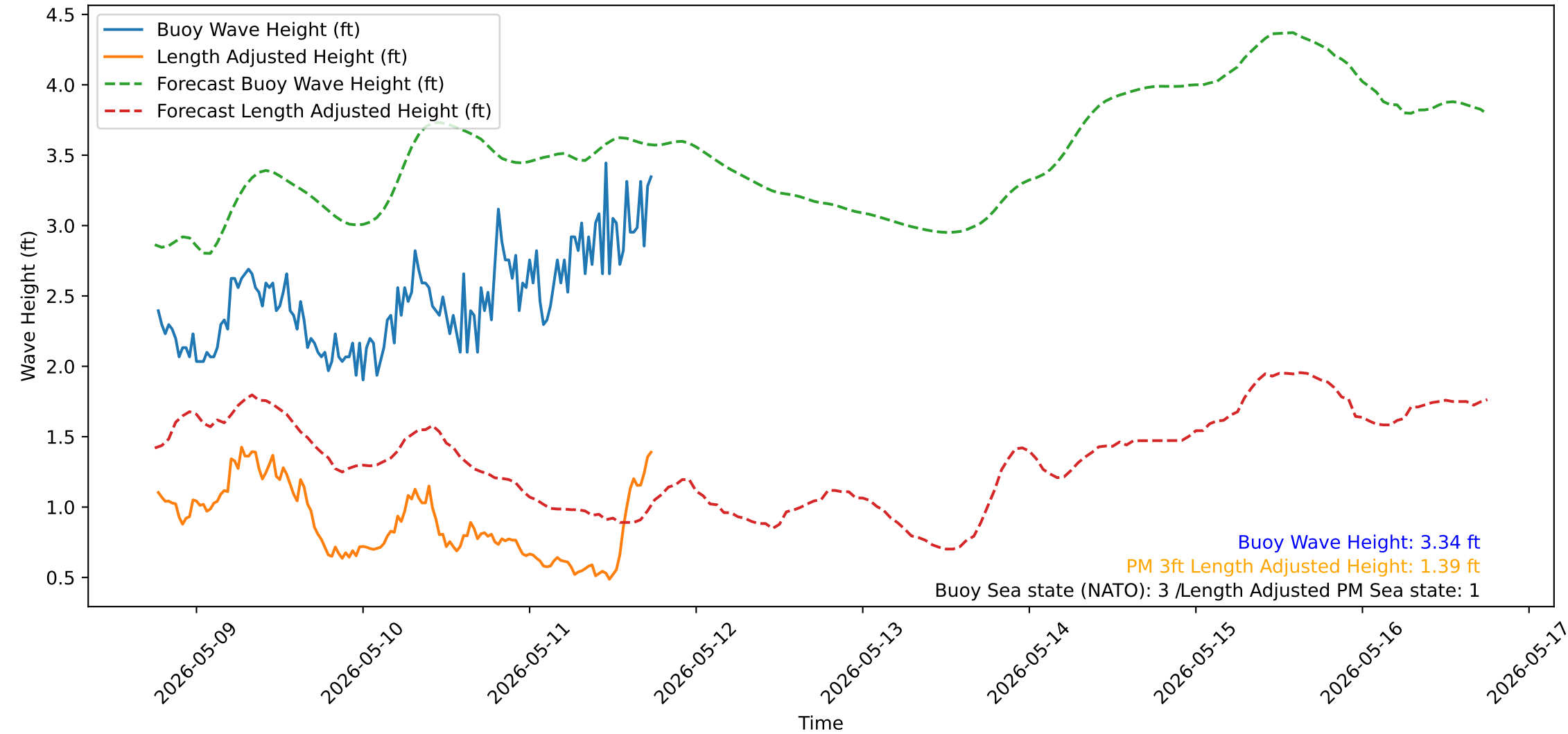
Wave Heights over Time for Green Beach at 2026-05-11 18:21:14
