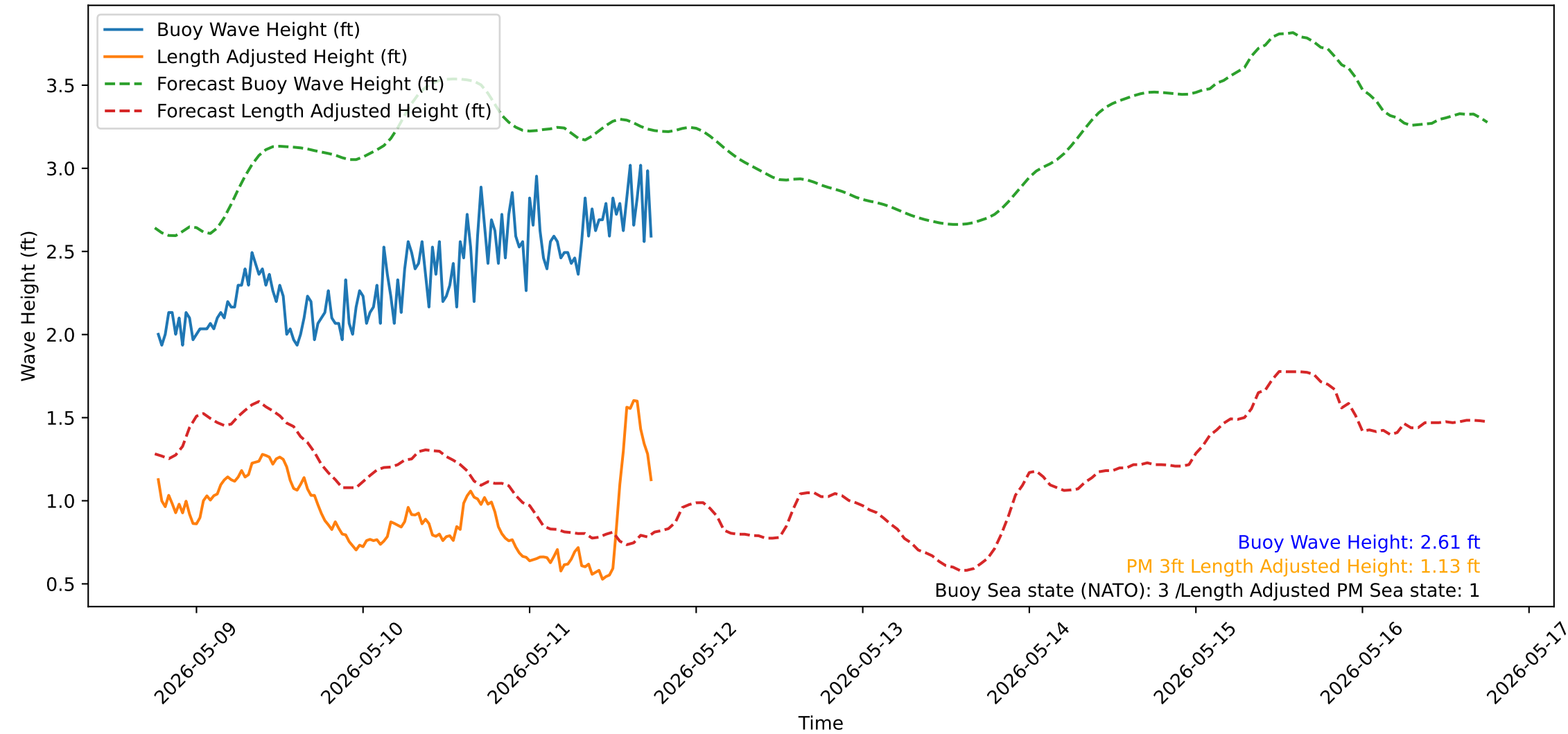
Wave Heights over Time for Red Beach at 2026-05-11 18:20:51
