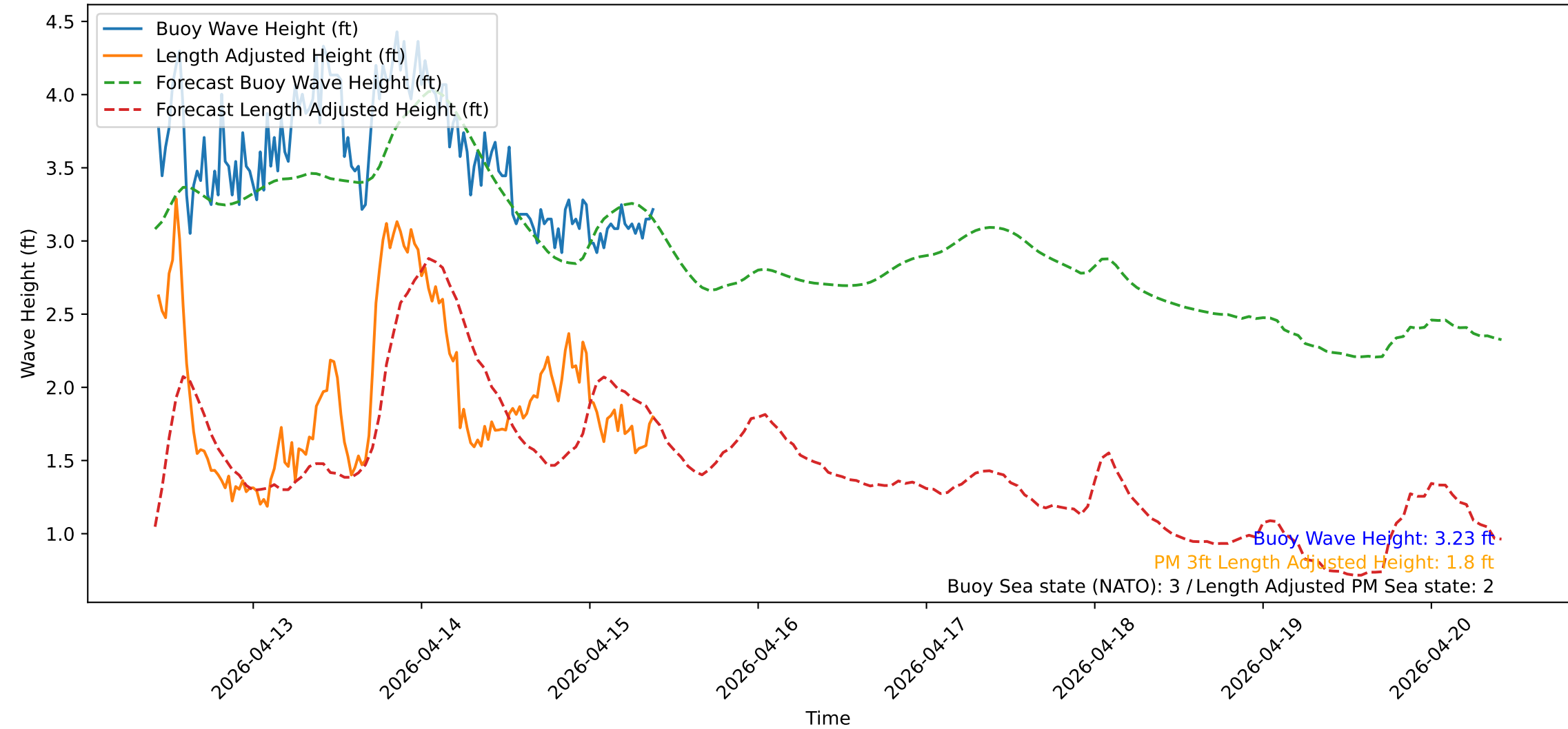
Wave Heights over Time for Red Beach at 2026-04-15 10:00:51
