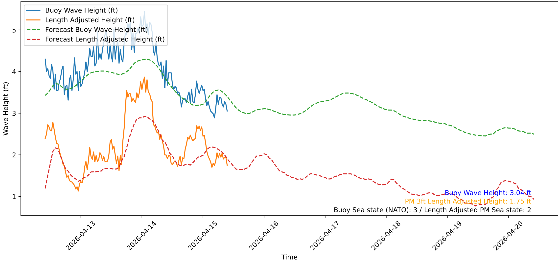
Wave Heights over Time for Oceanside Harbor at 2026-04-15 10:00:32
