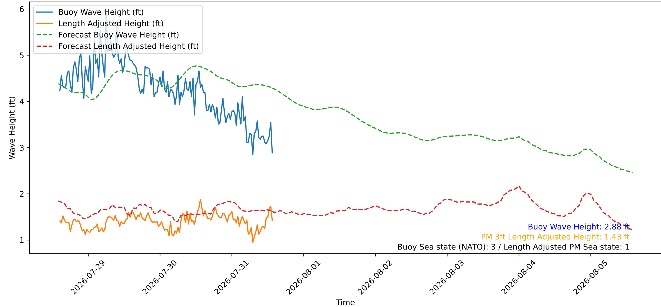
Wave Heights over Time for Oceanside Harbor at 2026-07-31 14:20:27
