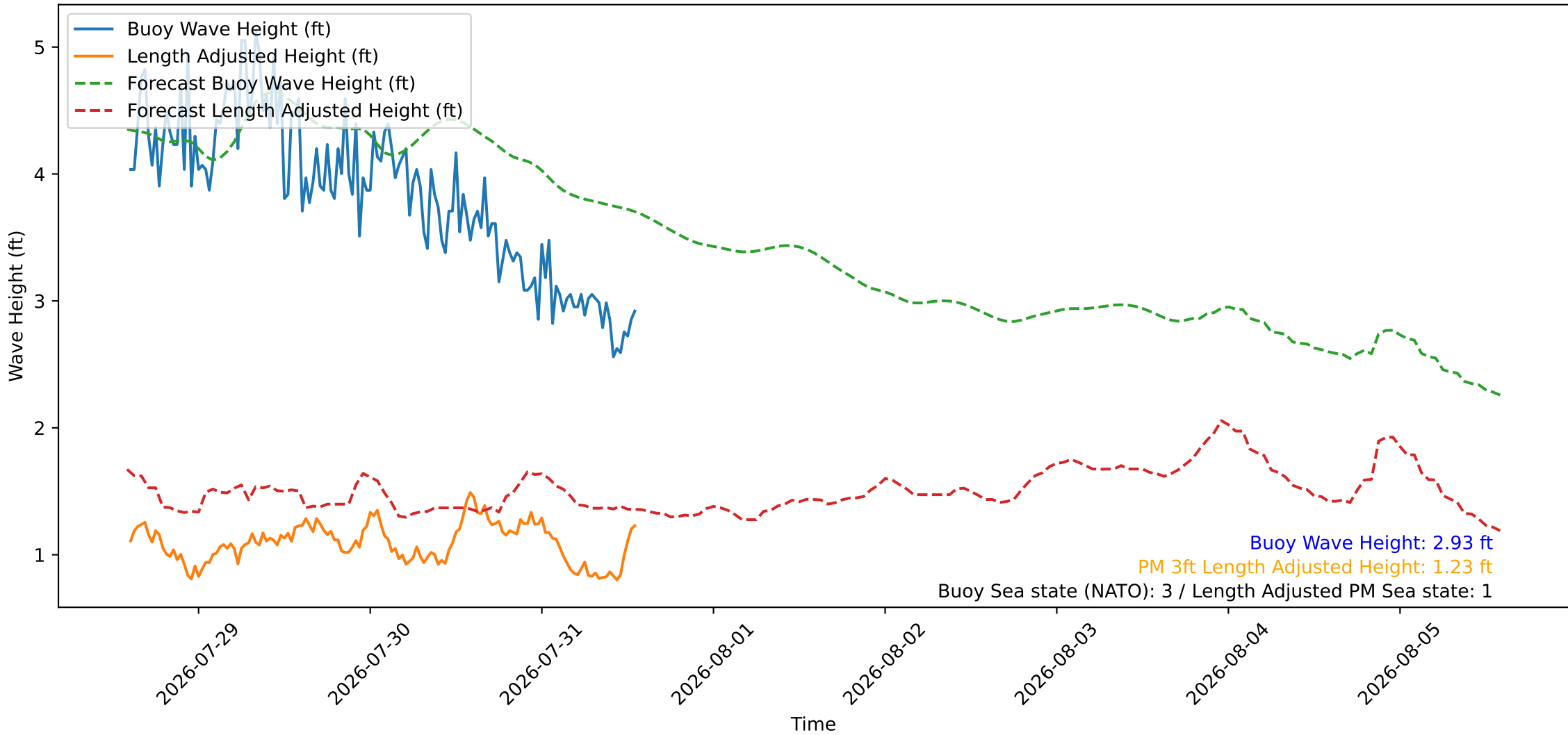
Wave Heights over Time for Red Beach at 2026-07-31 14:20:48
