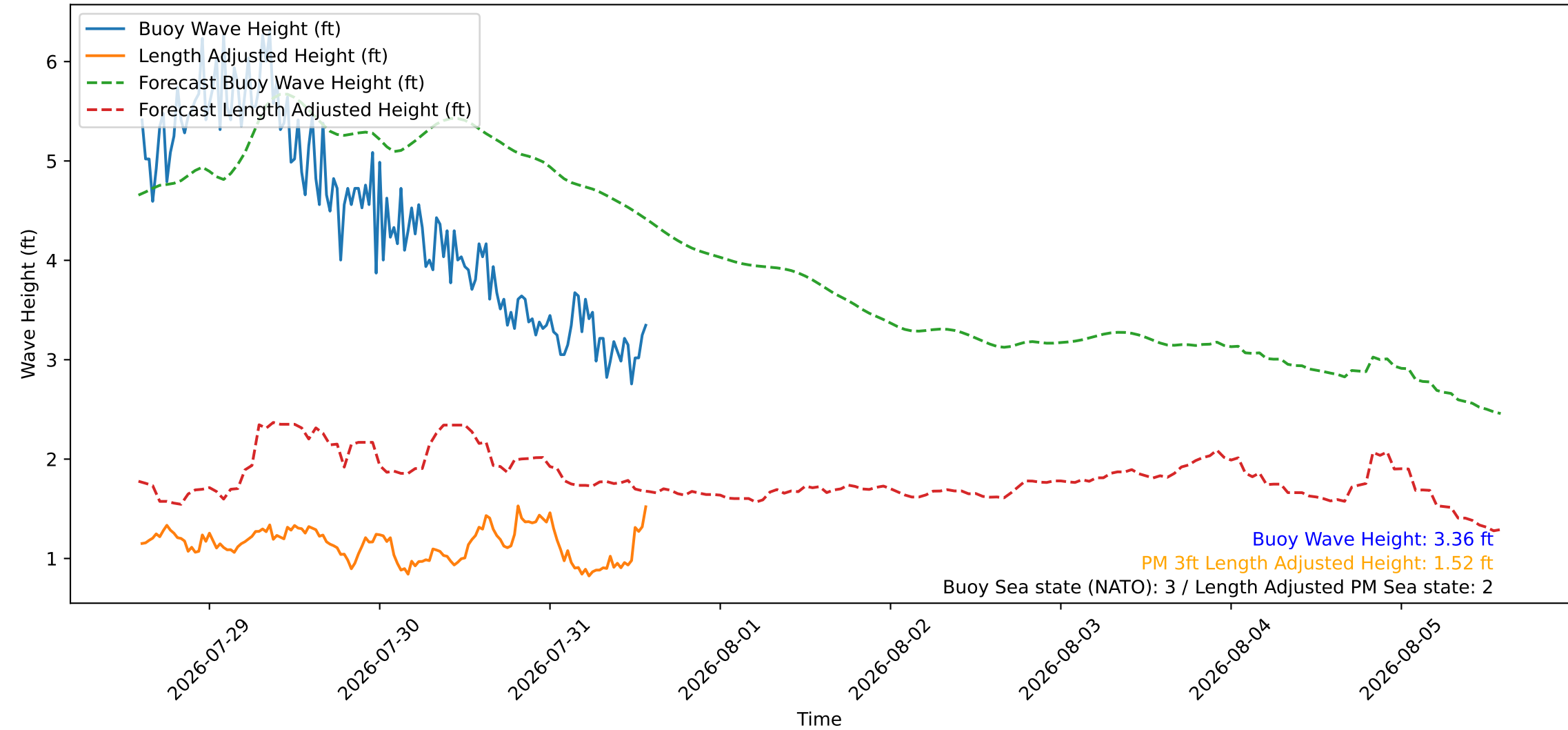
Wave Heights over Time for Green Beach at 2026-07-31 14:21:11
