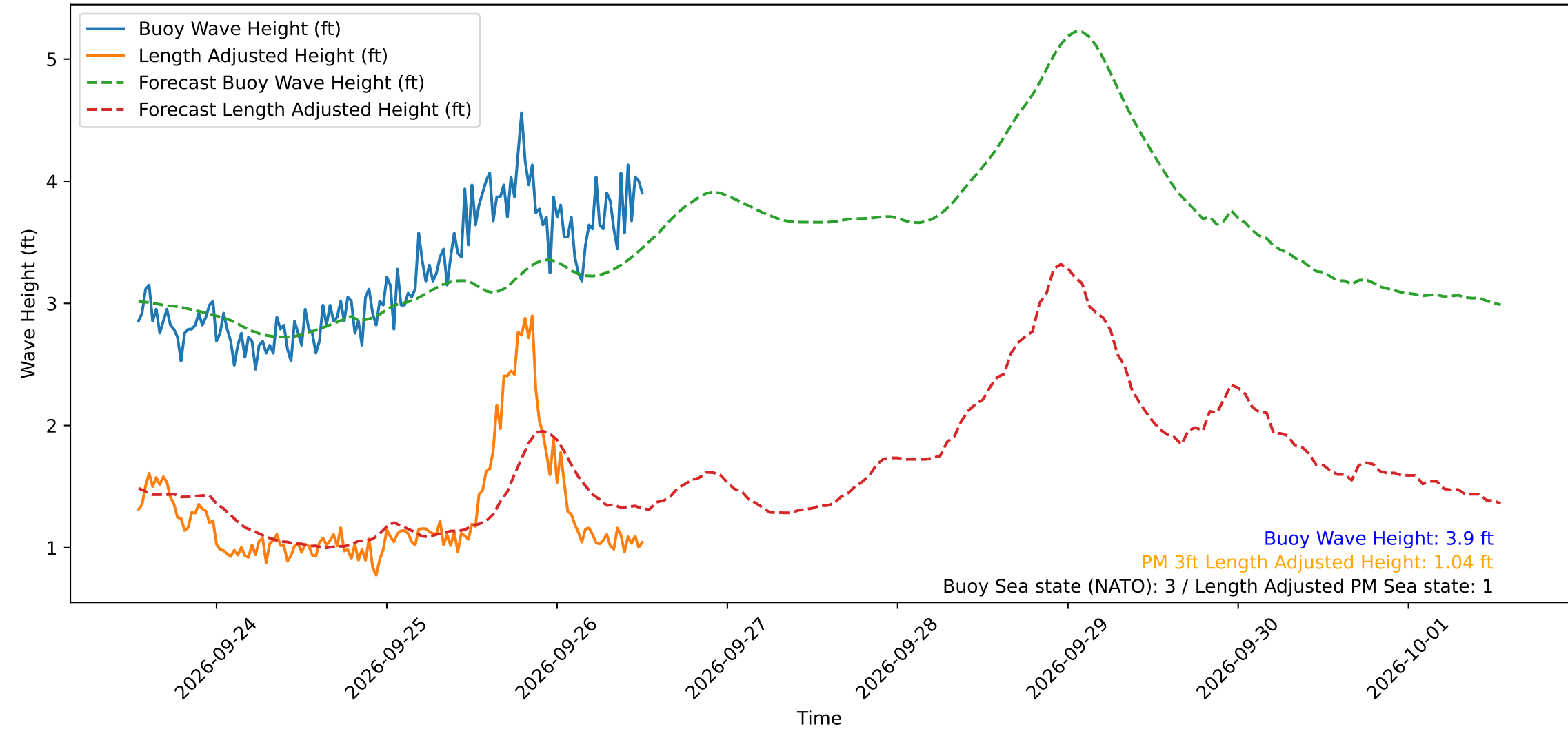
Wave Heights over Time for Green Beach at 2026-09-26 12:51:14
