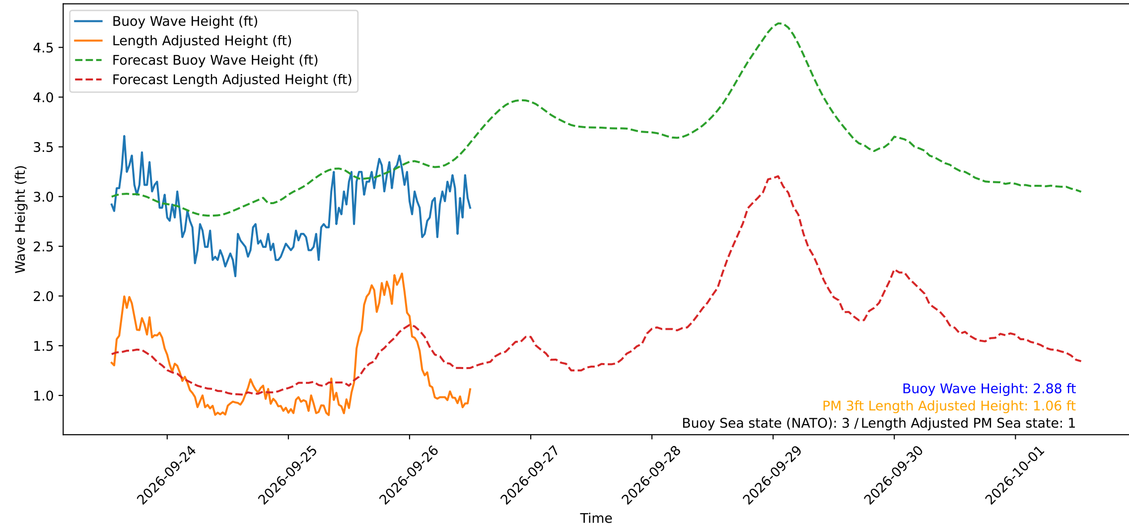
Wave Heights over Time for Oceanside Harbor at 2026-09-26 12:50:30
