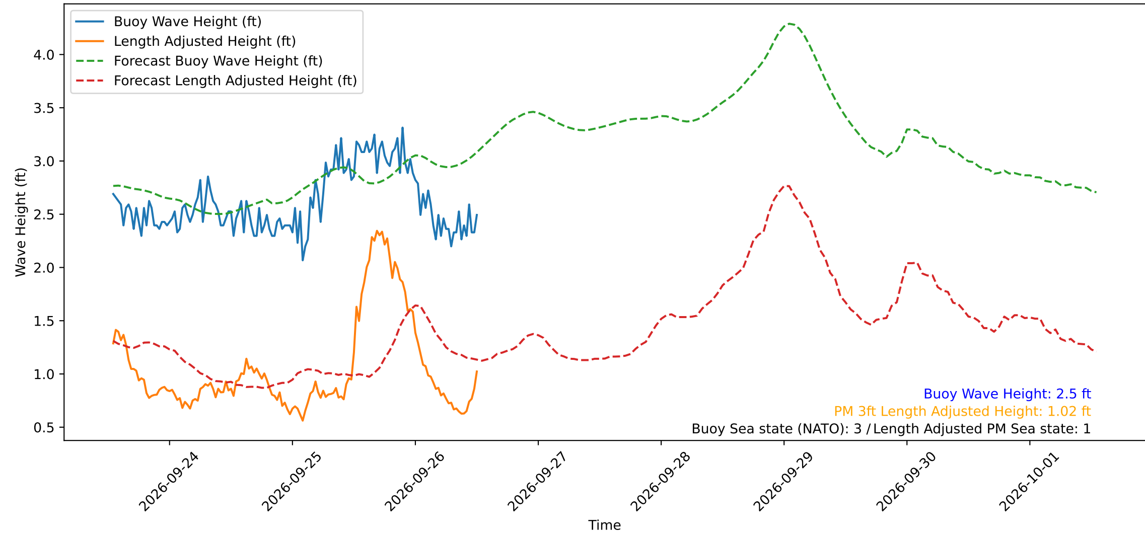
Wave Heights over Time for Red Beach at 2026-09-26 12:50:50
