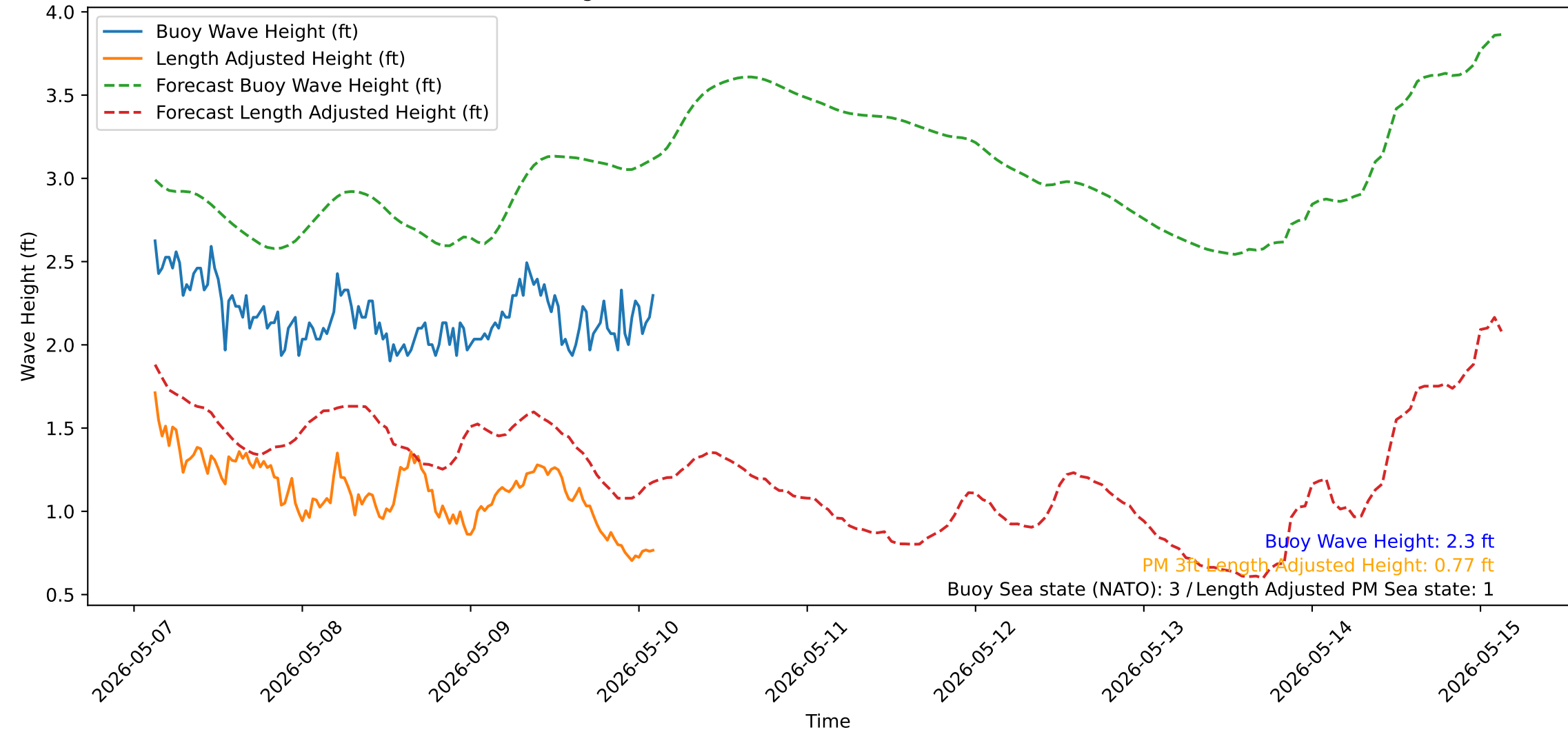
Wave Heights over Time for Red Beach at 2026-05-10 02:50:51
