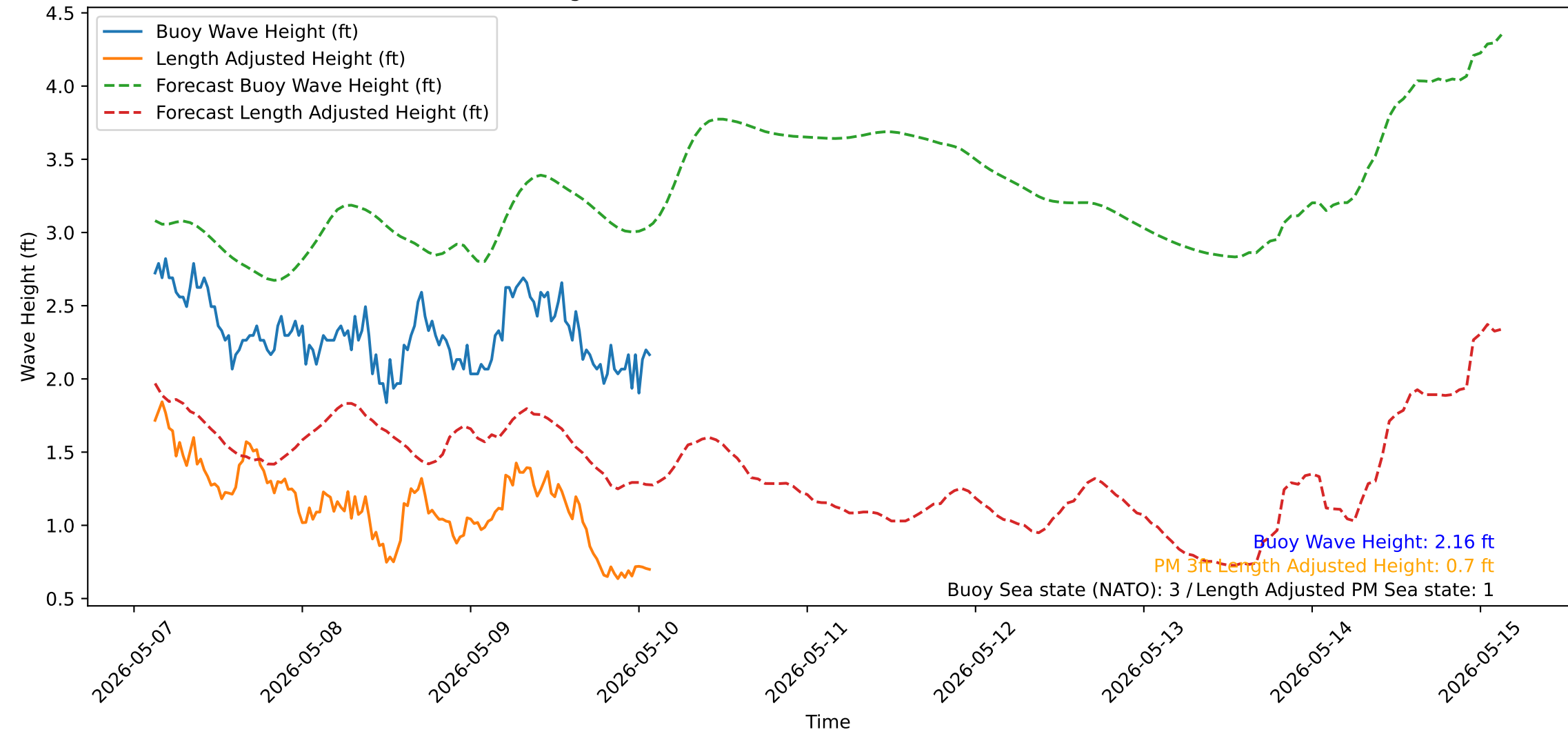
Wave Heights over Time for Green Beach at 2026-05-10 02:51:14
