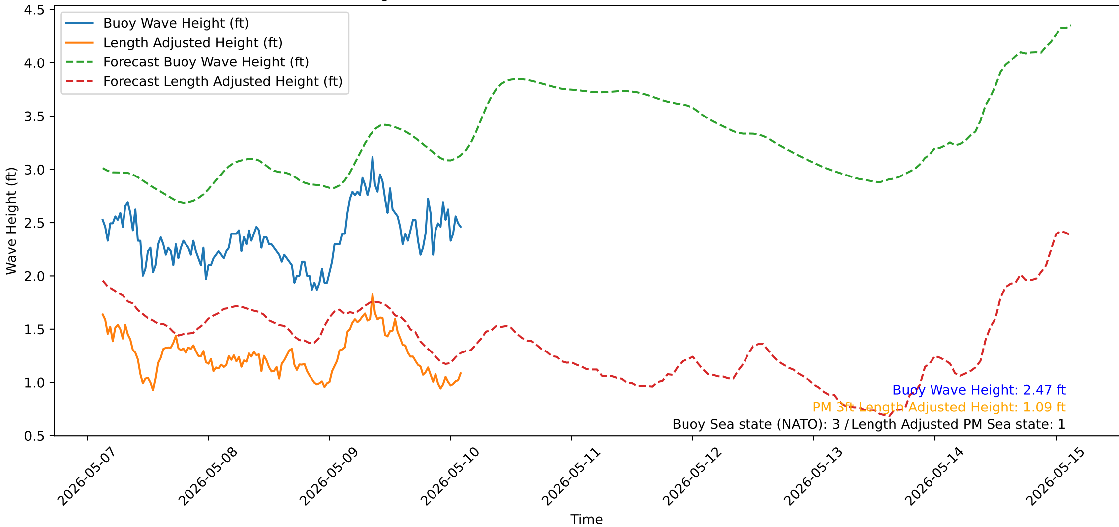
Wave Heights over Time for Oceanside Harbor at 2026-05-10 02:50:31
