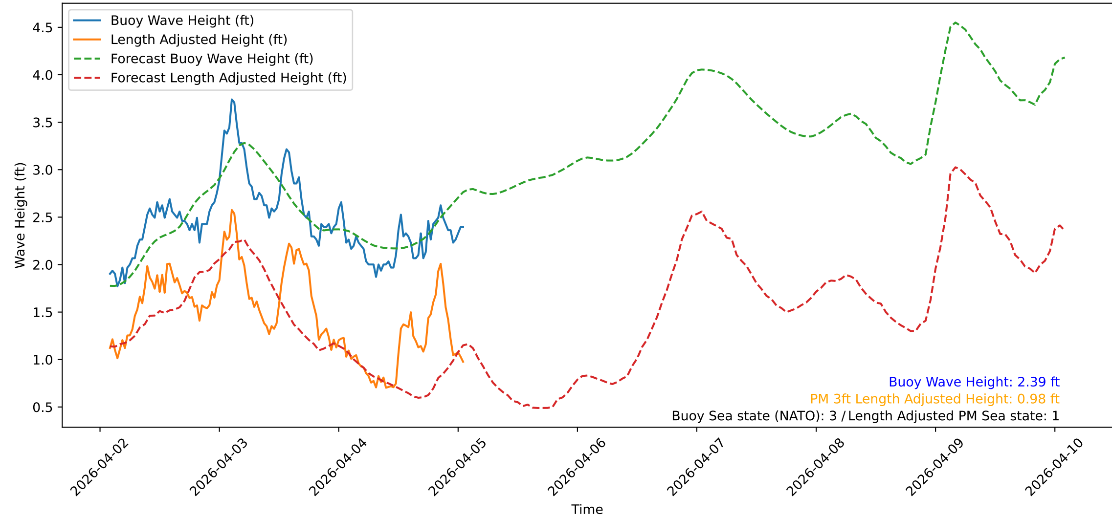
Wave Heights over Time for Red Beach at 2026-04-05 01:50:48
