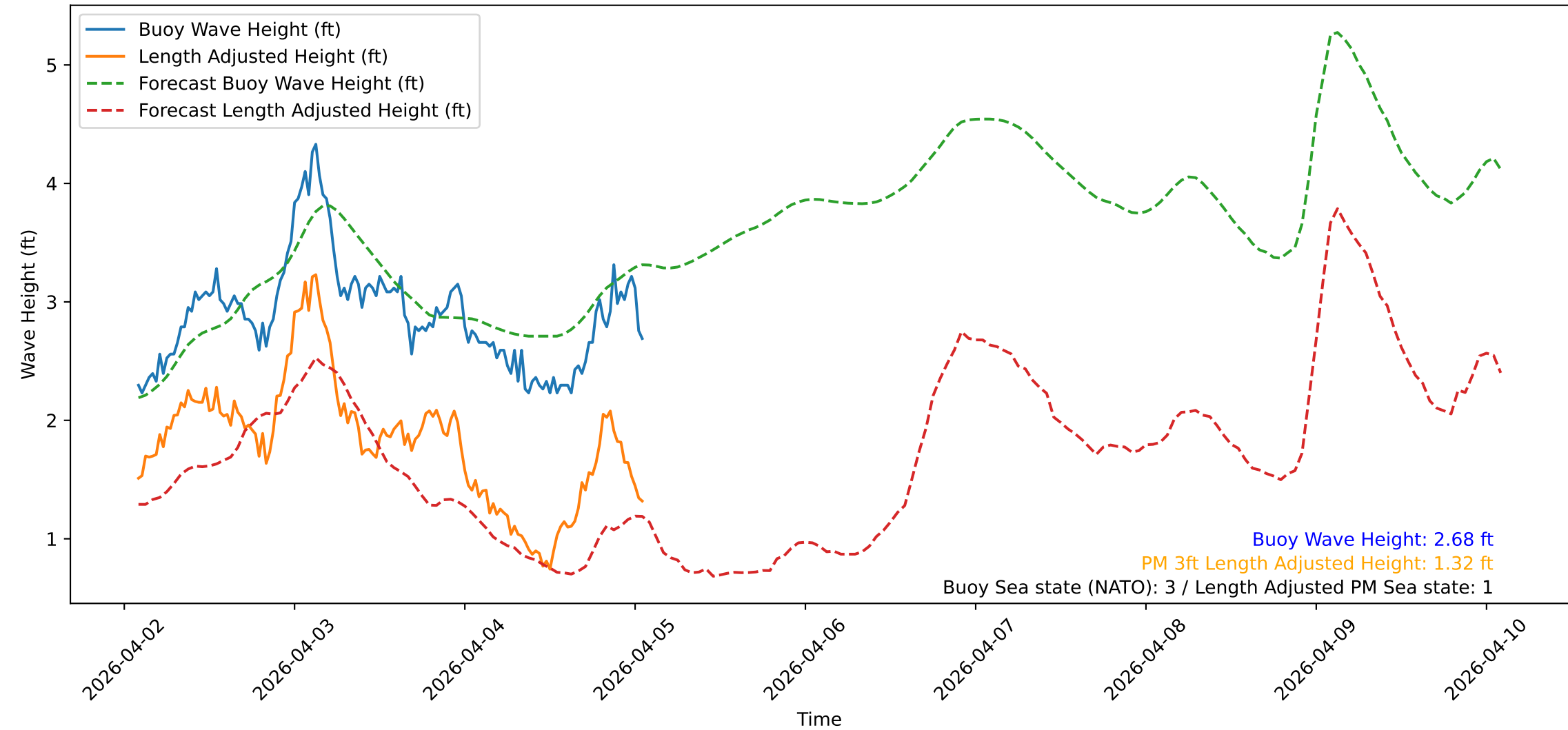
Wave Heights over Time for Green Beach at 2026-04-05 01:51:10
