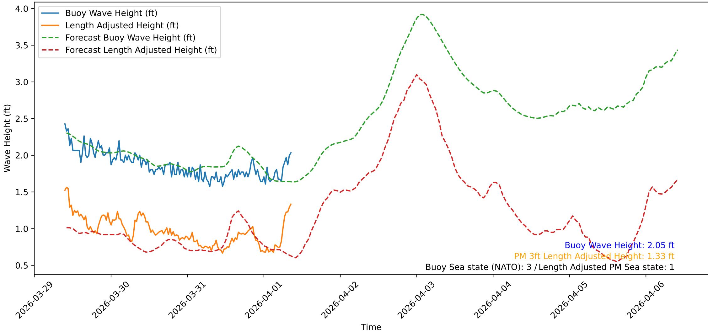
Wave Heights over Time for Oceanside Harbor at 2026-04-01 09:40:30
