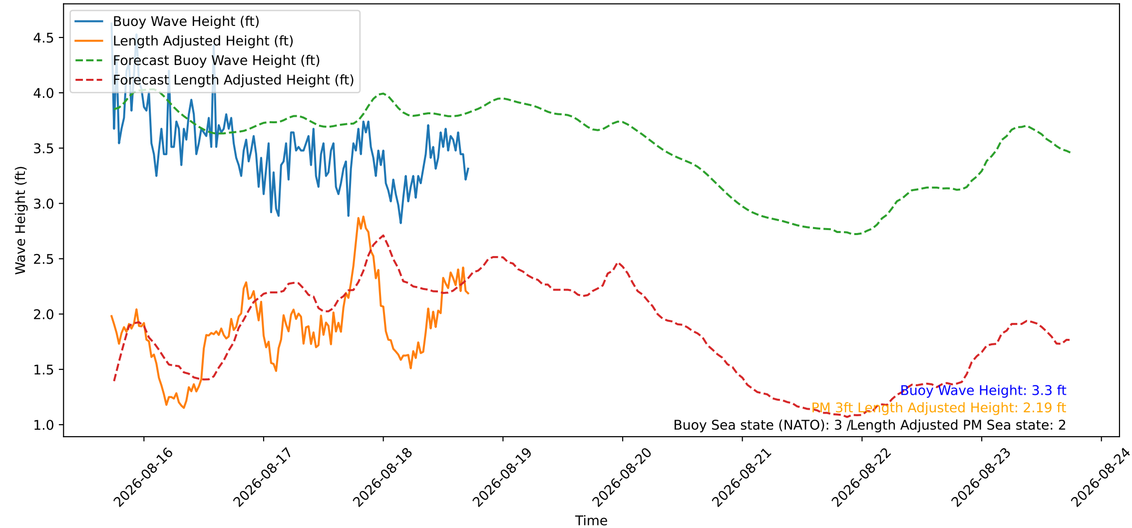
Wave Heights over Time for Oceanside Harbor at 2026-08-18 17:40:26
