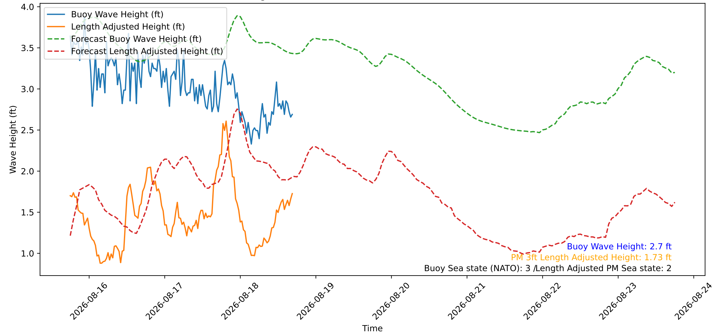
Wave Heights over Time for Red Beach at 2026-08-18 17:40:47
