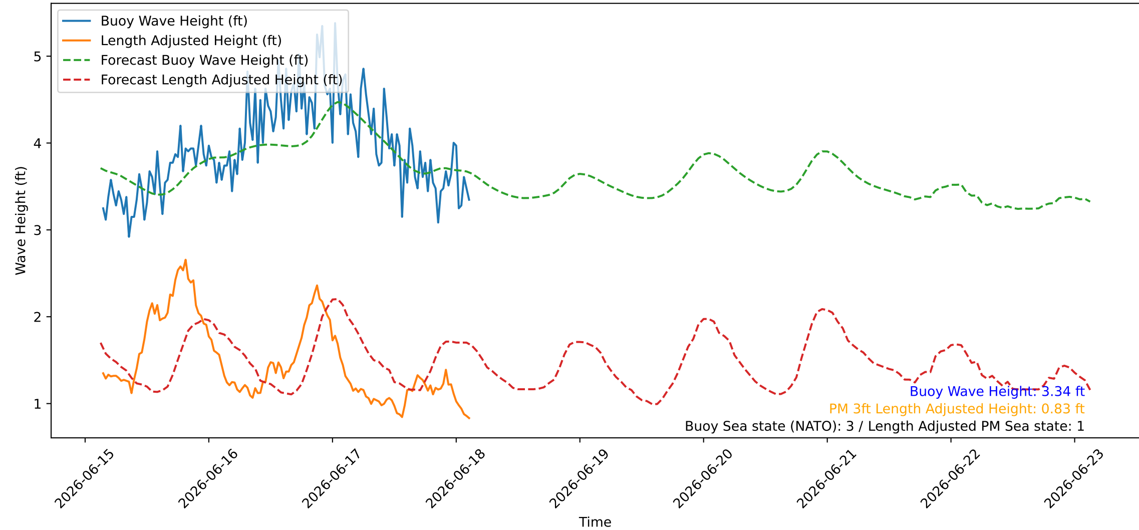
Wave Heights over Time for Red Beach at 2026-06-18 03:10:45
