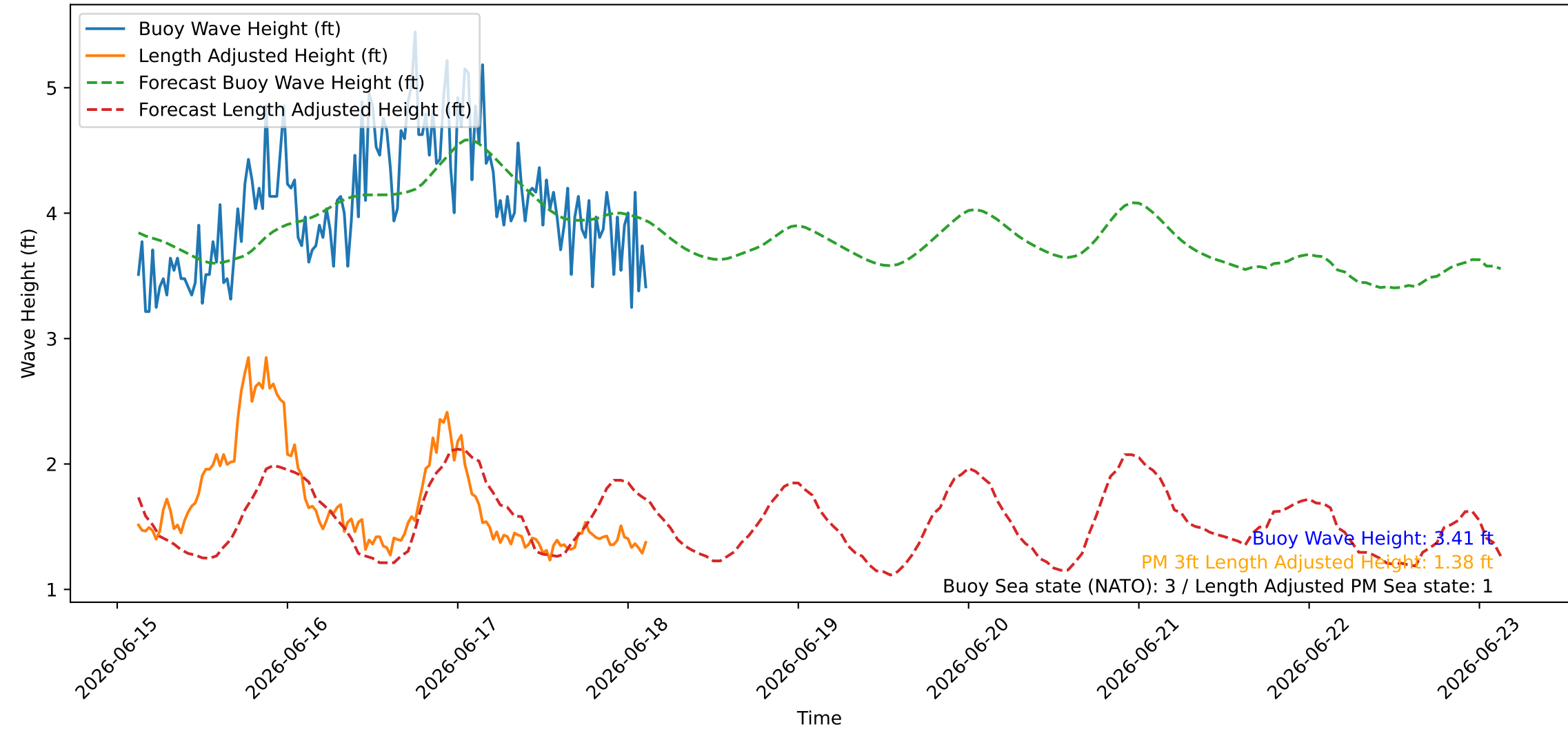
Wave Heights over Time for Oceanside Harbor at 2026-06-18 03:10:26
