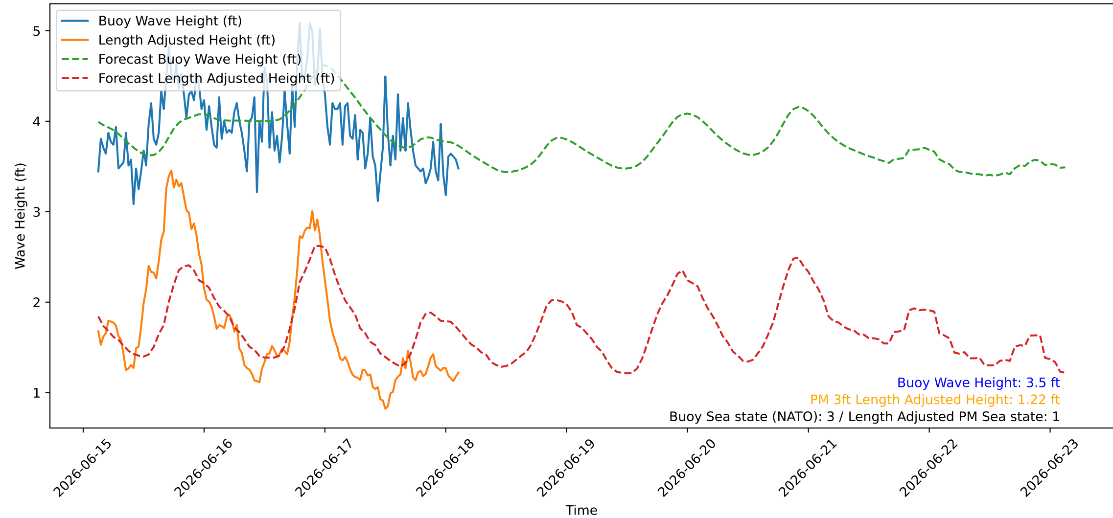
Wave Heights over Time for Green Beach at 2026-06-18 03:11:07
