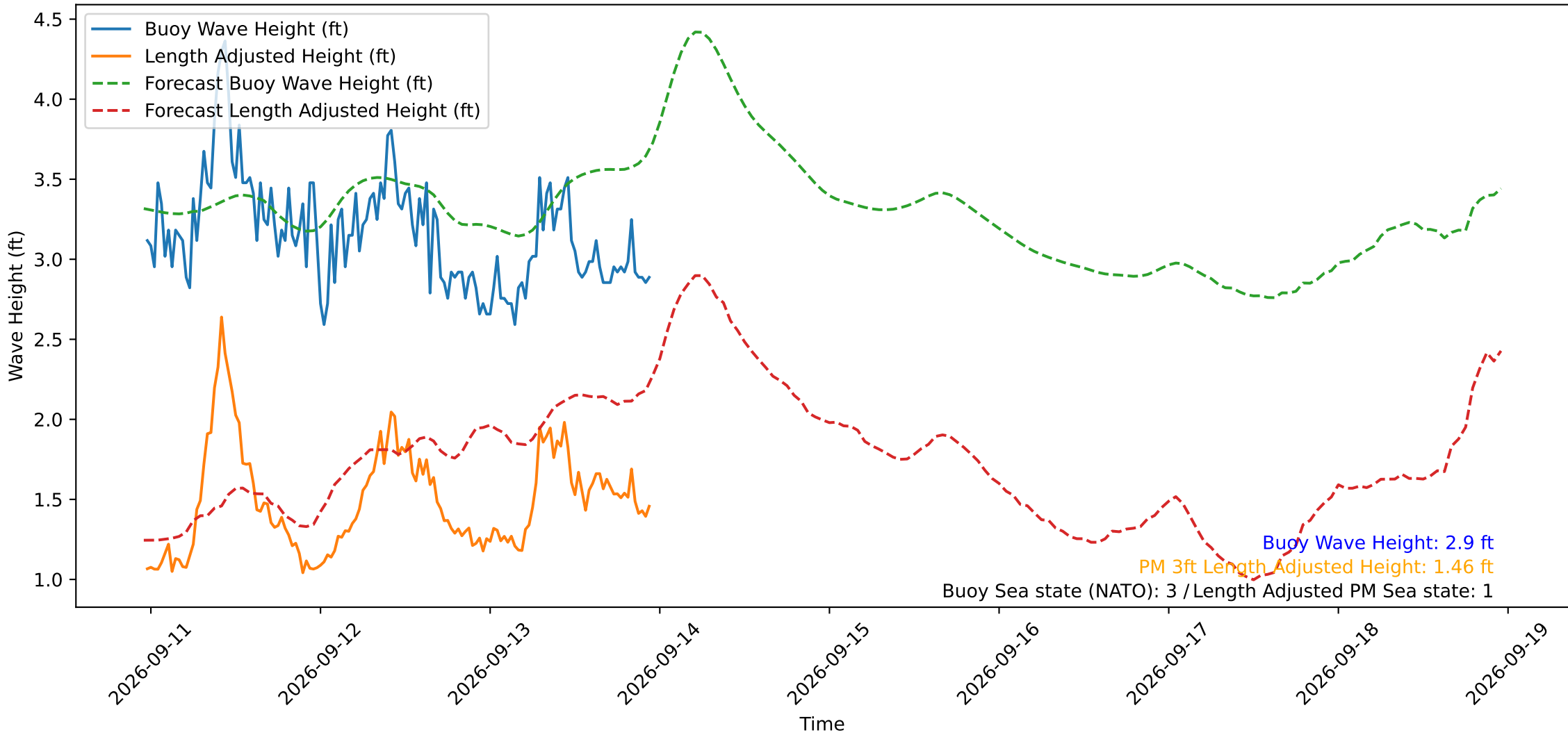
Wave Heights over Time for Oceanside Harbor at 2026-09-13 23:20:29
