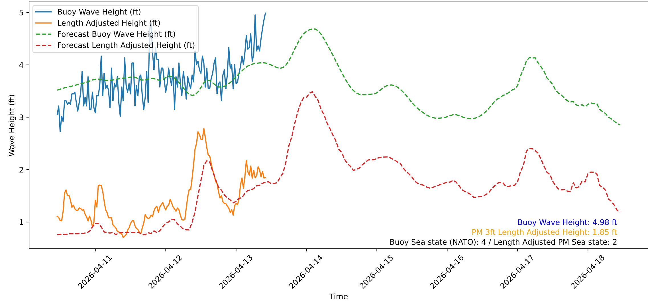
Wave Heights over Time for Oceanside Harbor at 2026-04-13 10:50:31
