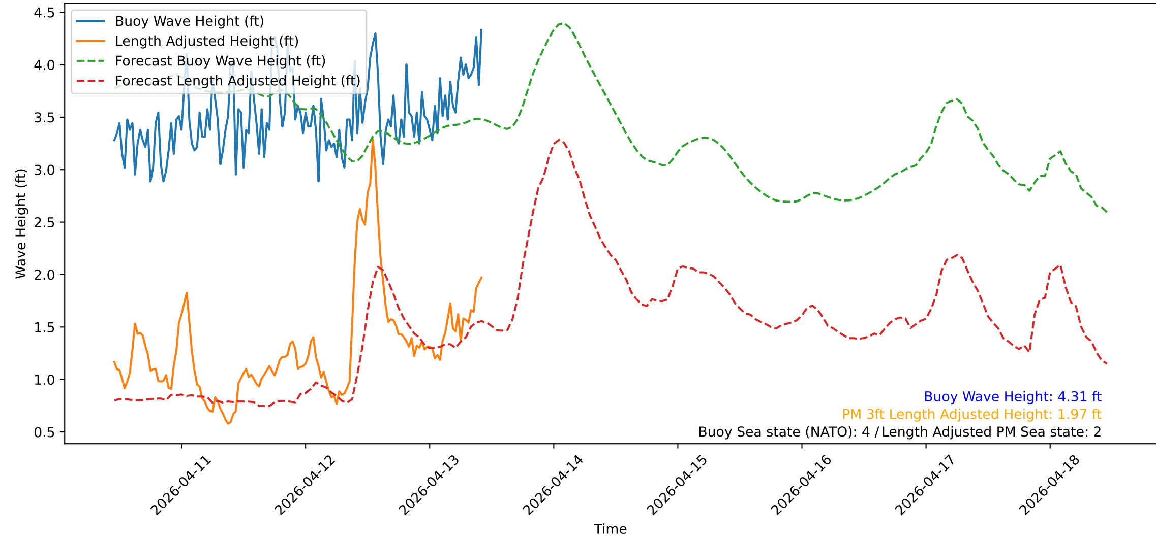
Wave Heights over Time for Red Beach at 2026-04-13 10:50:52
