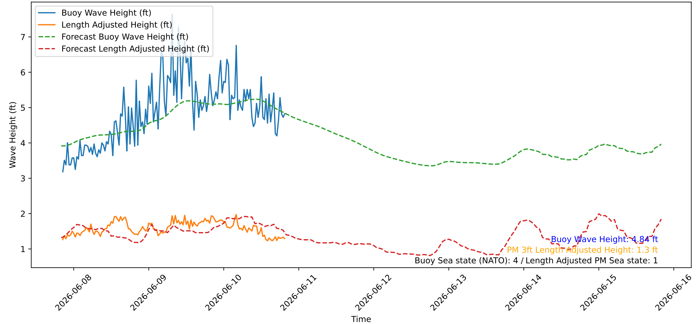
Wave Heights over Time for Red Beach at 2026-06-10 20:10:47
