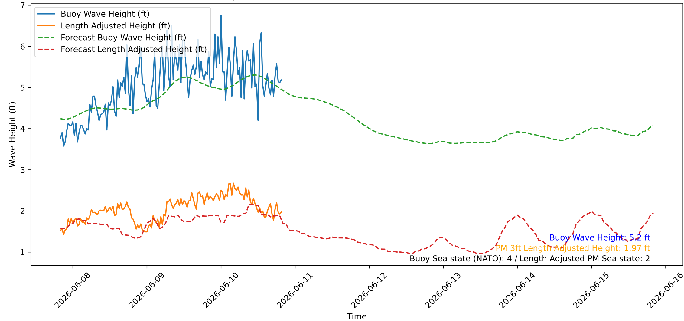
Wave Heights over Time for Oceanside Harbor at 2026-06-10 20:10:26
