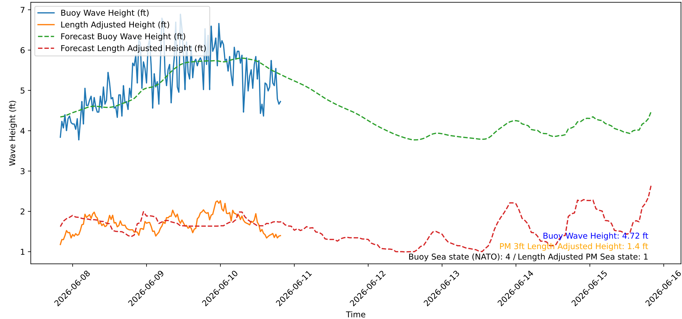
Wave Heights over Time for Green Beach at 2026-06-10 20:11:10
