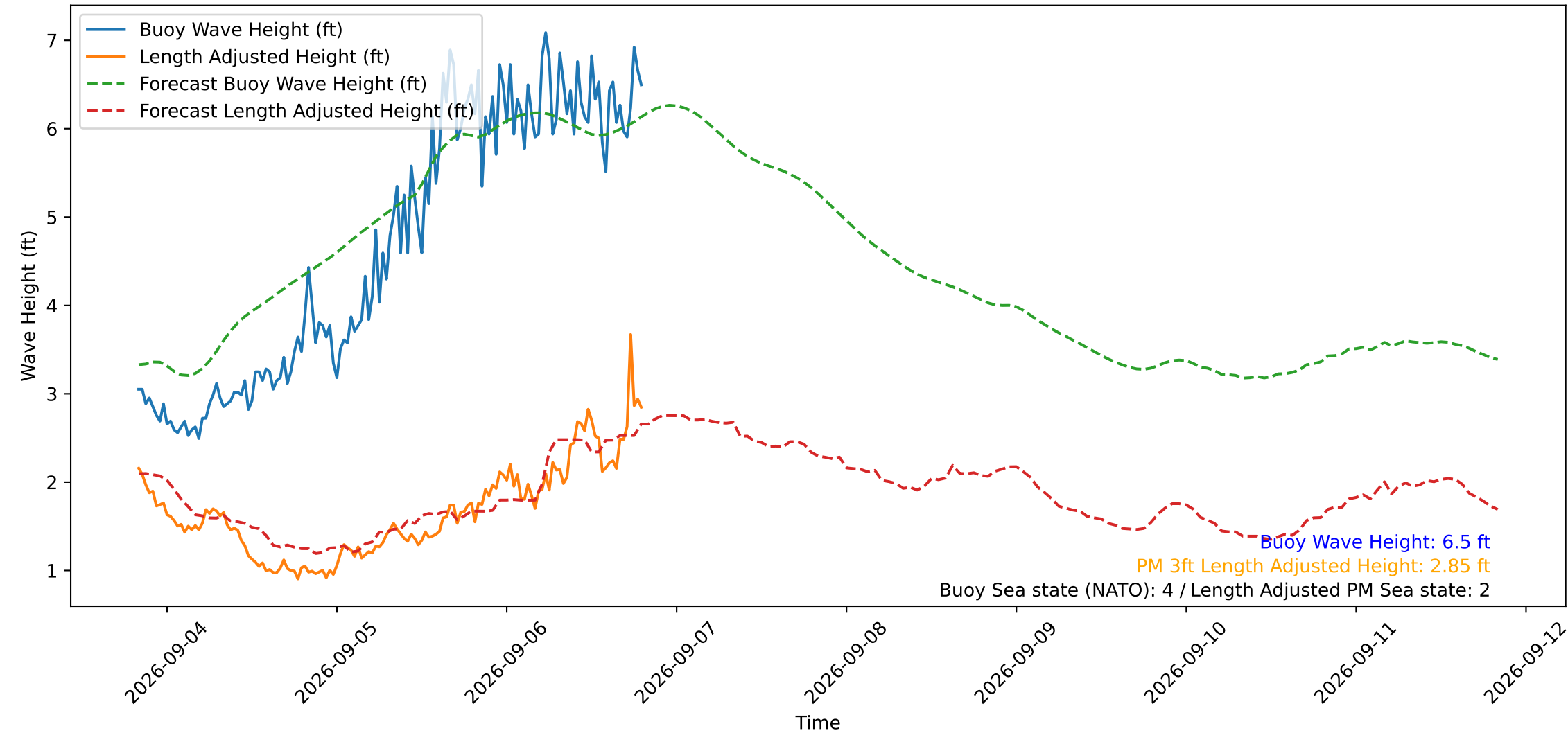
Wave Heights over Time for Green Beach at 2026-09-06 19:51:15
