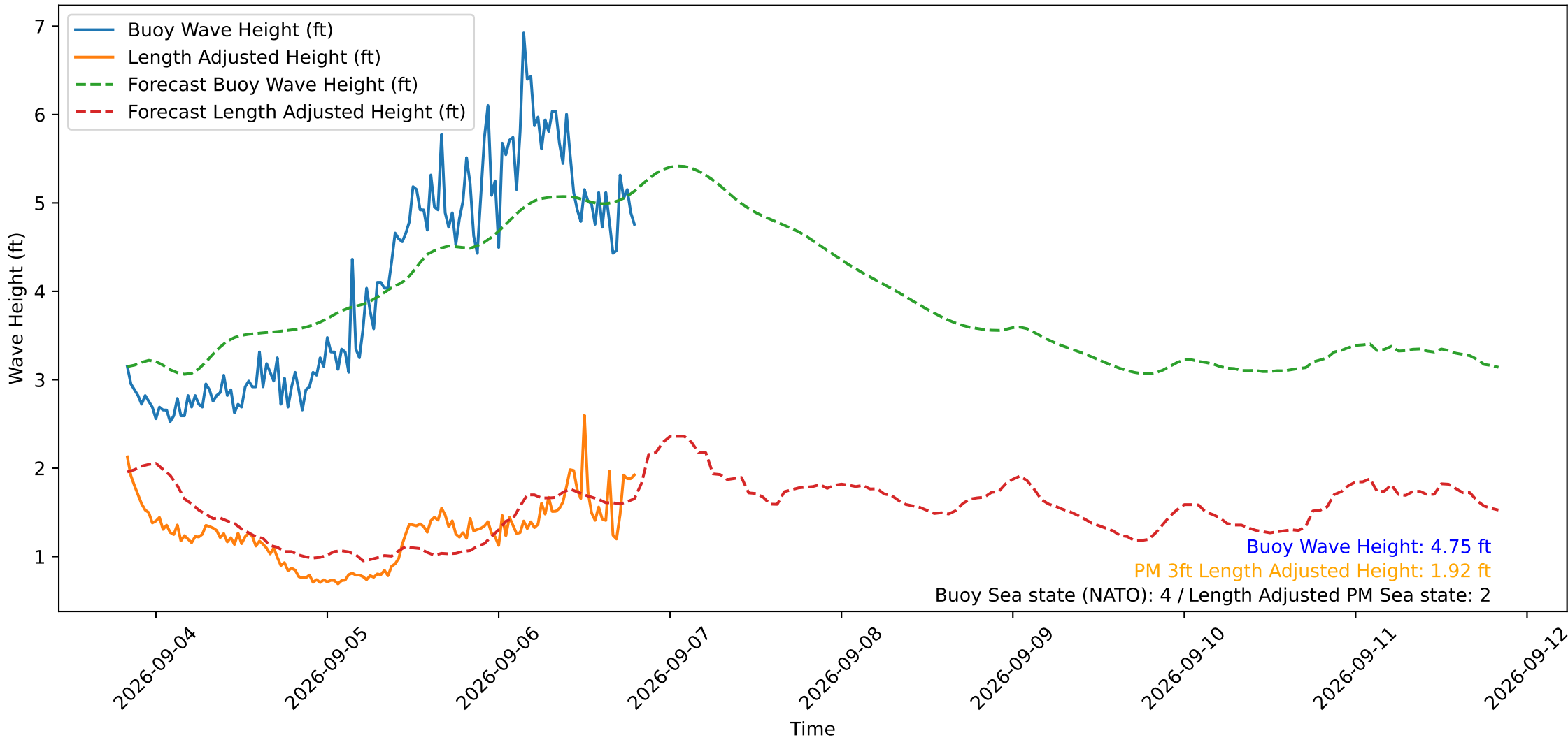
Wave Heights over Time for Red Beach at 2026-09-06 19:50:50
