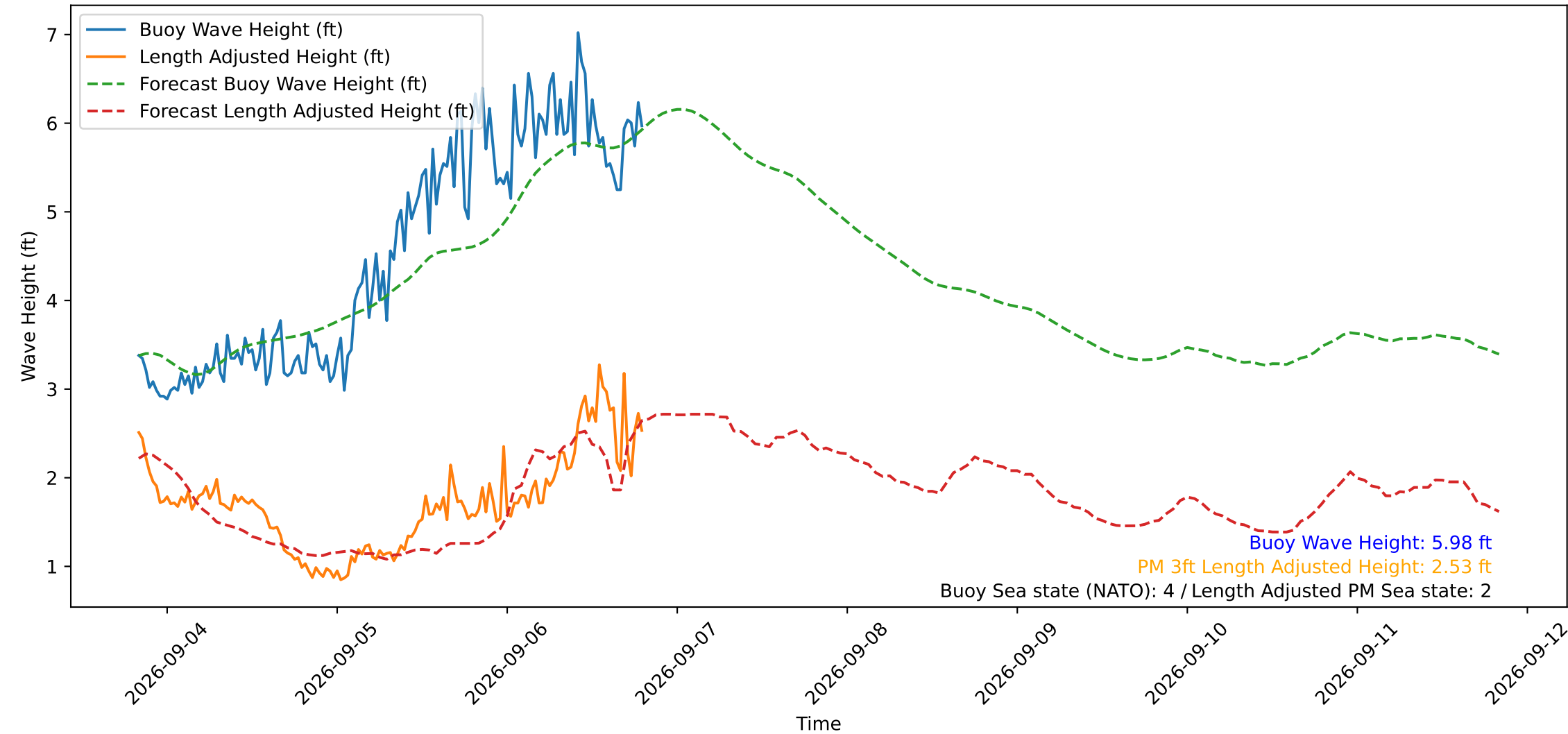
Wave Heights over Time for Oceanside Harbor at 2026-09-06 19:50:29
