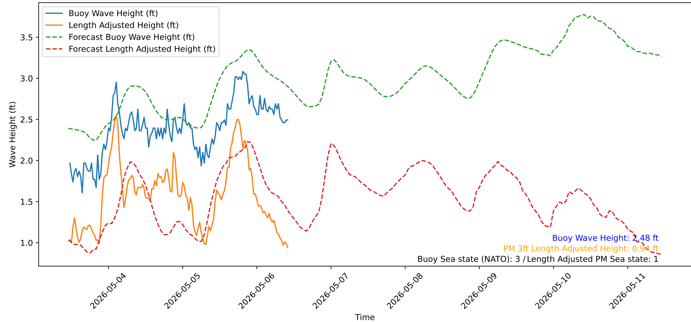
Wave Heights over Time for Red Beach at 2026-05-06 11:20:52
