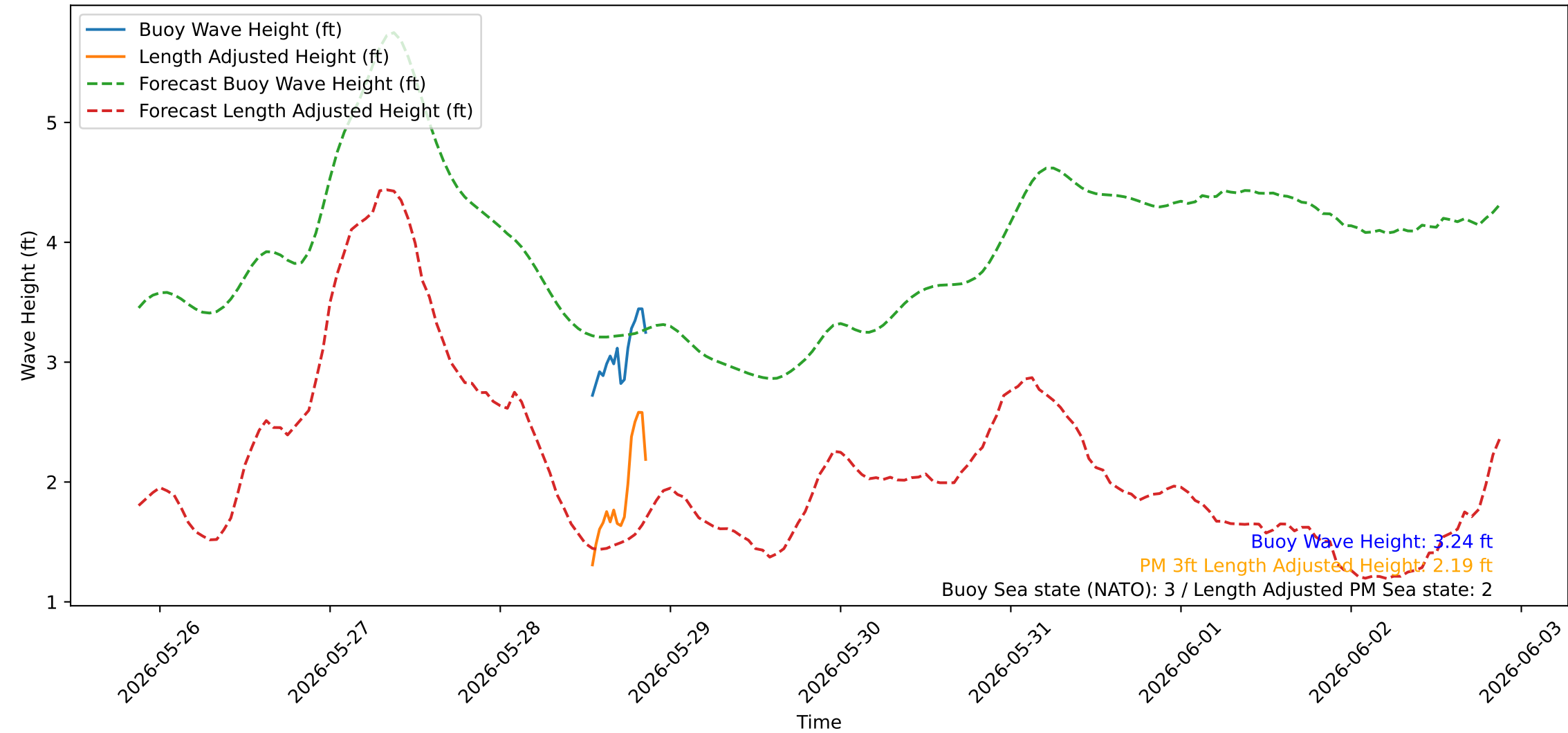
Wave Heights over Time for Oceanside Harbor at 2026-05-28 21:10:20
